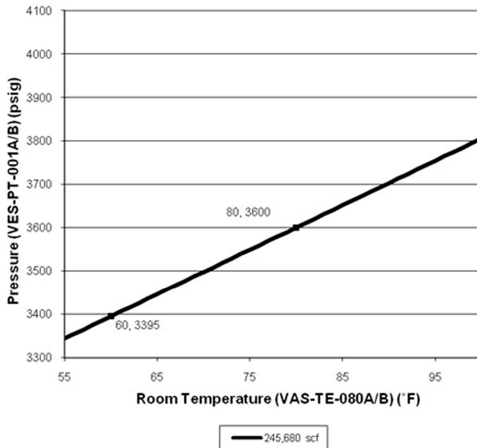
Figure B 3.7.6-2 Compressed Air Storage Tanks Minimum Volume – One Bank of VES Air Tanks (8 Tanks) Inoperable
