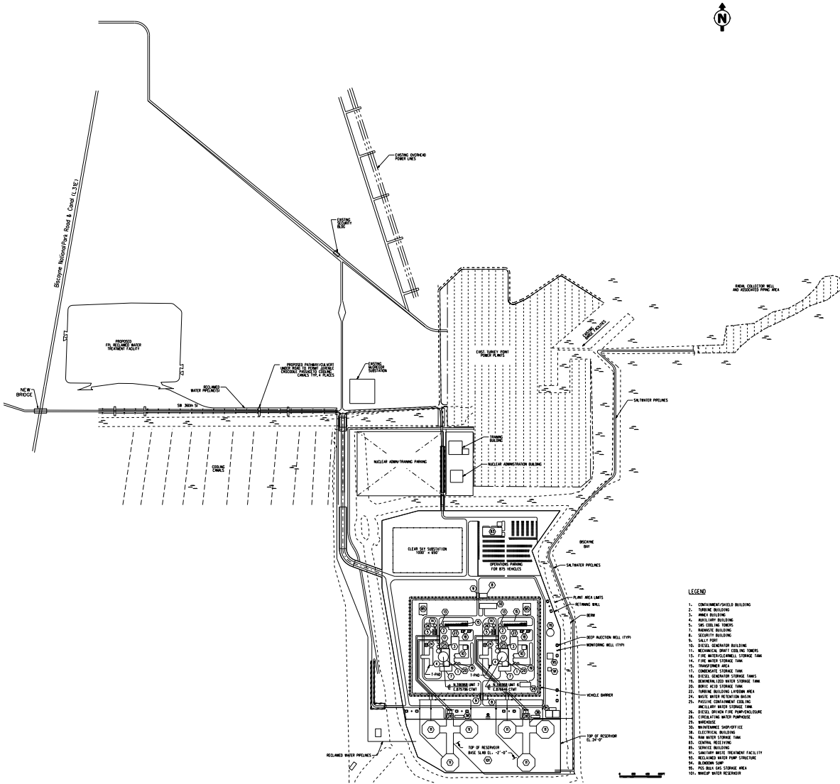
Figure 3.1-3 Plot Plan Showing Major Structures
