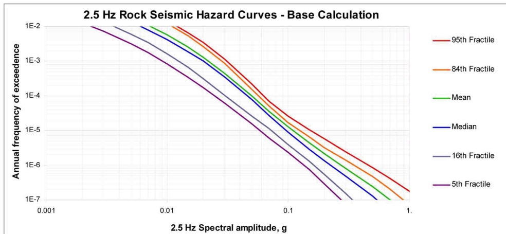
Figure 2.5.2-222 Mean and Fractile Rock 2.5 Hz Seismic Hazard Curves, Rock
