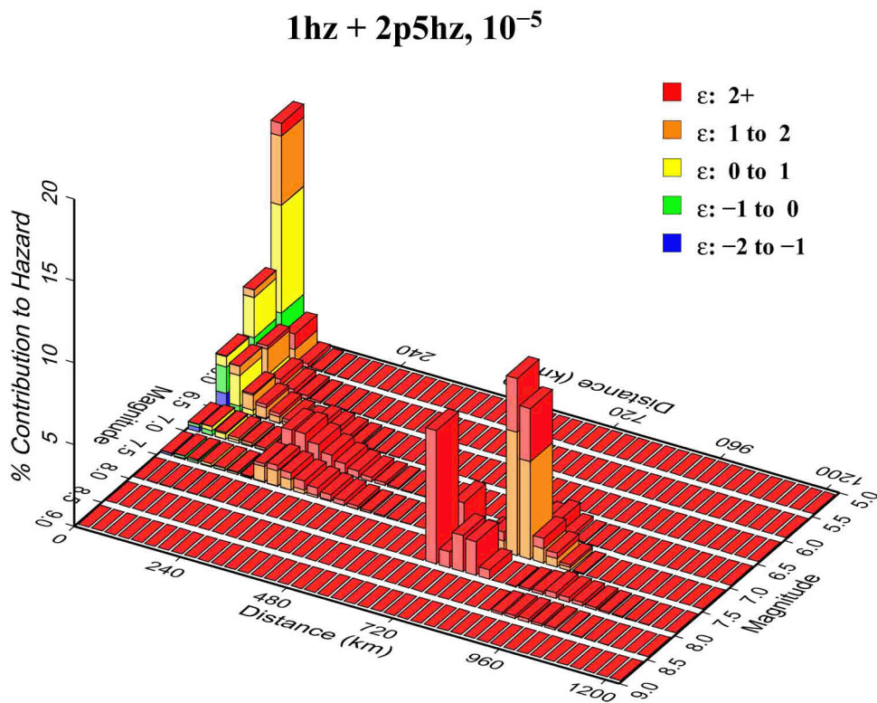
Figure 2.5.2-228 M and R Deaggregation for 1 and 2.5 Hz at 1E-05 Annual Frequency of Exceedence
