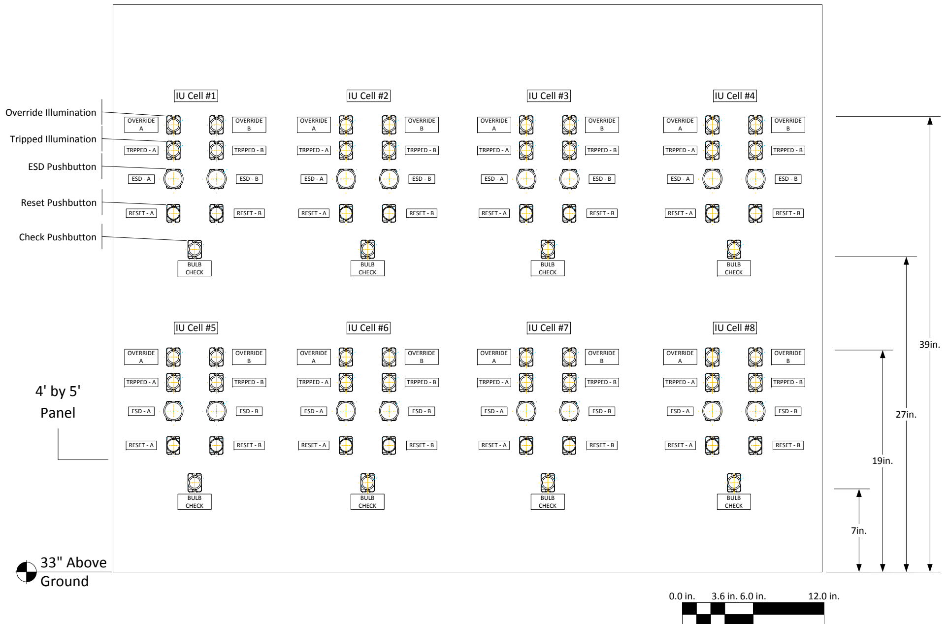
Figure 7a2.5-3 – ESFAS Manual Operator Panel
