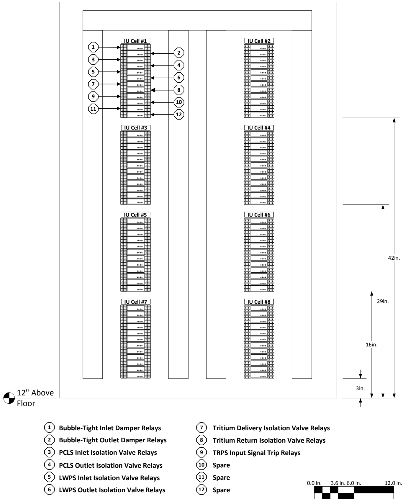
Figure 7a2.5-2 – Example ESFAS Panel
