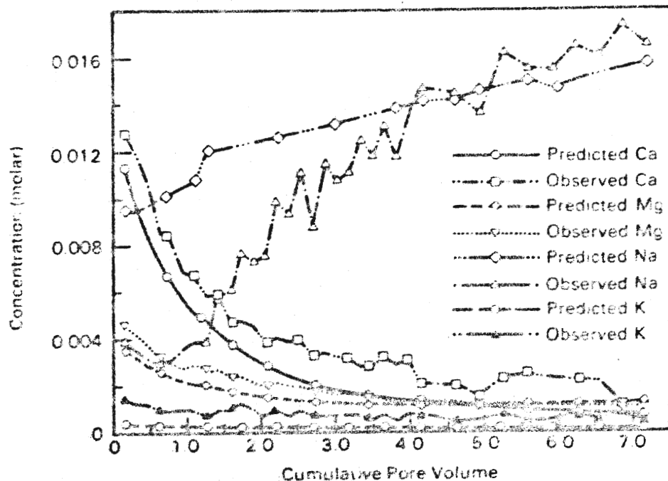
FIGURE 26. Comparison of Predicted Major Cation Effluent Compositions with Analytical Values for the Wyoming Natural Restoration Column Experiment
