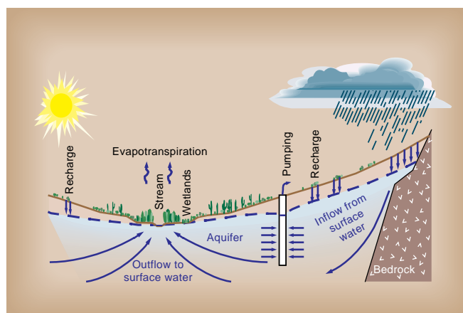
Figure 5. Availability of an adequate supply of freshwater is a significant issue affecting continued economic growth of cities and towns in the Southwest, which also contains some of the most productive agricultural lands in the United States. Environmental considerations create increasing constraints on water development. For example, perennial streams, springs, and wetlands depend on ground-water discharge for their existence. In addition, the effects of climatic variability on water resources, particularly on ground-water recharge, are not well understood and are a major deficiency in current models used in water management.
