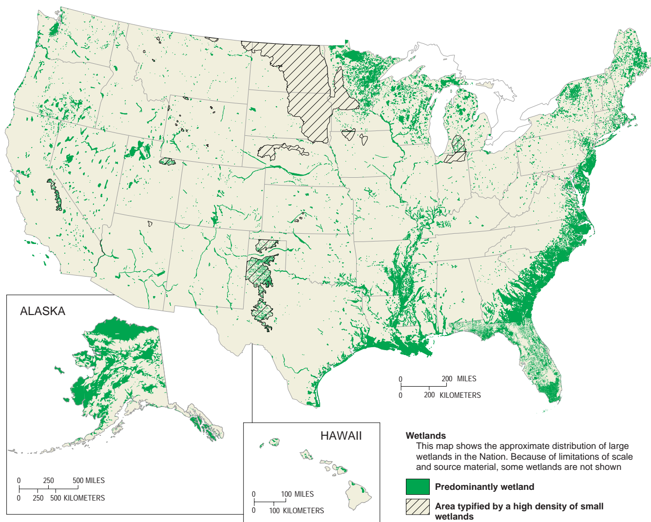
Figure 8. Understanding wetland hydrology will be improved if the relationships between ground water and wetlands are more clearly established. Wetlands occur throughout the United States and cover large areas in the north-central and north-eastern United States, coastal areas along the Atlantic and Gulf coasts, riverine terrane in the lower Mississippi River valley, and Alaska. (Modified from U.S. Geological Survey Water-Supply Paper 2425.)
