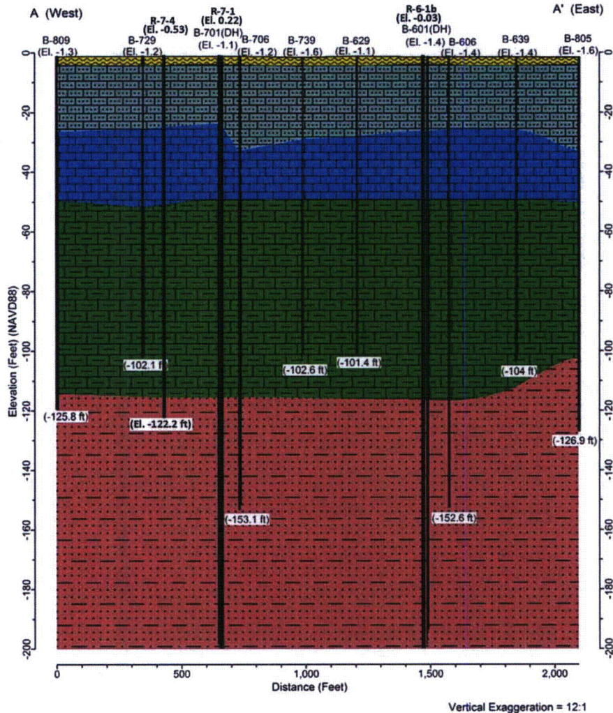
Figure 2.5AA-211 Cross-Section A-A' Truncated (Vertical Exaggeration = 12:1) This figure appears in FSAR Subsection 2.5.1 as Figure 2.5.1-338
