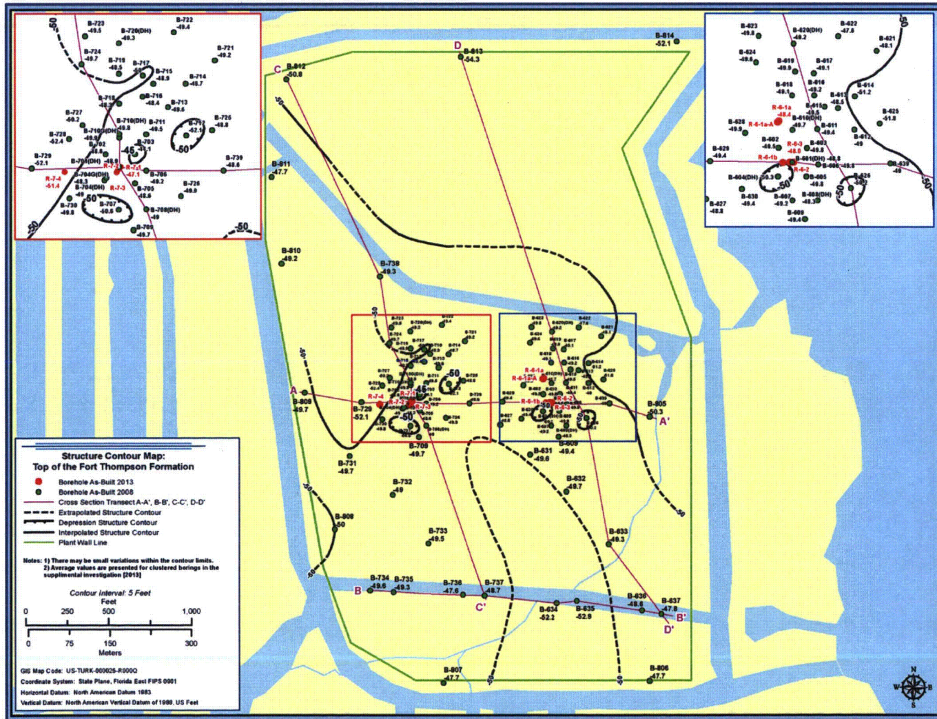
Figure 2.5AA-208 Structure Contour Map of the Top of the Fort Thompson Formation This figure appears in FSAR Subsection 2.5.1 as Figure 2.5.1-343
