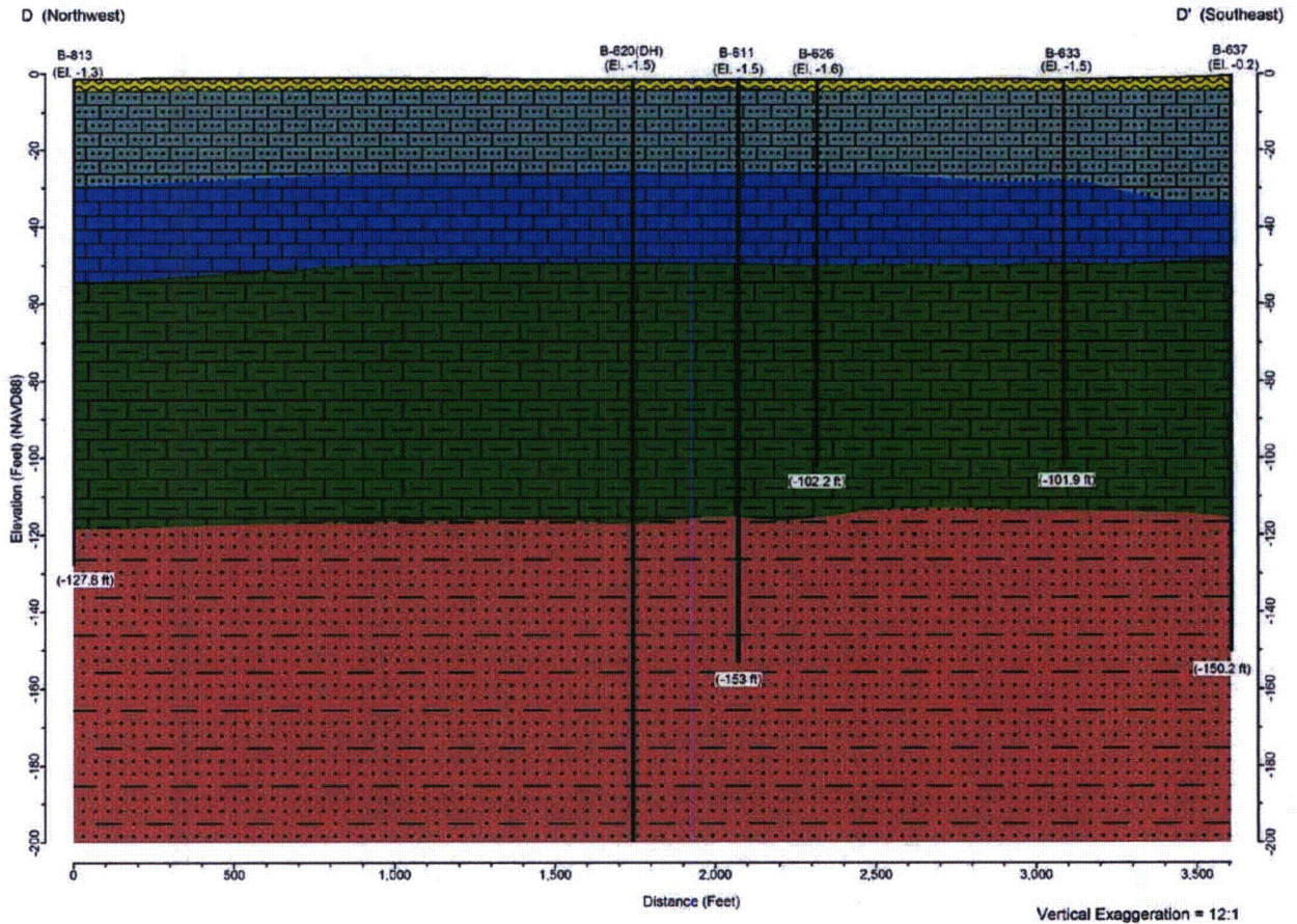
Figure 2.5AA-214 Cross-Section D-D' Truncated (Vertical Exaggeration = 12:1) This figure appears in FSAR Subsection 2.5.1 as Figure 2.5.1-341
