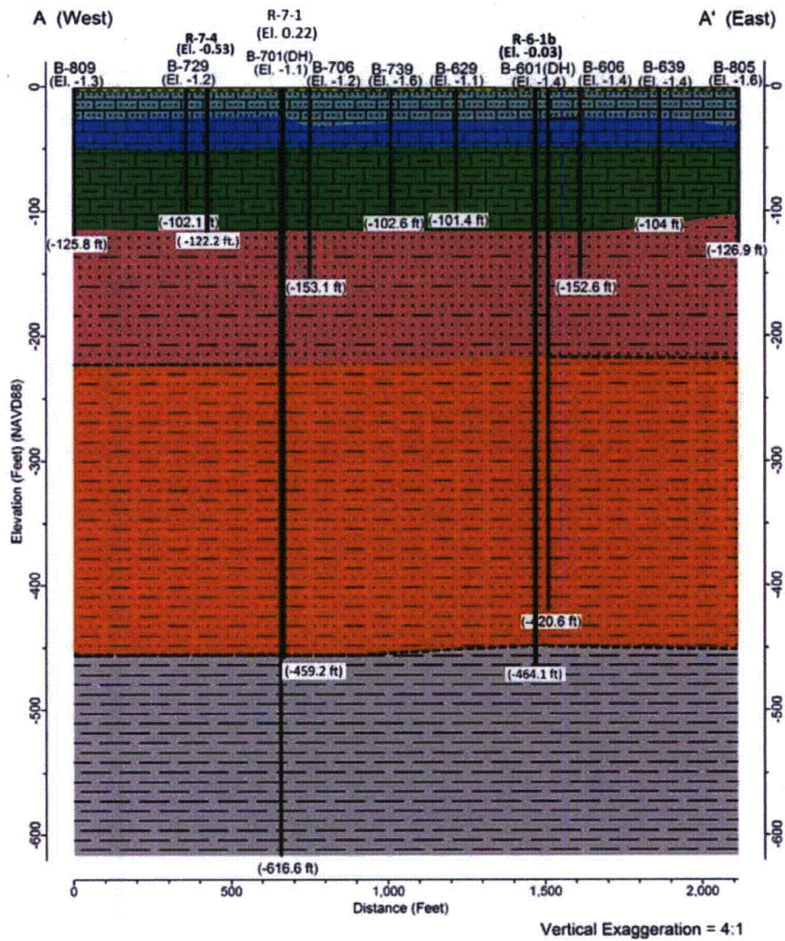
Figure 2.5AA-215 Cross-Section A-A' (Vertical Exaggeration = 4:1) This figure appears in FSAR Subsection 2.5.1 as Figure 2.5.1-386
