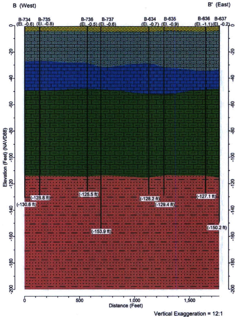
Figure 2.5AA-212 Cross-Section B-B' Truncated (Vertical Exaggeration = 12:1) This figure appears in FSAR Subsection 2.5.1 as Figure 2.5.1-339
