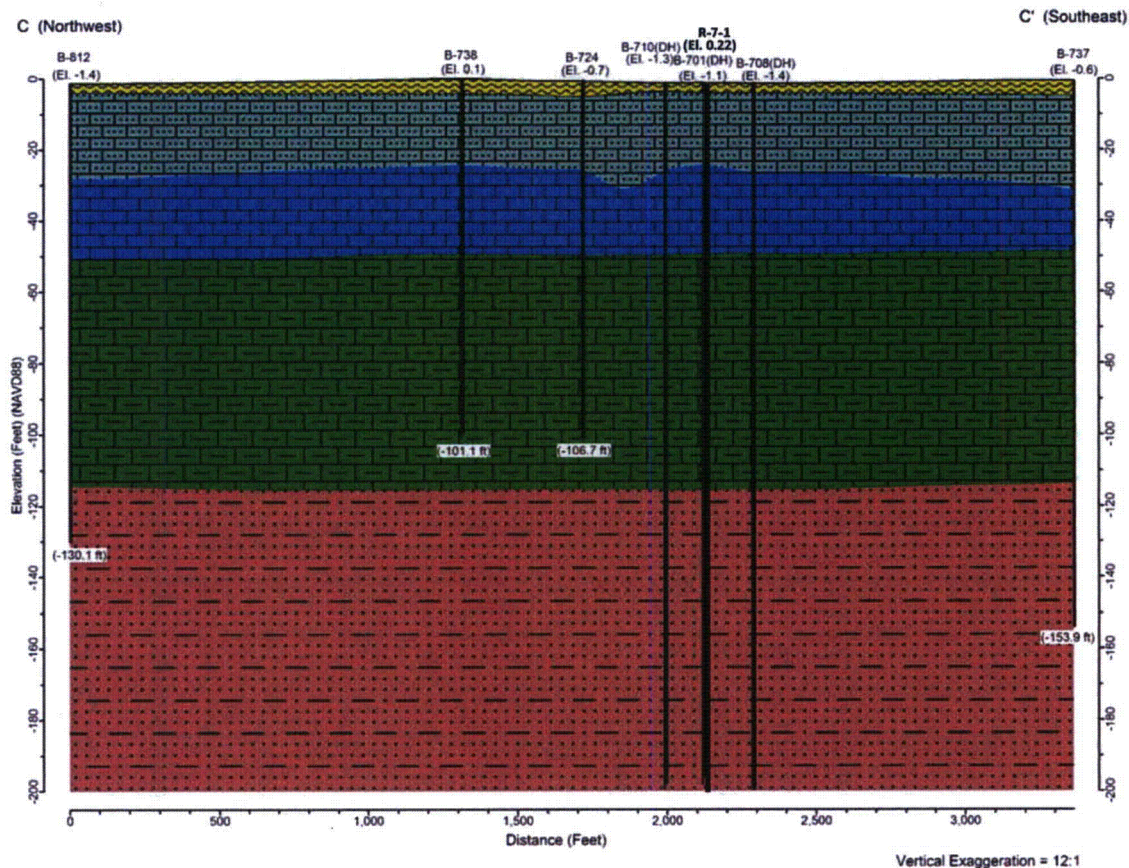
Figure 2.5AA-213 Cross-Section C-C' Truncated (Vertical Exaggeration = 12:1) This figure appears in FSAR Subsection 2.5.1 as Figure 2.5.1-340
