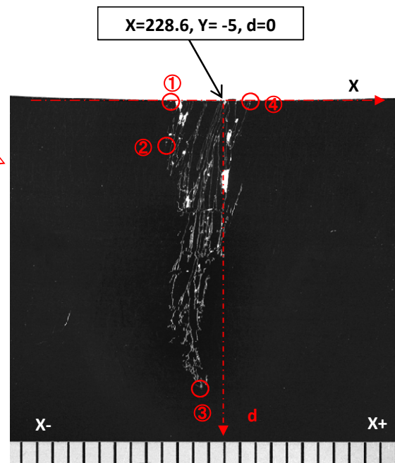
Position of cross section for observation (Y= - 5)
