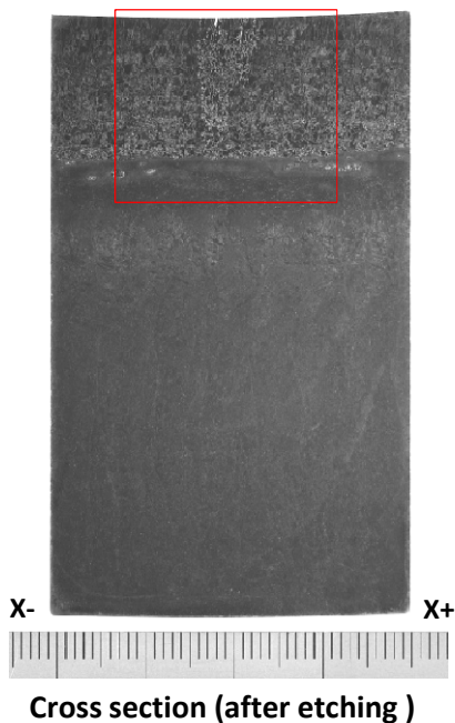
Fig. A-1.12 Detailed crack information at Y= - 11 section in P15 (JRV-S1)
