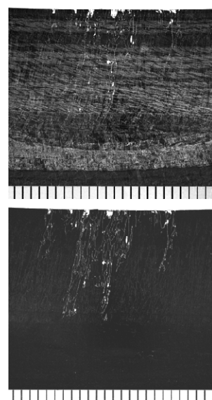
Typical photo of SCC at Y= -2 (Upper: before etching, Lower : after etching)
