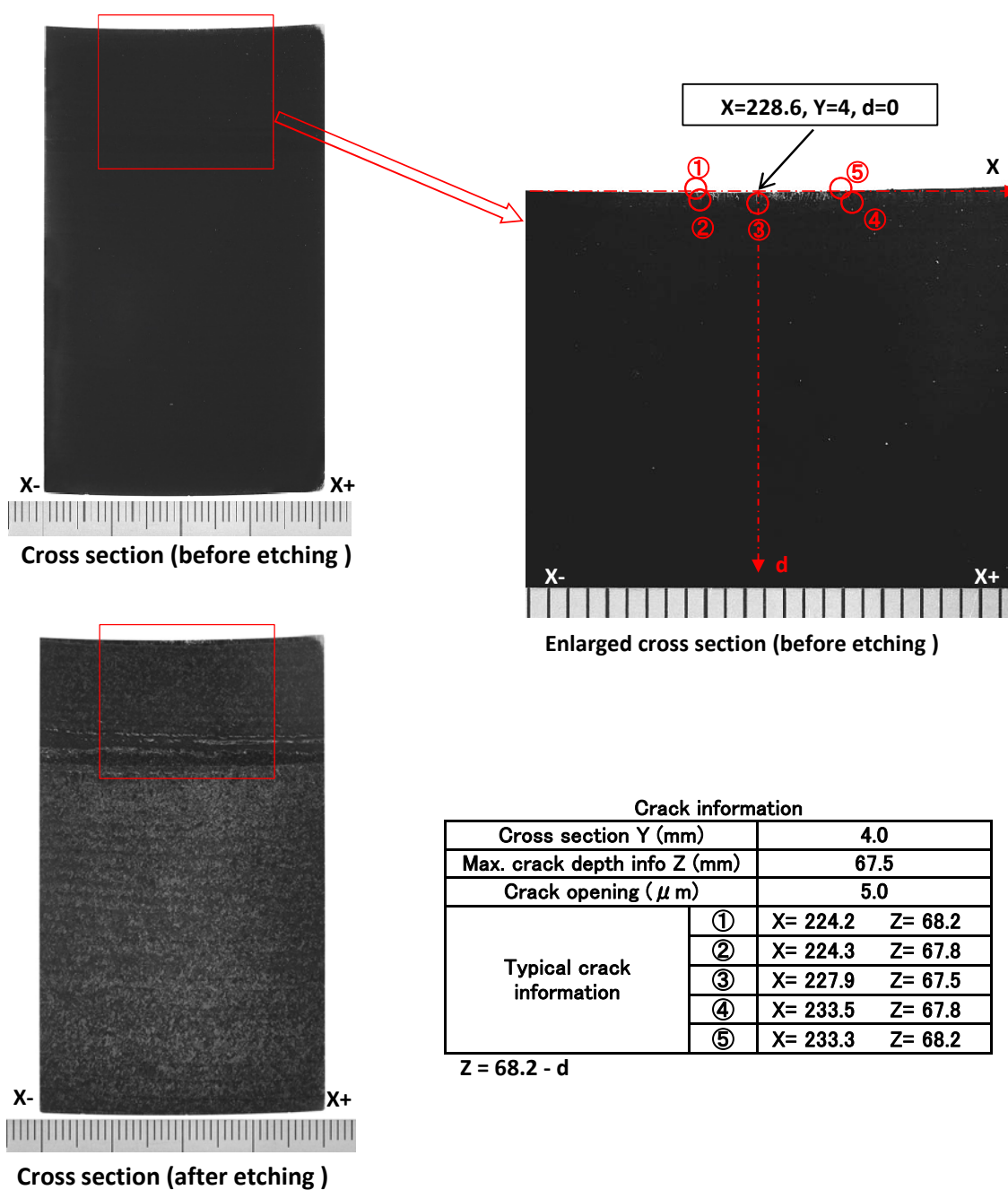
Fig. A-1.3 Detailed crack information at Y=4 section in P15 (JR-V-S1)
