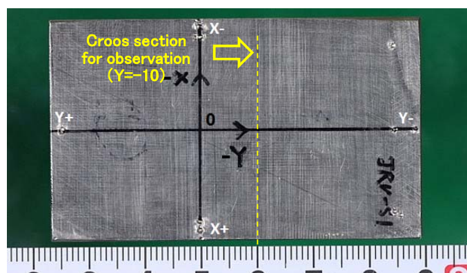
Position of cross section for observation (Y= - 10)
