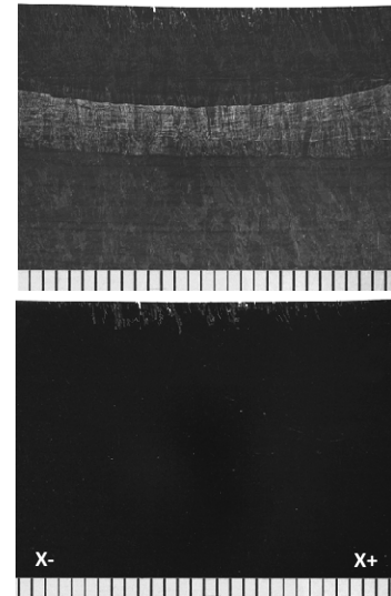
Typical photo of SCC at Y = -2 (Upper: before etching, Lower : after etching)
