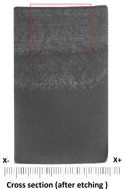
Fig. A-2.13 Detailed crack information at Y= - 11 section in P16 (JRV-S2)
