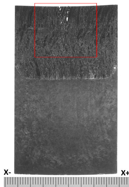
Fig. A-1.9 Detailed crack information at Y= - 5 section in P15 (JRV-S1)
