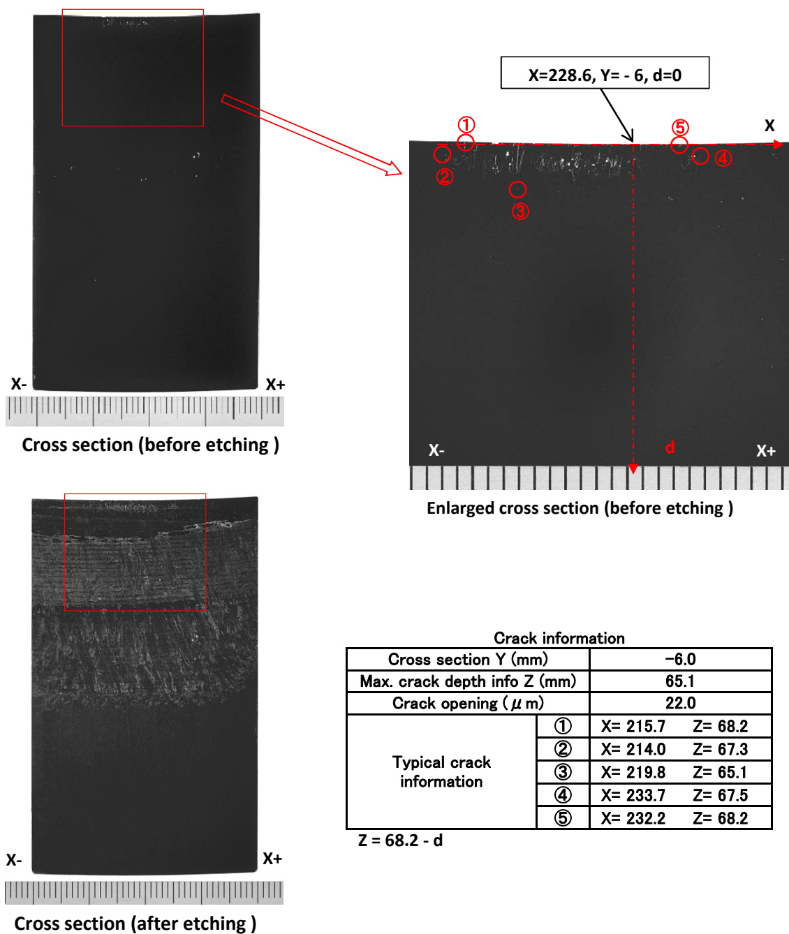
Fig. A-2.8 Detailed crack information at Y= - 6 section in P16 (JRV-S2)
