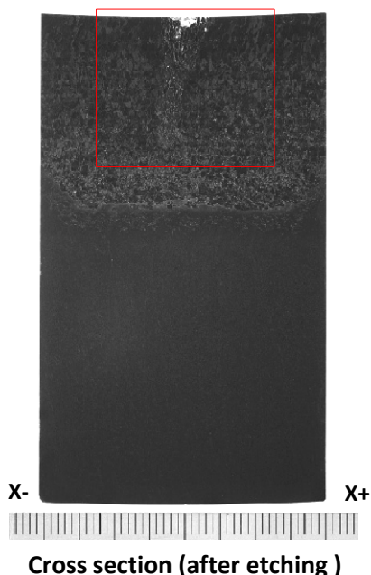
Fig. A-1.10 Detailed crack information at Y= - 9 section in P15 (JRV-S1)
