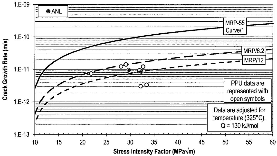
Figure 3. Plot of da/dt versus K_I for Alloy 690 HAZ Data from Heat WP142
