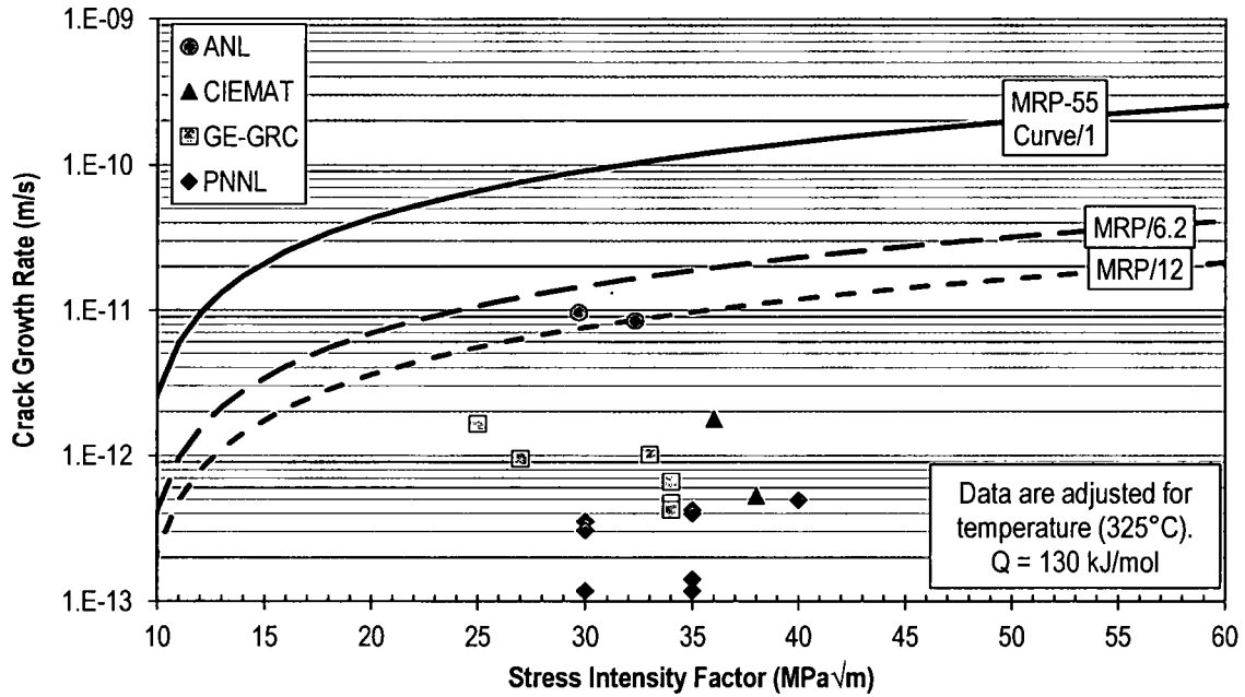
Figure 9. Plot of da/dt versus K_I for Alloy 690 HAZ Data from All Laboratories, \leq 10\% Cold Work, Constant Load or K_I
