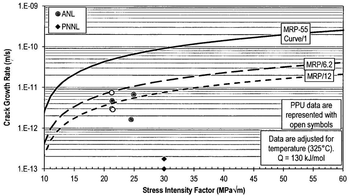
Figure 24. Plot of da/dt versus K_I for Alloy 690 Data from Heat WP142
