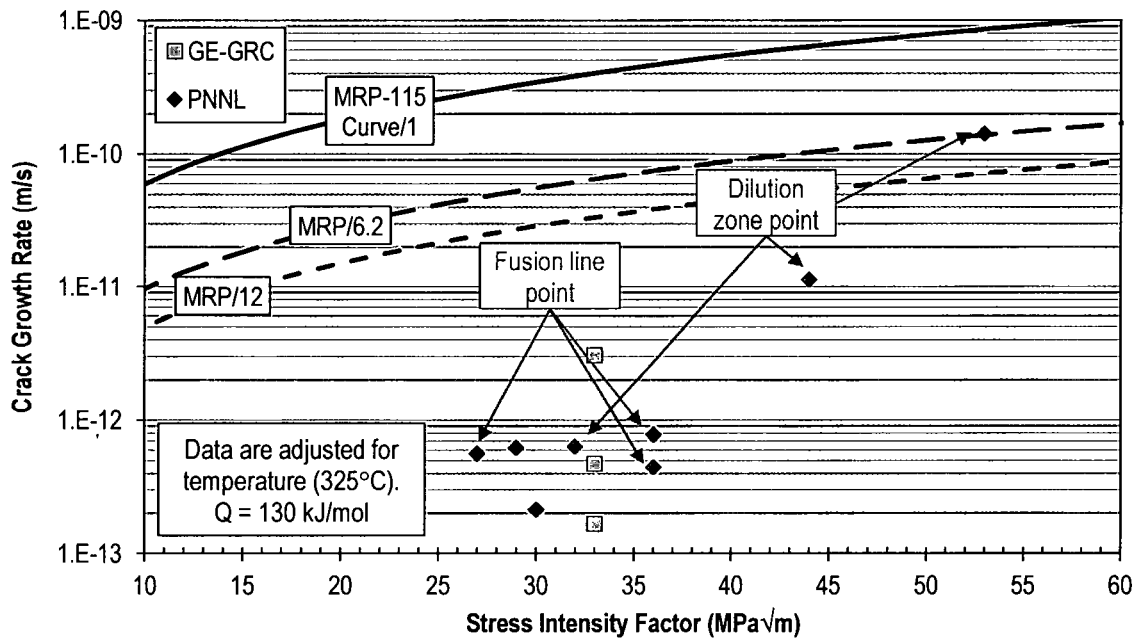
Figure 5. Plot of da/dt versus K_I for Alloy 152 Data from Heat WC83F8
