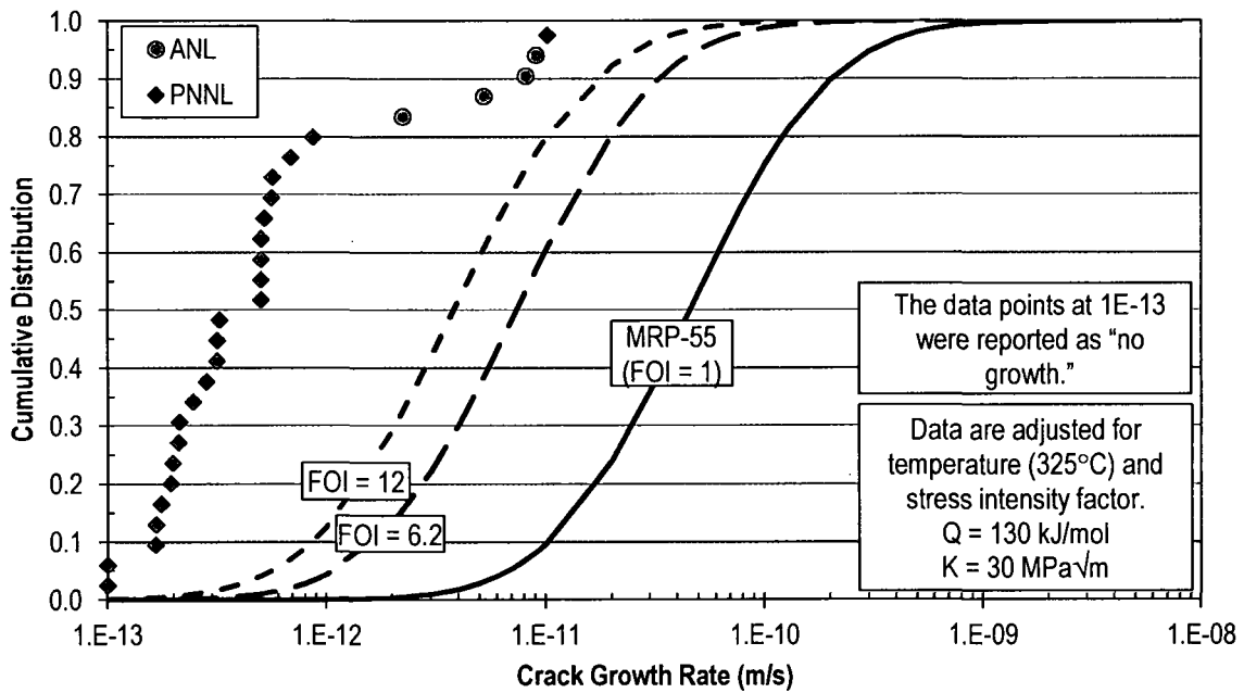
Figure 15. Cumulative Distribution Function of Adjusted da/dt Alloy 690 Data Produced by ANL and PNNL and Available in Public References, \leq 20\% Cold Work
