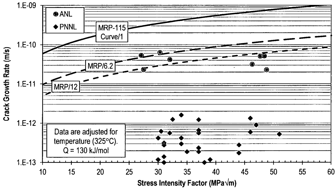
Figure 18. Plot of da/dt versus K_I for Alloy 52/152 Data Produced by ANL and PNNL and Available in Public References, \leq 20\% Cold Work
