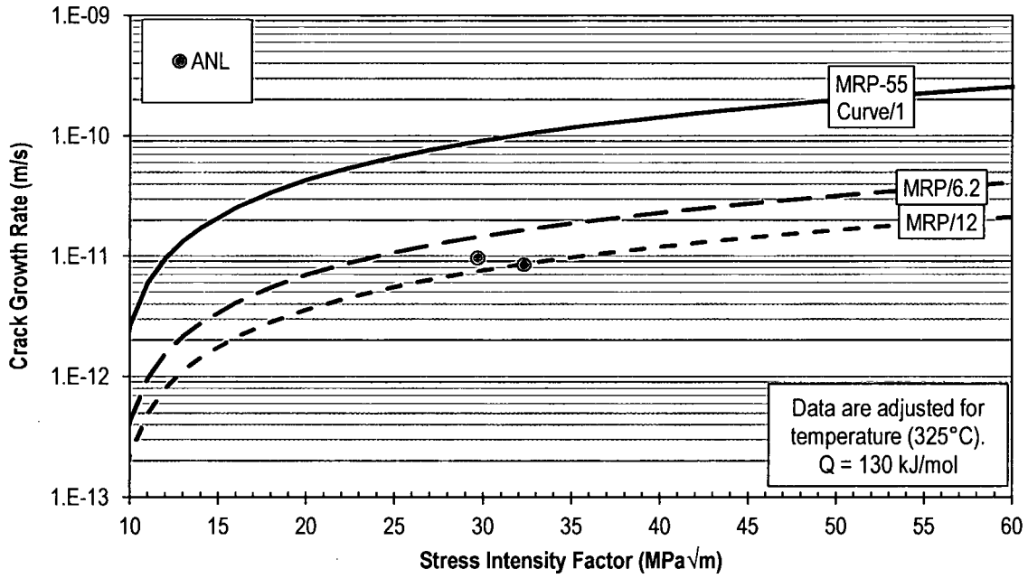
Figure 16. Plot of da/dt versus K_I for Alloy 690 HAZ Data Produced by ANL and PNNL and Available in Public References, \leq 20\% Cold Work
