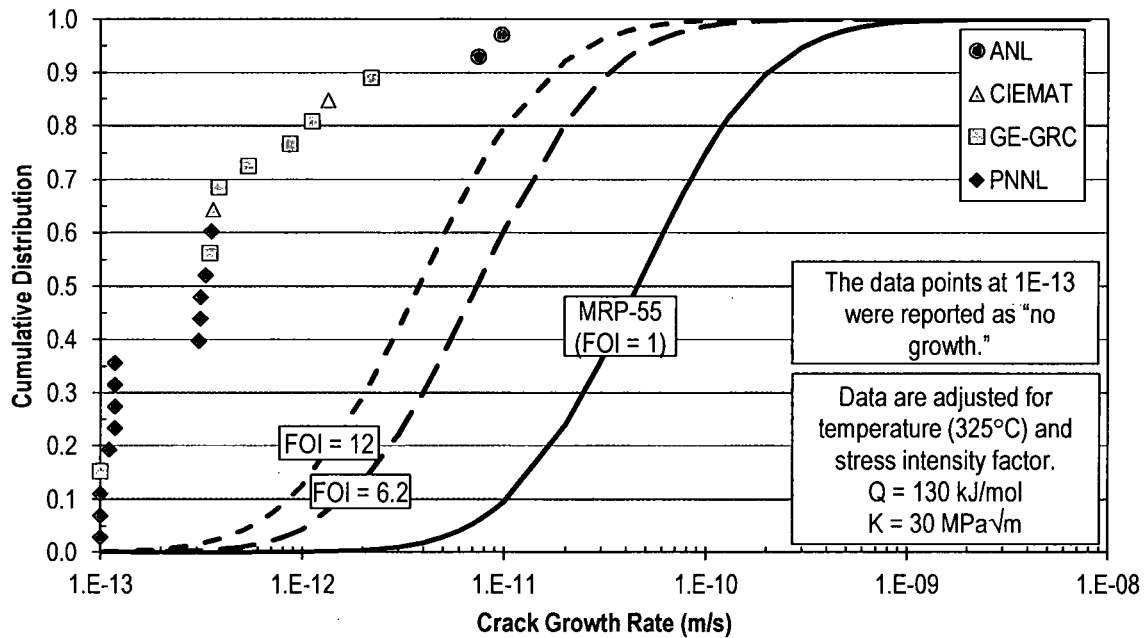
Figure 10. Cumulative Distribution Function of Adjusted da/dt for Alloy 690 HAZ Data from All Laboratories, \leq 10\% Cold Work, Constant Load or K_I
