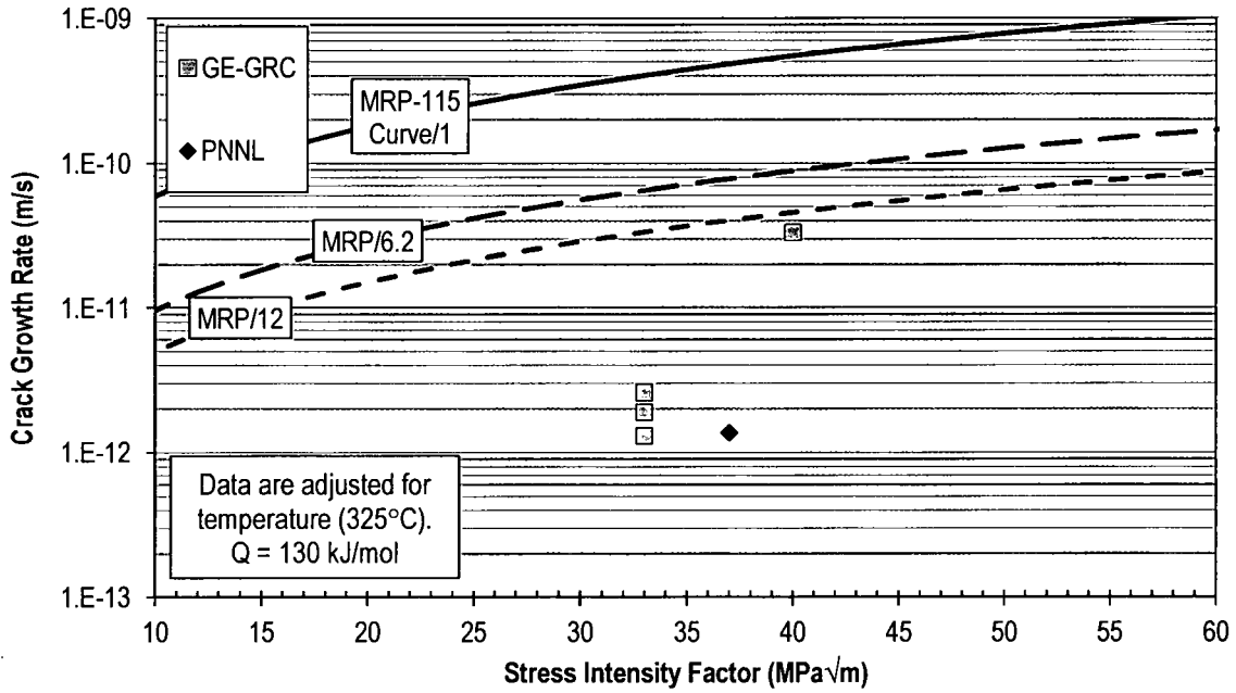
Figure 22. Plot of da/dt versus K_I for Alloy 52/152 Data from All Laboratories, > 10 & \leq 20\% Cold Work, Constant Load or K_I
