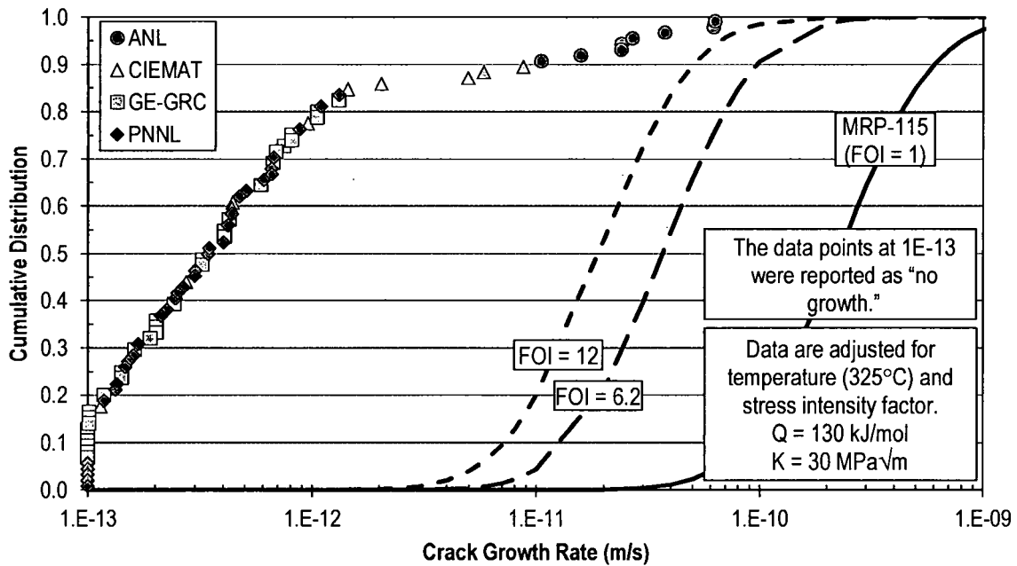
Figure 12. Cumulative Distribution Function of Adjusted da/dt for Alloy 52/152 Data from All Laboratories, \leq 10\% Cold Work, Constant Load or K_I
