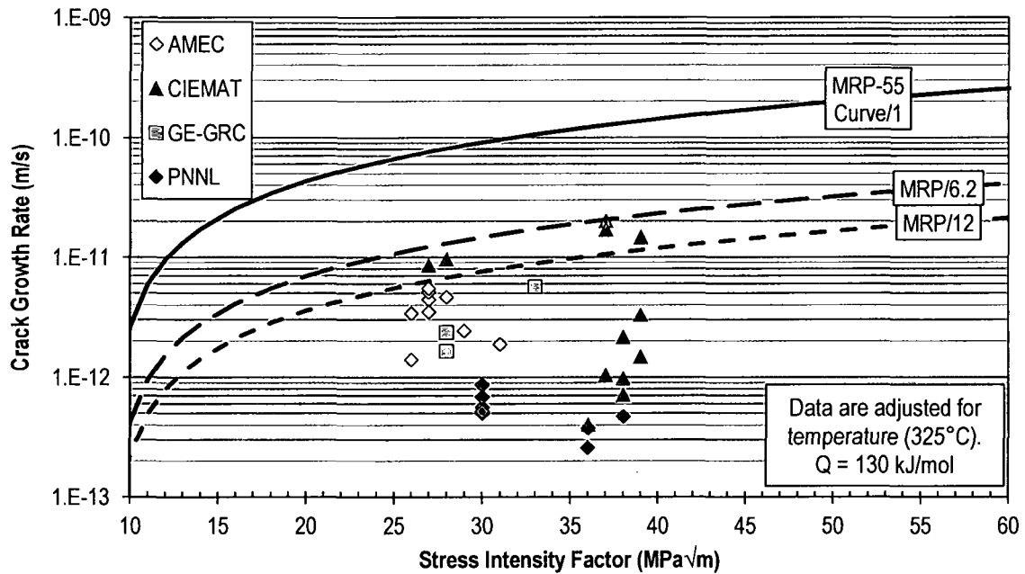
Figure 20. Plot of da/dt versus K_I for Alloy 690 Data from All Laboratories, > 10 & \leq 20\% Cold Work, CRDM and Bar Material, Constant Load or K_I Testing
