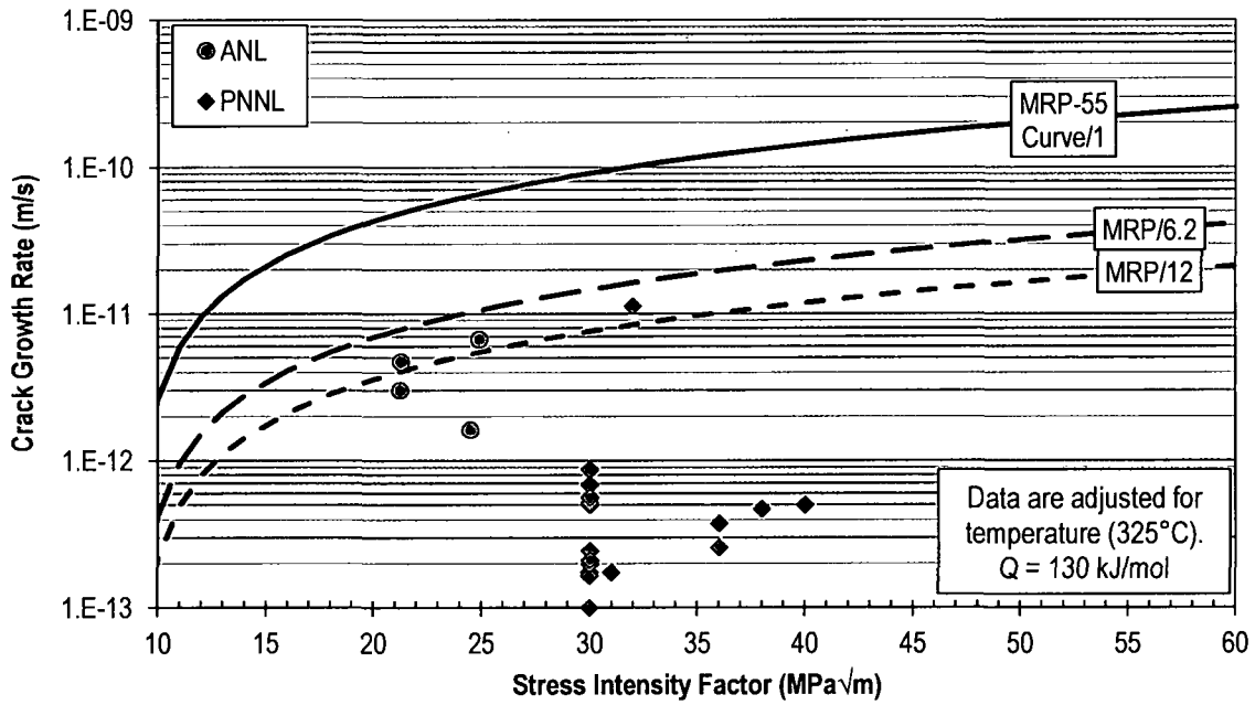
Figure 14. Plot of da/dt versus K_I for Alloy 690 Data Produced by ANL and PNNL and Available in Public References, \leq 20\% Cold Work
