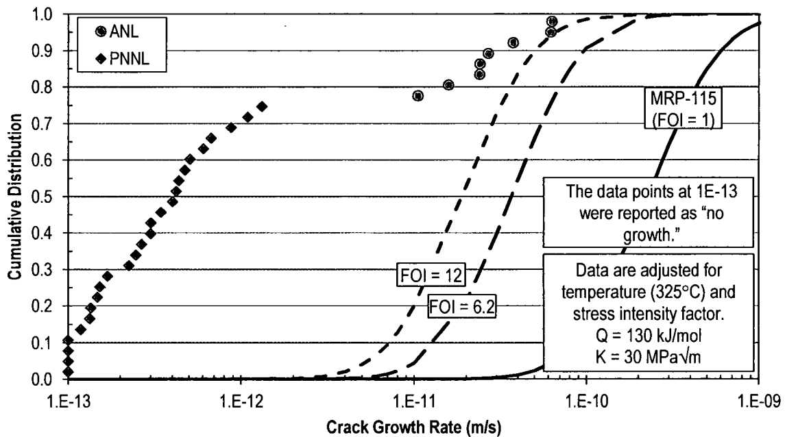
Figure 19. Cumulative Distribution Function of Adjusted da/dt Alloy 52/152 Data Produced by ANL and PNNL and Available in Public References, \leq 20\% Cold Work
