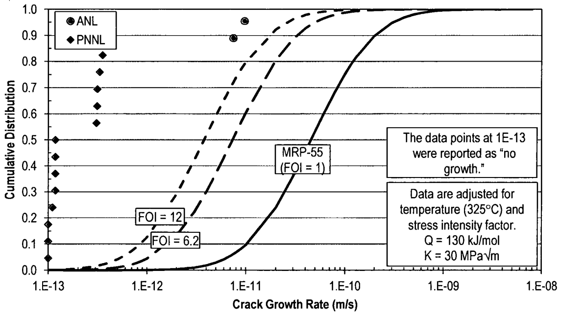
Figure 17. Cumulative Distribution Function of Adjusted da/dt Alloy 690 HAZ Data Produced by ANL and PNNL, Including Data Not Openly Published, \leq 20\% Cold Work
