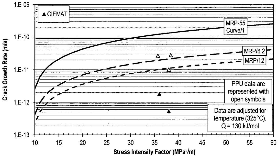
Figure 4. Plot of da/dt versus K_I for Alloy 690 HAZ Data from Plate Material Tested by CIEMAT
