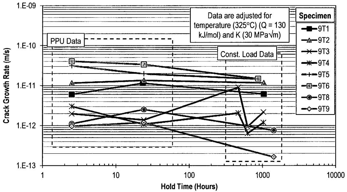
Figure 13. Plot of da/dt versus Loading Hold Time (for PPU testing) or Test Segment Duration (for Constant K_I /Load Testing) from Heat WP787
