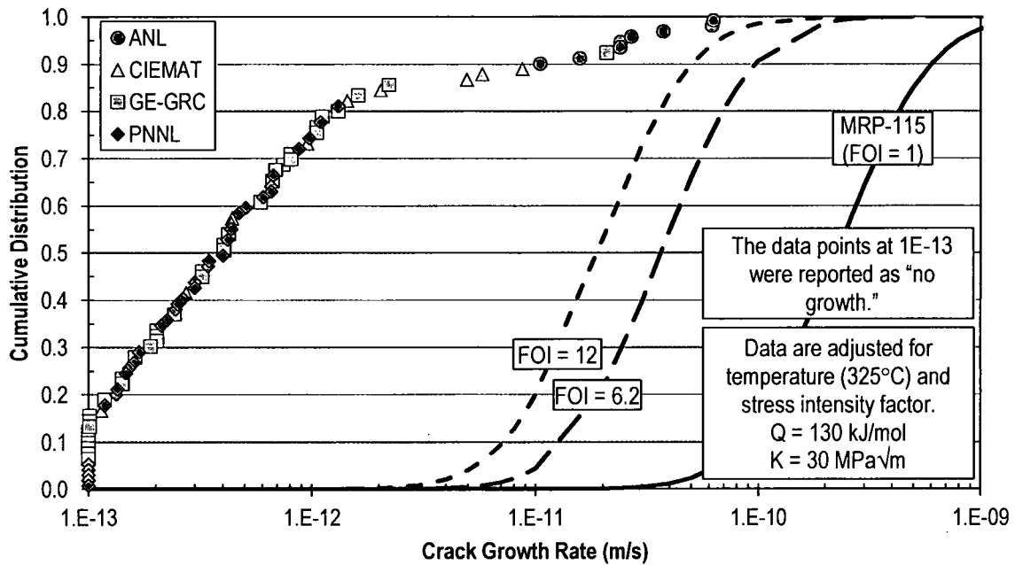
Figure 23. Cumulative Distribution Function of Adjusted da/dt Alloy 52/152 Data from All Laboratories, \leq 20\% Cold Work, Constant Load or K_I
