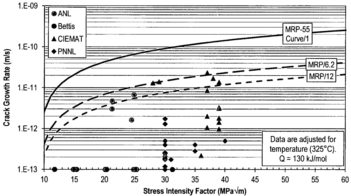
Figure 7. Plot of da/dt versus K_I for Alloy 690 Data from All Laboratories, \leq 10\% Cold Work, Constant Load or K_I
