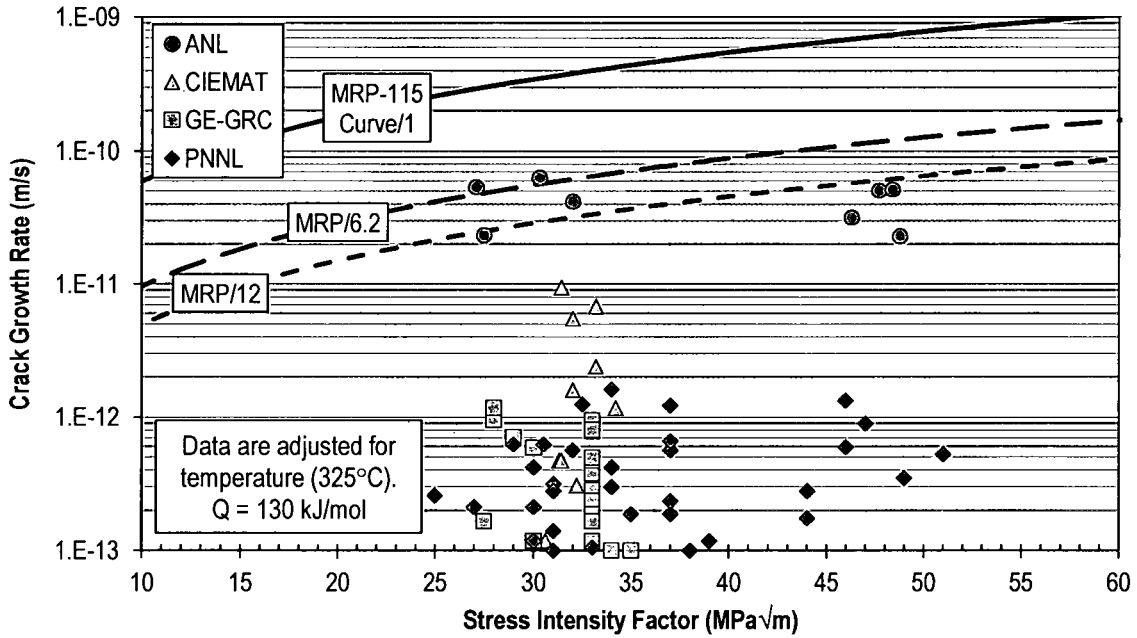
Figure 11. Plot of da/dt versus K_I for Alloy 52/152 Data from All Laboratories, \leq 10\% Cold Work, Constant Load or K_I
