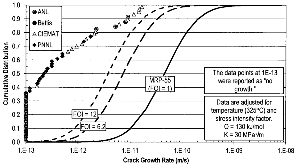
Figure 8. Cumulative Distribution Function of Adjusted da/dt for Alloy 690 Data from All Laboratories, \leq 10\% Cold Work, Constant Load or K_I
