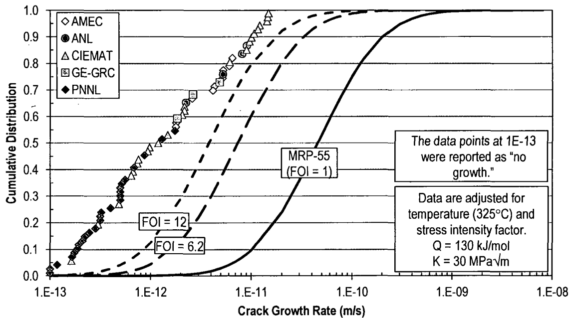
Figure 21. Cumulative Distribution Function of Adjusted da/dt Alloy 690 Data from All Labs, \leq 20\% Cold Work, CRDM and Bar Material, Constant Load or K_I
