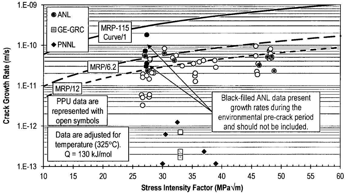
Figure 6. Plot of da/dt versus K_I for Alloy 152 Data from Heat WC04F6
