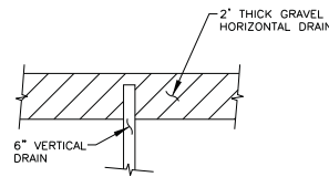
HORIZONTAL & VERTICAL DRAINS TYPICAL SECTION
