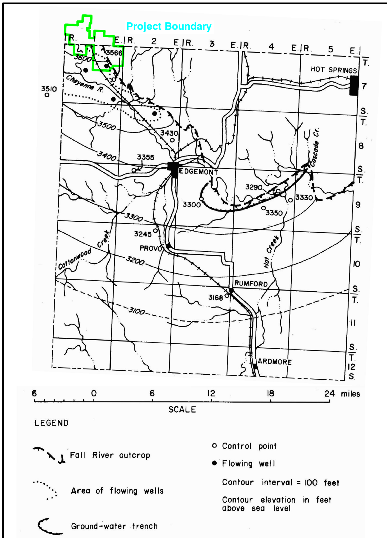
Figure 12. Probable potentiometric surface of the Fall River Formation.
