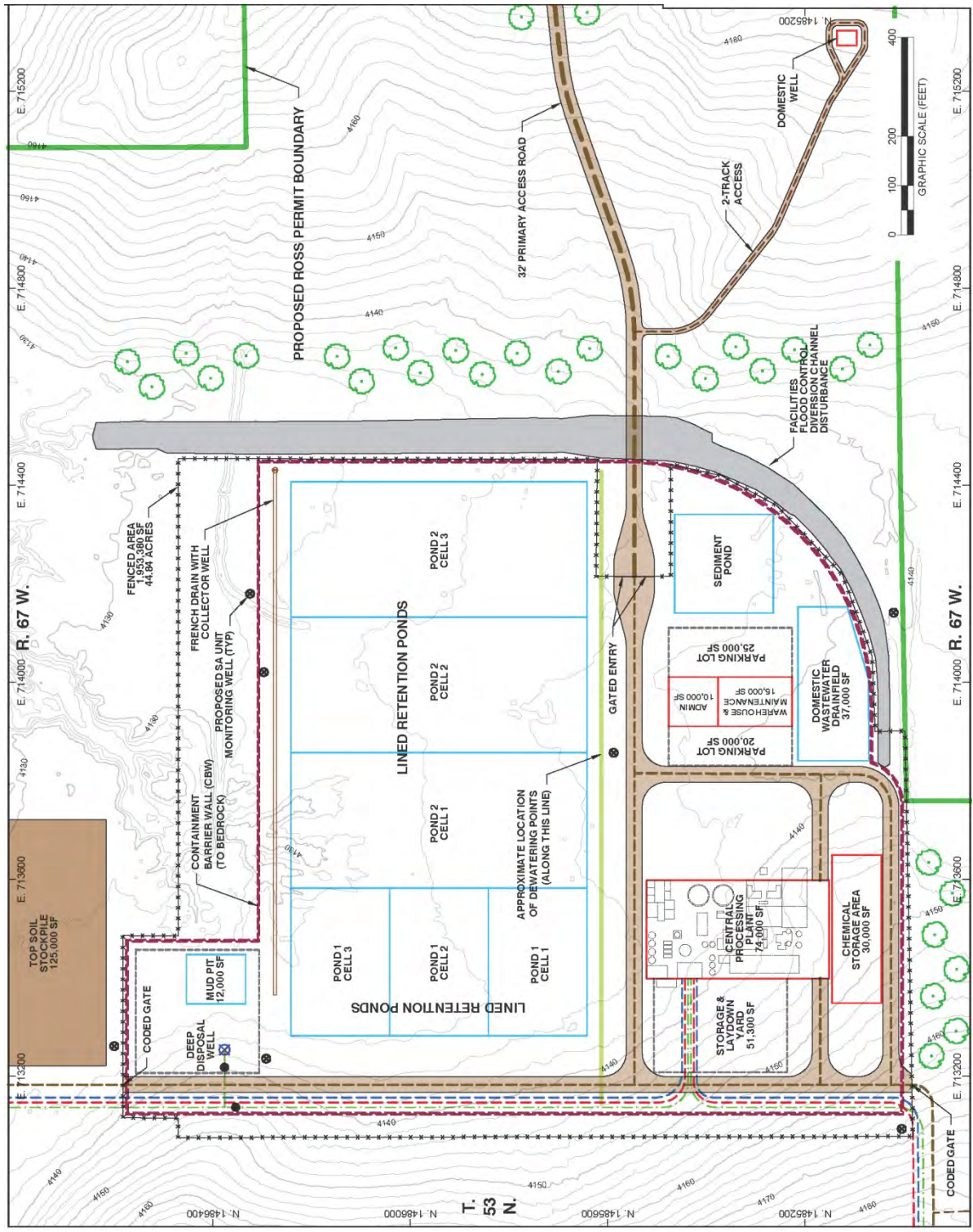
Source: Figure 3.1-16 (Strata, 2011a) Figure 3.2-1 Central Processing Plant Area Layout
