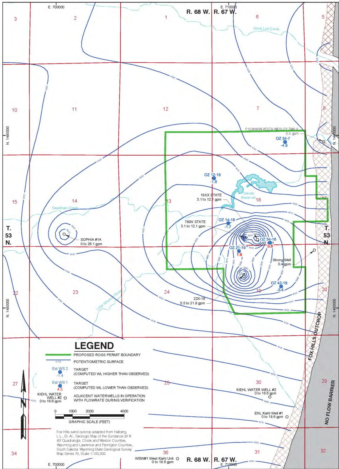
Figure 2.4-9 Contour Map of the Existing Potentiometric Surface for the OZ Aquifer
