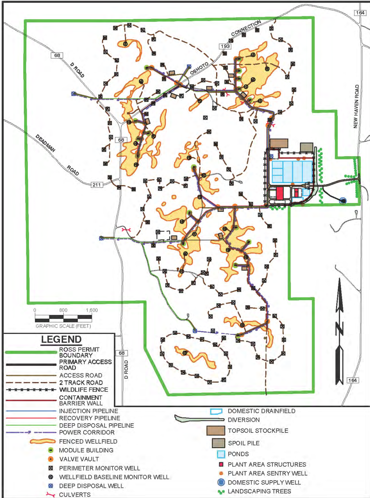
Source: Figure ER RAI GEN-1-3 (Strata, 2012a) Figure 3.1-1 Location of Ore Bodies at the Ross Project
