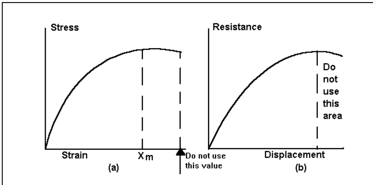
Figure 3.6.2-2 Limitations on pure tension members
