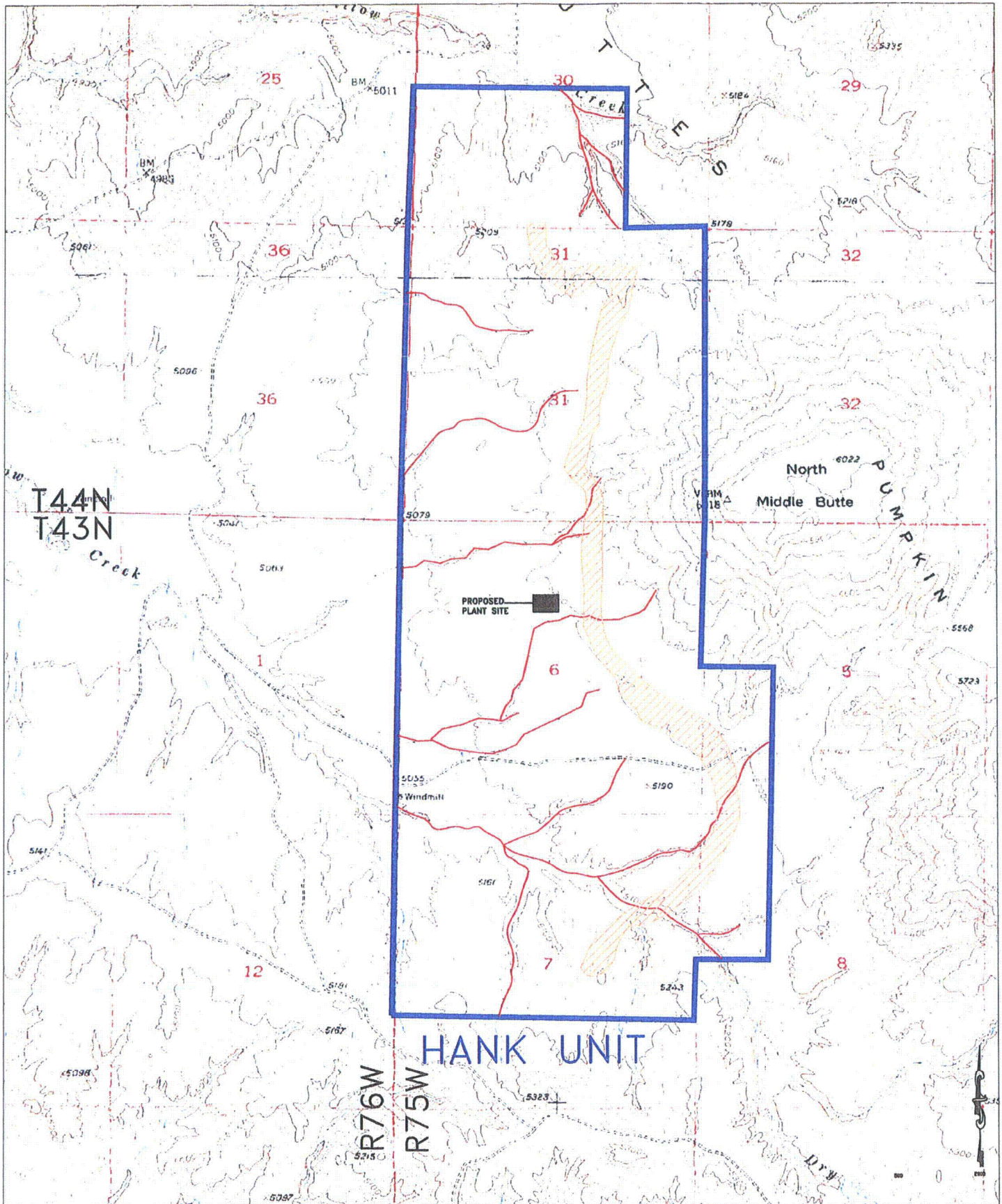
FIGURE 2-15b. HANK UNIT INUNDATED AREAS FOR 25 YEAR FLOOD
