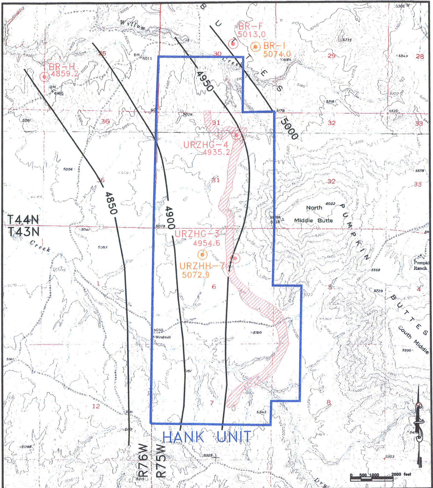
FIGURE 2-22. WATER-LEVEL ELEVATIONS FOR THE G & H SAND AQUIFERS, 2007, FT-MSL
