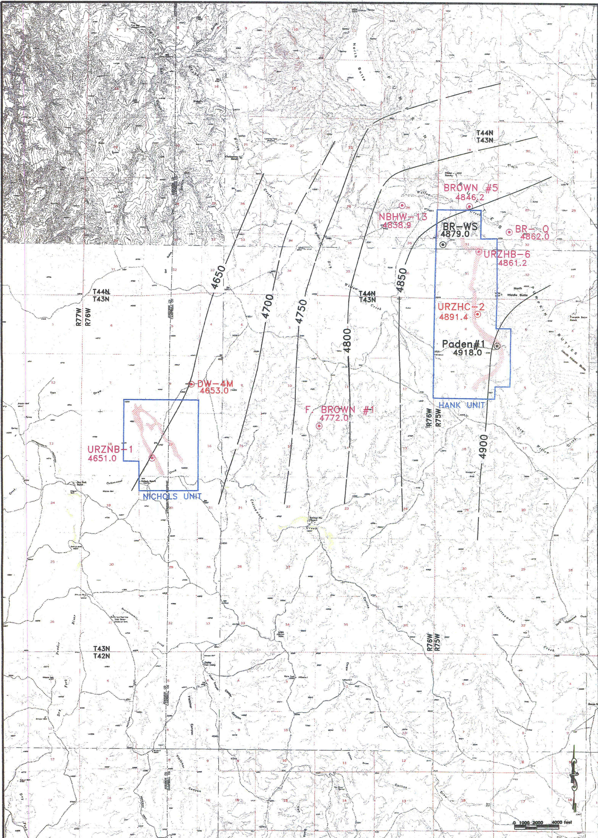
FIGURE 2-21. WATER-LEVEL ELEVATIONS FOR THE B & C SAND AQUIFERS, 2007, FT-MSL
