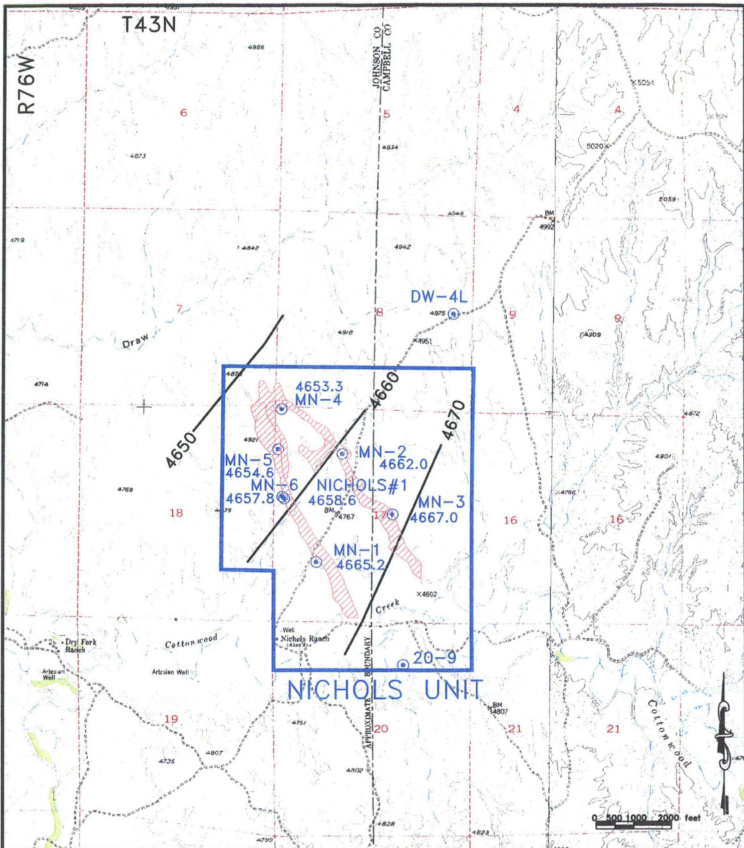
FIGURE 2-19. WATER-LEVEL ELEVATIONS FOR THE A SAND AQUIFER, 2007, FT-MSL
