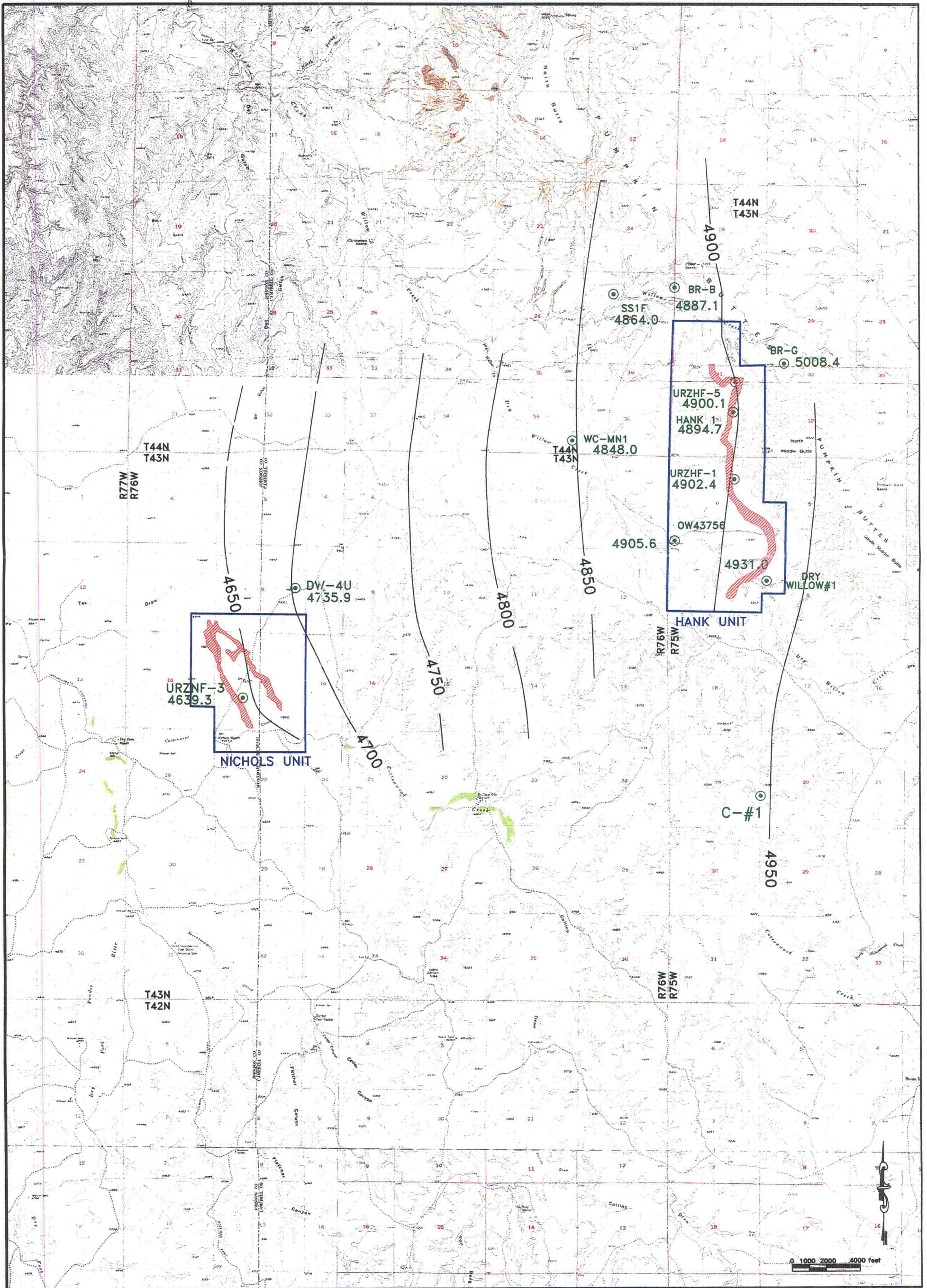
FIGURE 2-20. WATER-LEVEL ELEVATIONS FOR THE F SAND AQUIFER, 2007, FT-MSL
