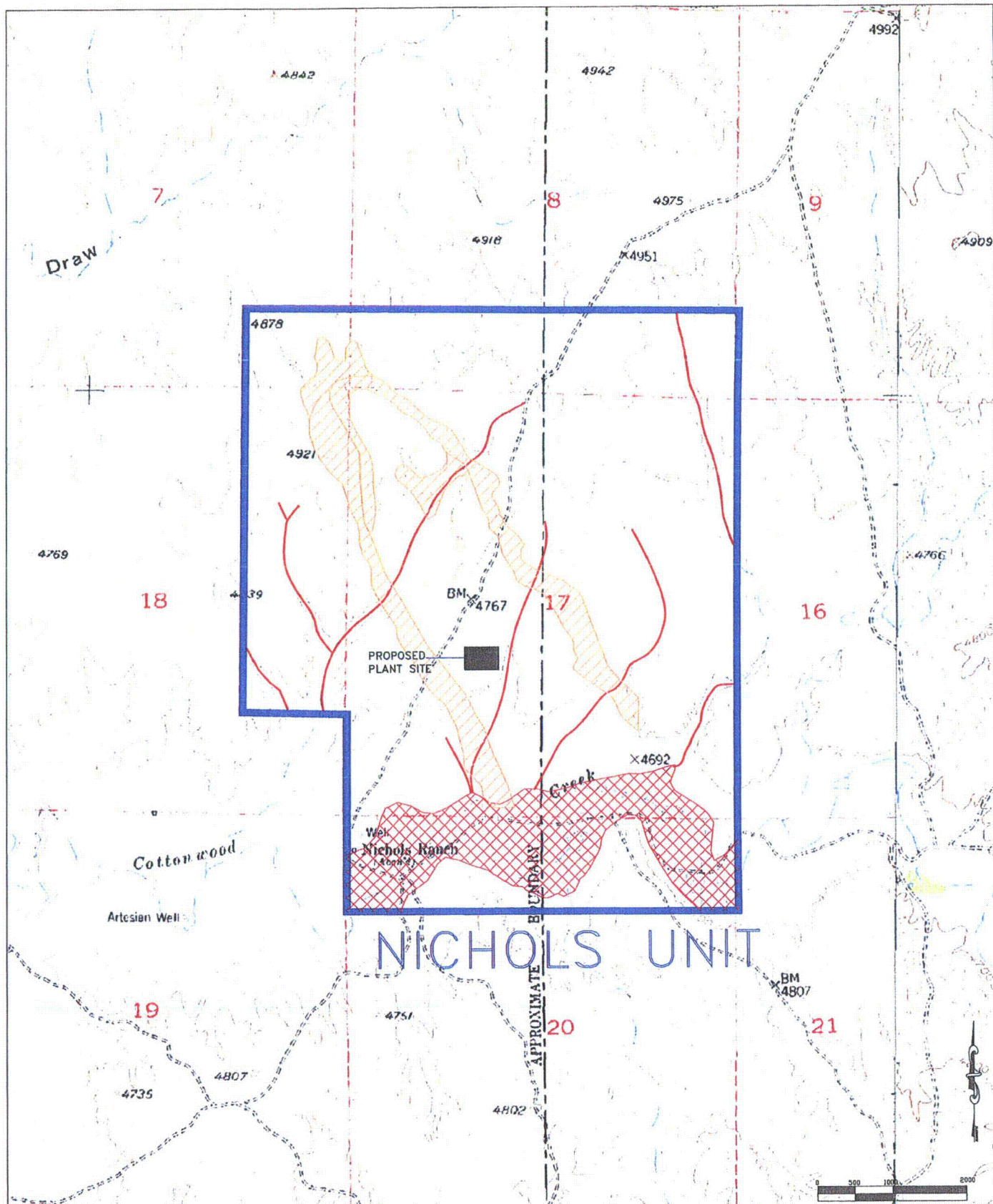
FIGURE 2-15a. NICHOLS RANCH UNIT INUNDATED AREAS FOR 25 YEAR FLOOD
