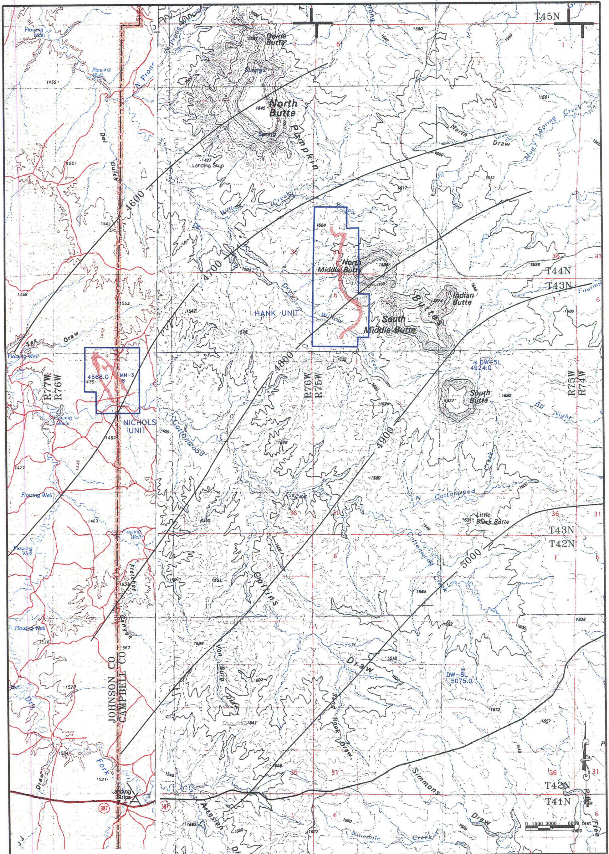
FIGURE 2-19a. REGIONAL WATER-LEVEL ELEVATION FOR THE A SAND AQUIFER, FT-MSL
