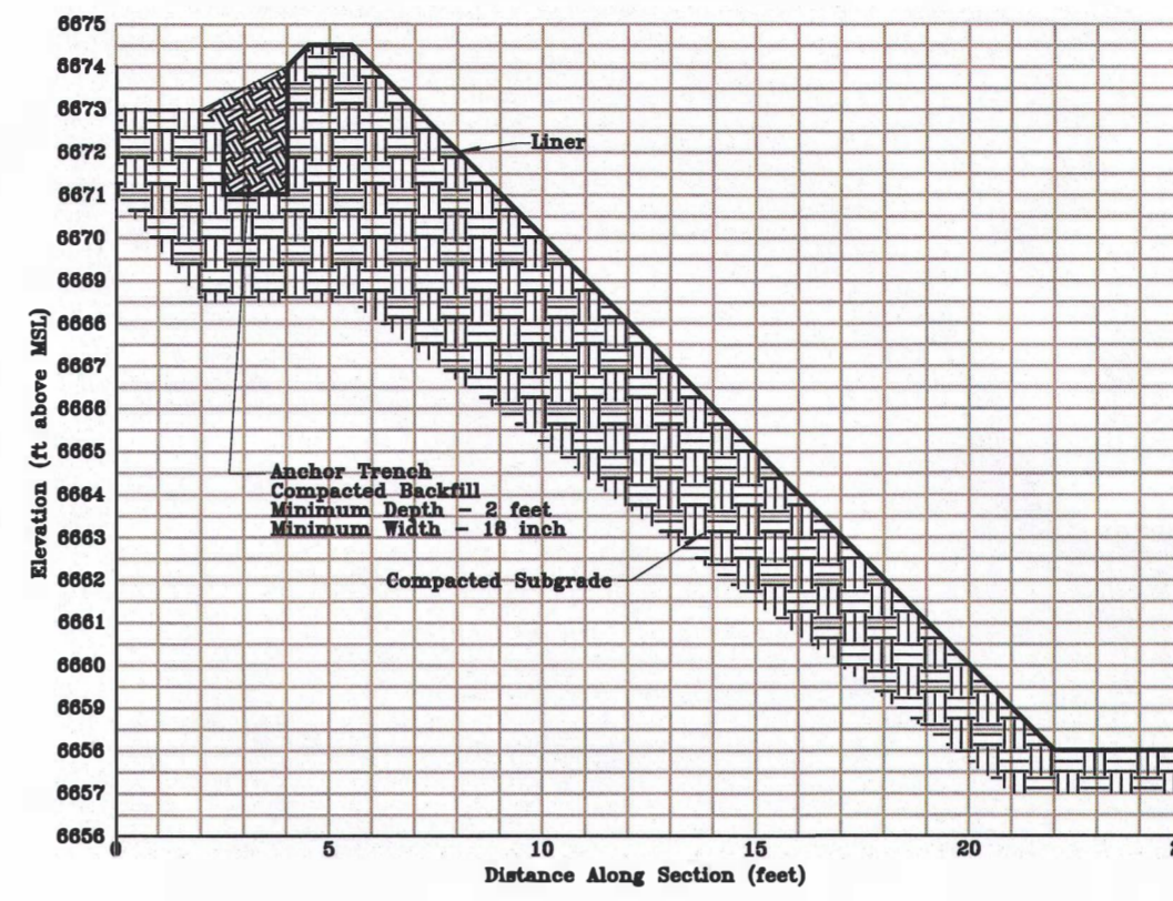
Perimeter Berm Liner Anchor Trench Section O (looking east)
