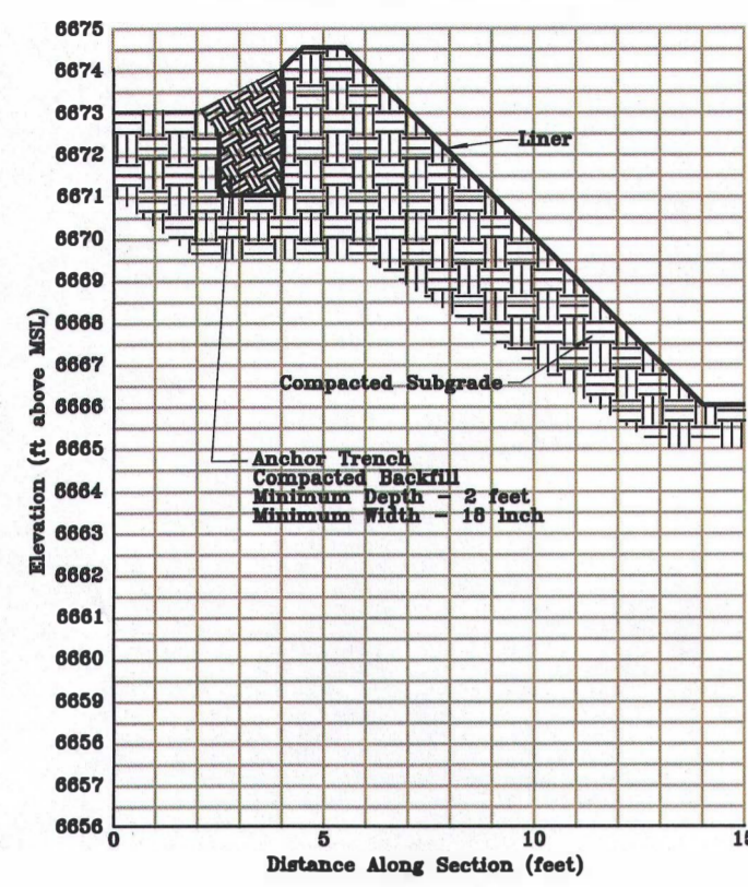
Perimeter Berm Liner Anchor Trench Section K (looking east)
