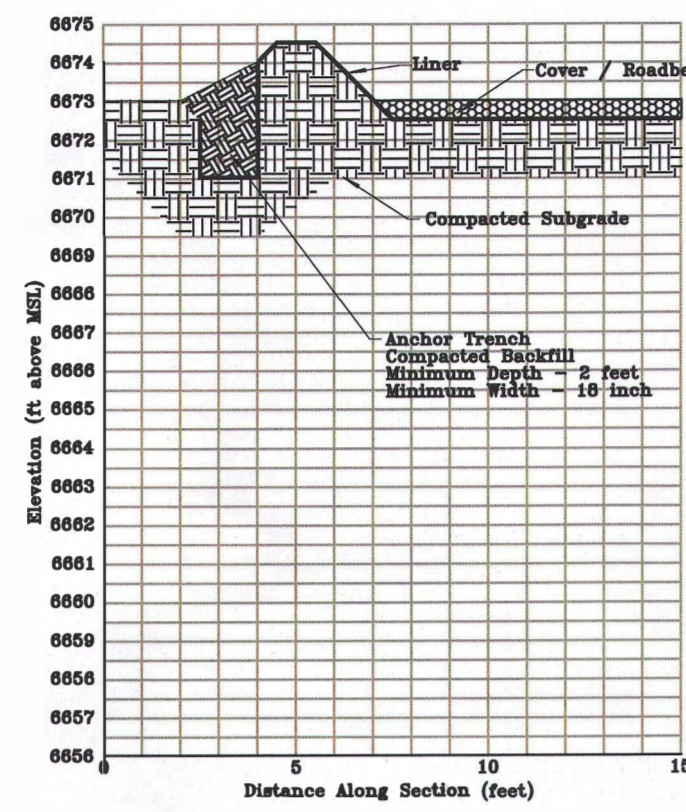
Perimeter Berm Liner Anchor Trench Section L (looking east)
