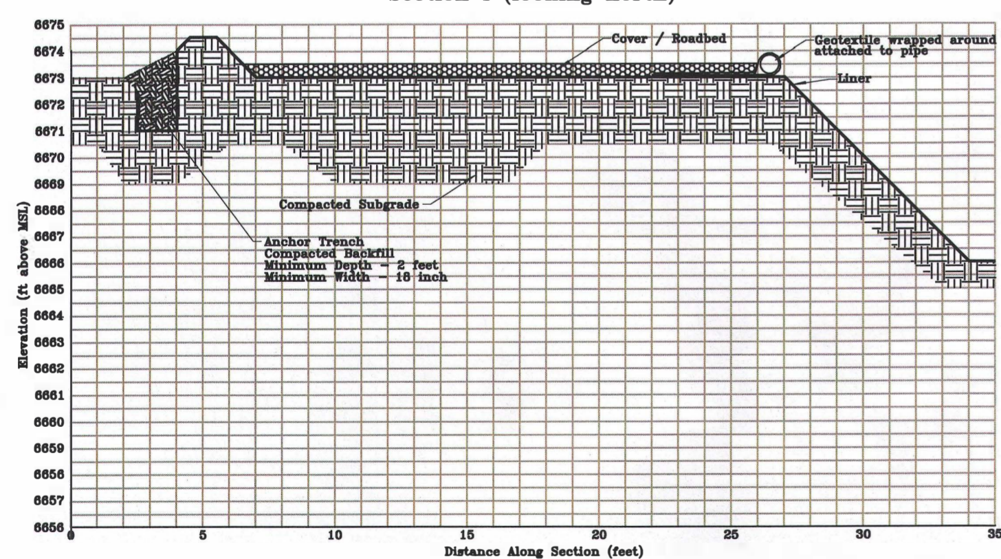
Perimeter Berm Liner Anchor Trench Section I (looking north)
