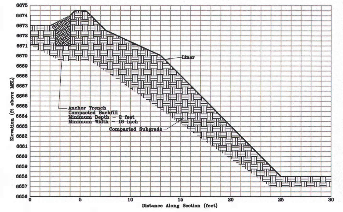
Perimeter Berm Liner Anchor Trench Section P (looking south)
