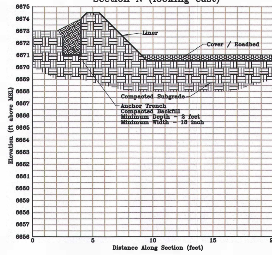
Perimeter Berm Liner Anchor Trench Section N (looking east)
