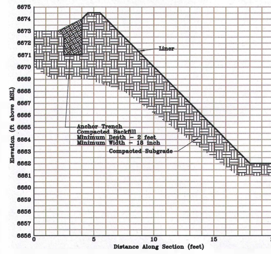
Perimeter Berm Liner Anchor Trench Section M (looking east)
