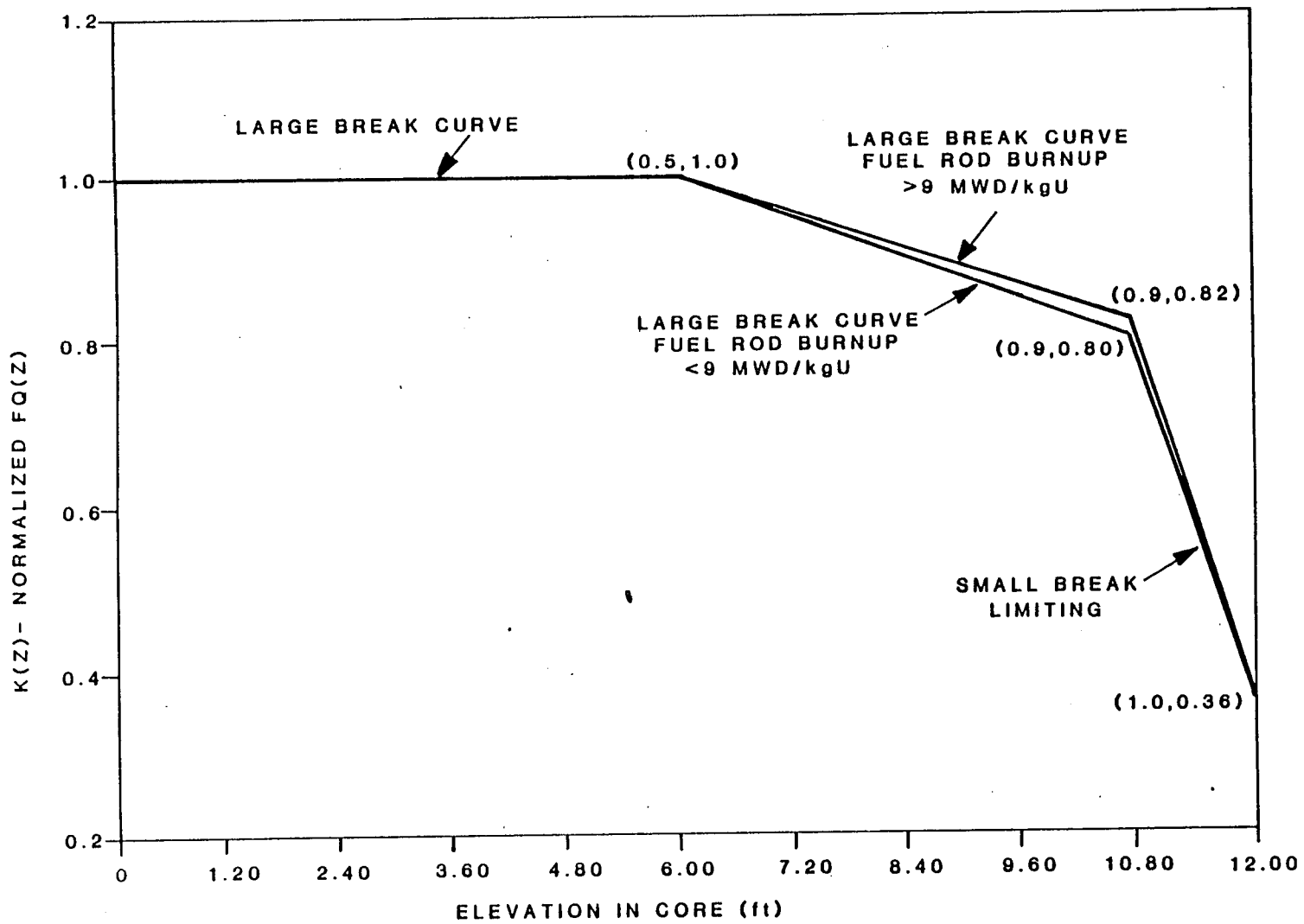
NORMALIZED AXIAL DEPENDENCE FACTOR FOR F_0^T = 2.32 VERSUS ELEVATION FOR F_{\Delta H} = 1.65
