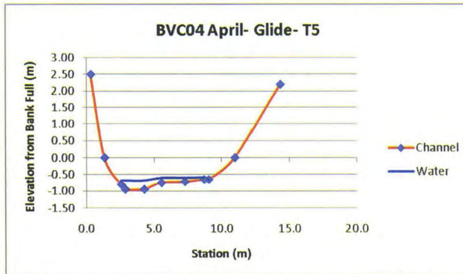
Figure 2.8-7: Channel Dimensions in Glide Habitat, Transect 5
