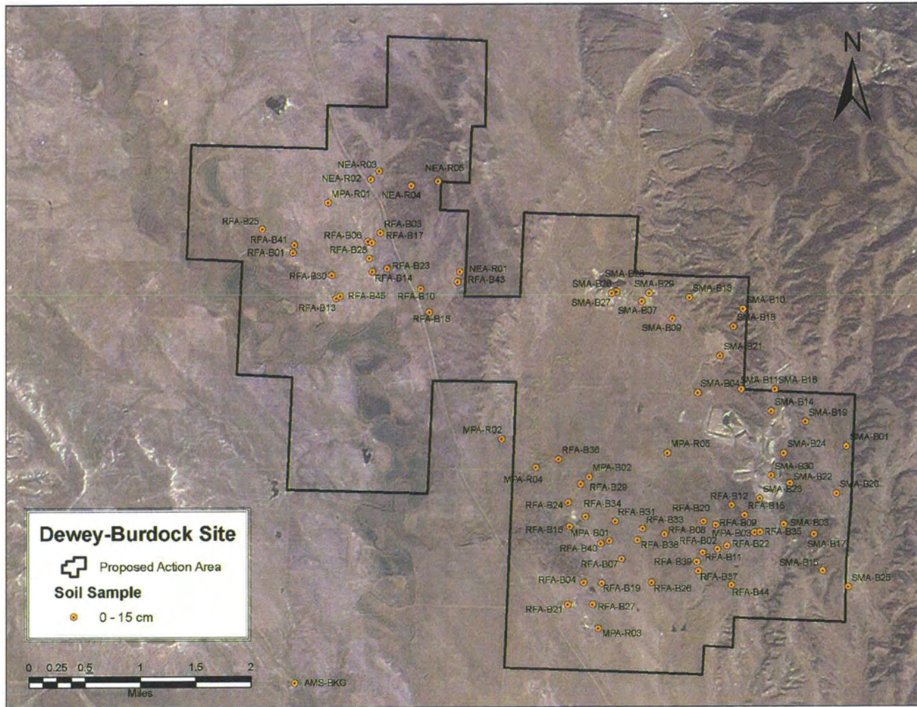
Figure 2.9-9: Surface Soil Sample Locations (80 Locations)
