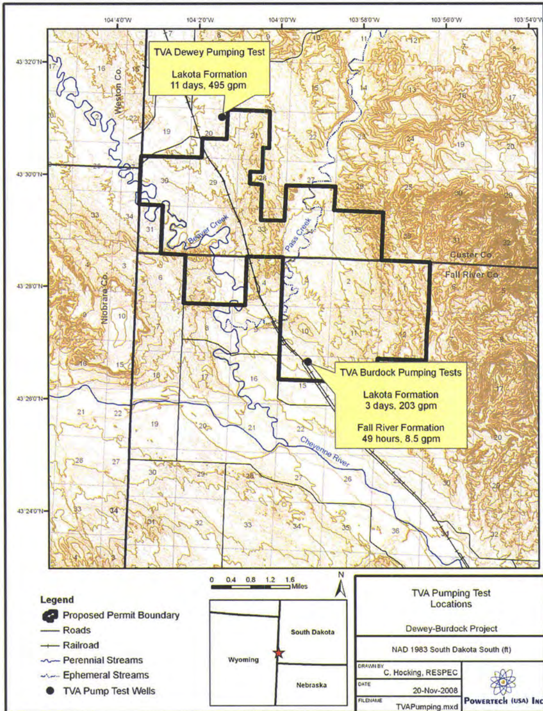
Figure 2.7-18: Location of Historical TVA Pumping Tests
