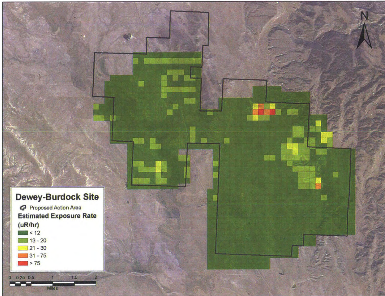
Figure 2.9-6: Predicted Site-Wide Exposure Rates, Grid Block Averages
