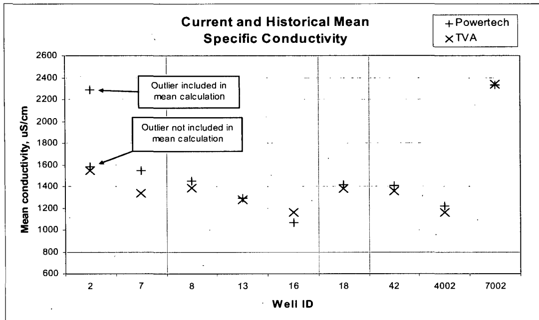
Figure 2.7-24: Mean Conductivity Comparison between Historic TVA and Current Powertech Data
