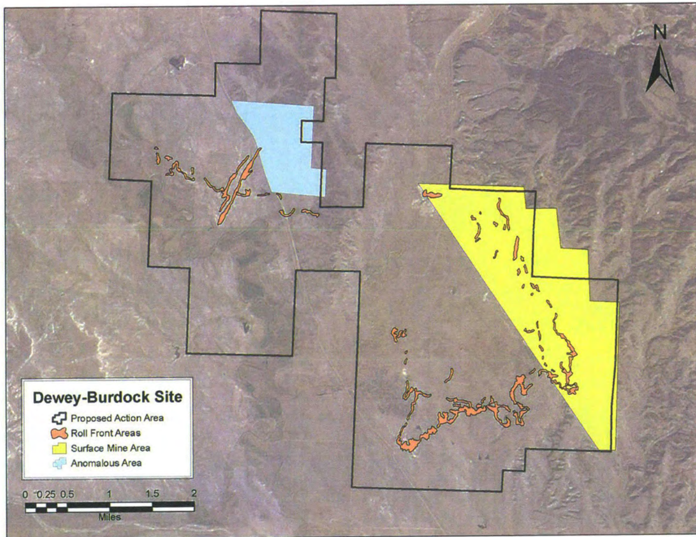
Figure 2.9-1: Areas Subject to GPS-Based Gamma Surveys
