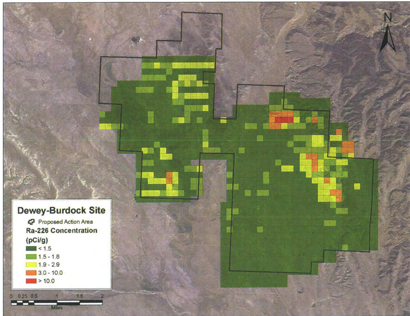
Figure 2.9-7: Predicted Site-Wide Radium-226 Concentrations, Grid Block Averages
