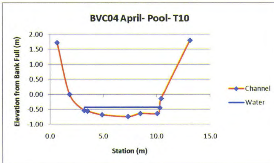
Figure 2.8-5: Channel Dimensions in Pool Habitat, Transect 10
