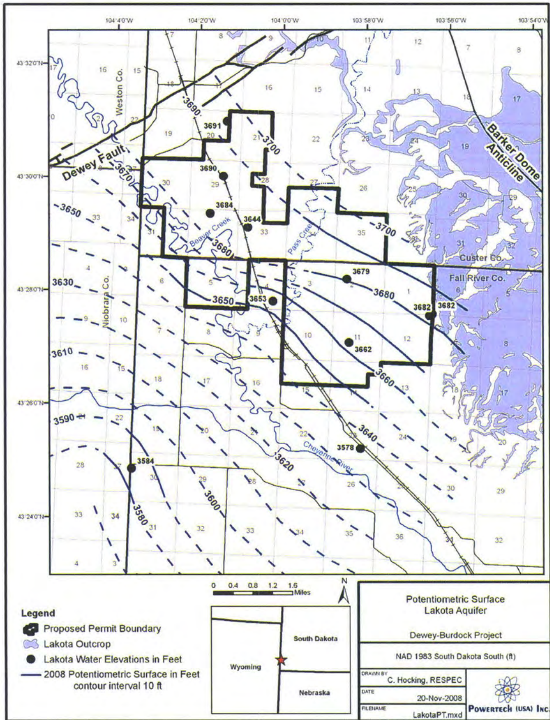
Figure 2.7-15: Potentiometric Surface of the Lakota Aquifer
