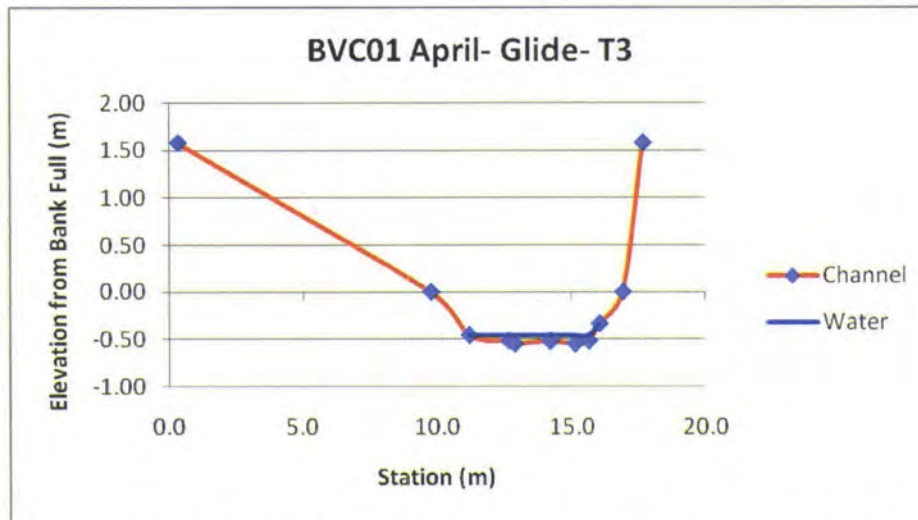
Figure 2.8-12: Channel Dimensions in Glide Habitat, Transect 3
