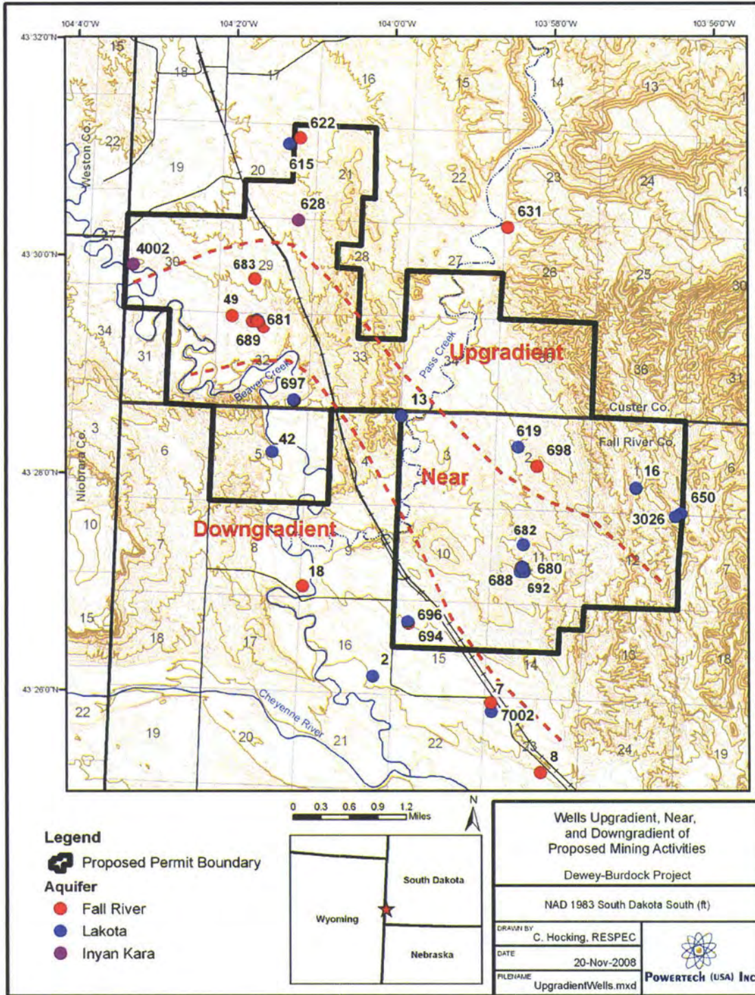
Figure 2.7-21: Wells Upgradient, Near, and Downgradient of Proposed Mining Activities
