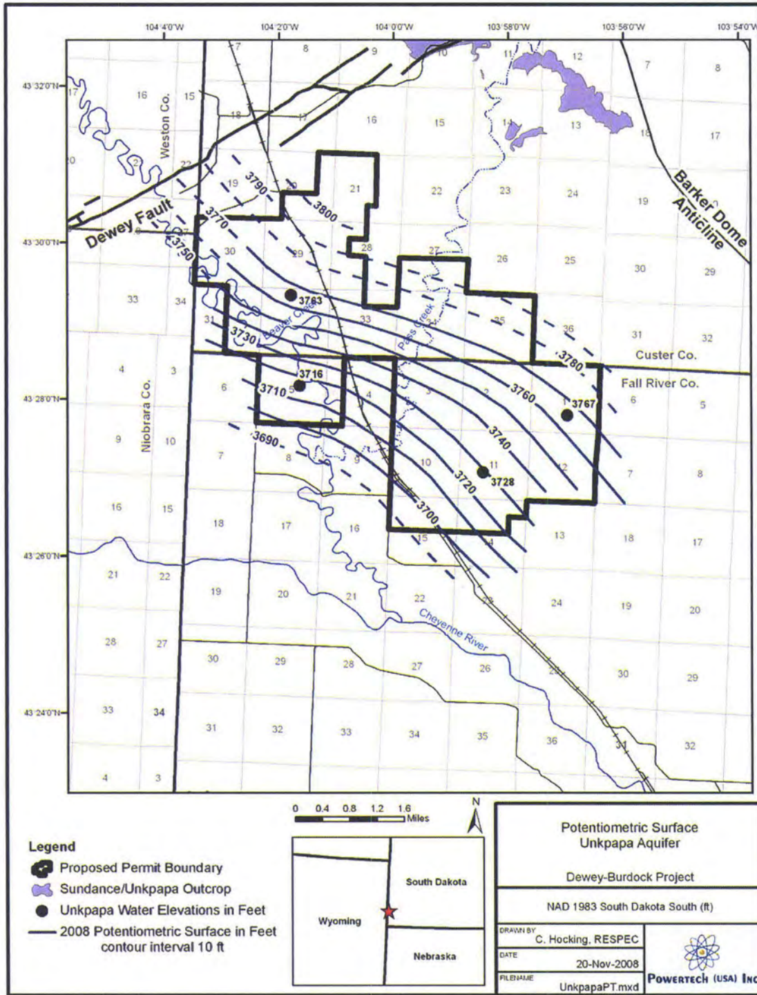
Figure 2.7-16: Potentiometric Surface of the Unkapa Aquifer
