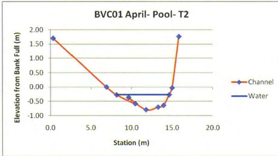
Figure 2.8-10: Channel Dimensions in Pool Habitat, Transect 2
