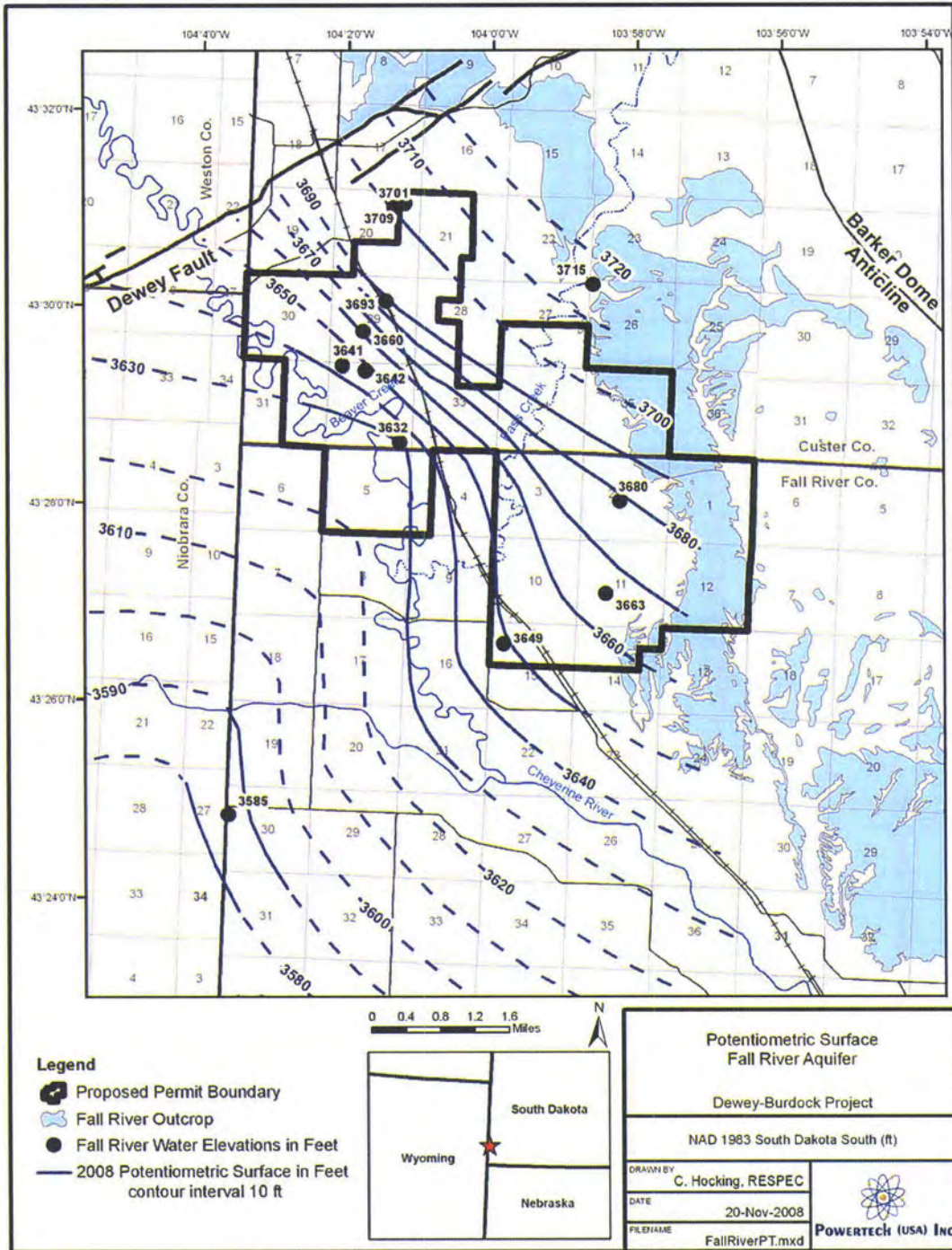
Figure 2.7-14: Potentiometric Surface of the Fall River Aquifer
