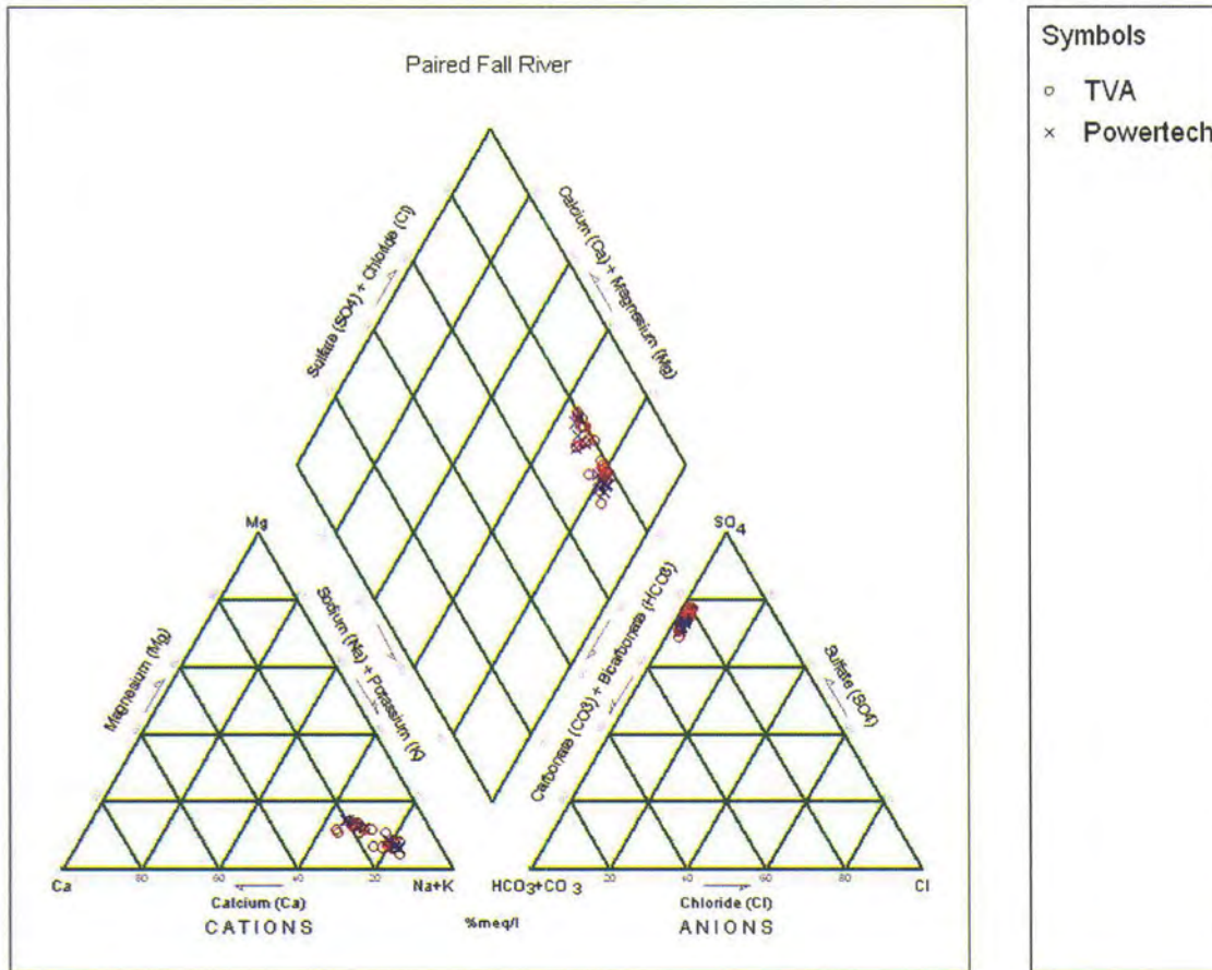
Figure 2.7-30: Piper Diagram of Sample Results from Fall River Wells Grouped by Vintage
