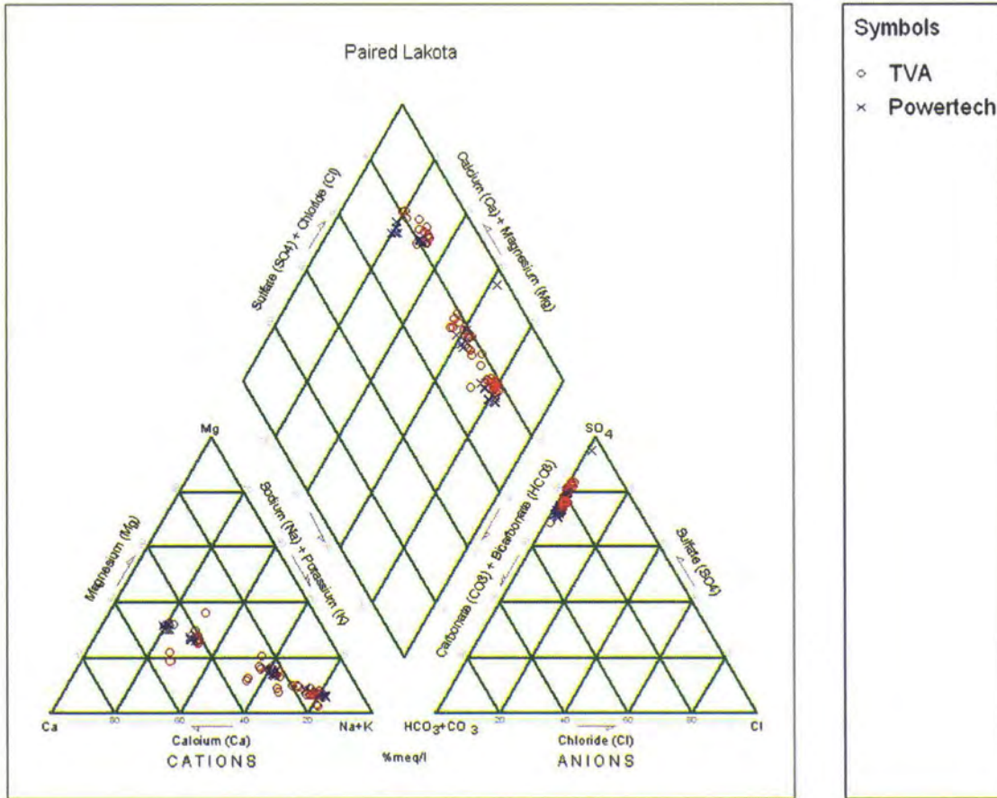
Figure 2.7-28: Piper Diagram of Sample Results from Lakota Wells Grouped by Vintage
