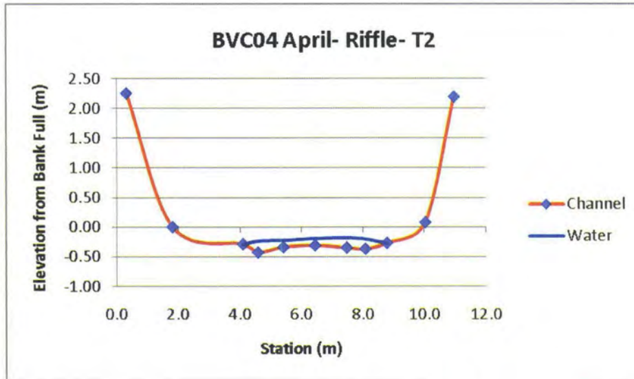
Figure 2.8-6: Channel Dimensions in Riffle Habitat, Transect 2
