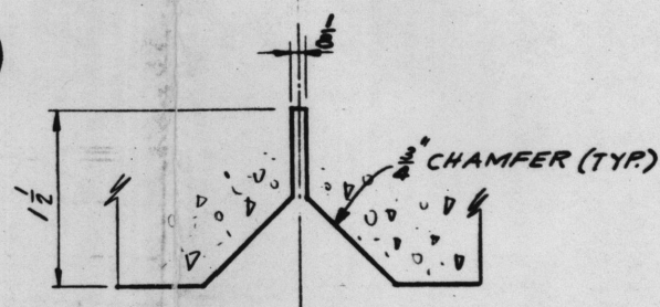
DETAIL 1 3/32" = 1'-0"
