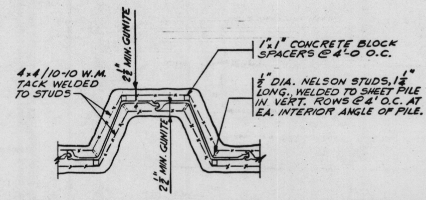
"GUNITE" FACING ON SHEET PILE WALL
