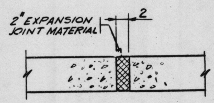
TYPICAL EXPANSION JOINT DETAIL SCALE: NONE
