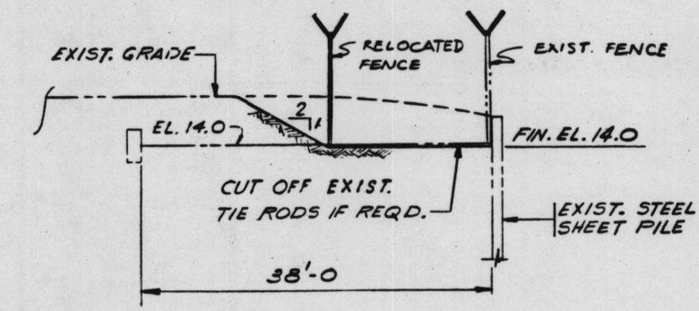
SECTION @ SOUTH OFFSHORE PAD
