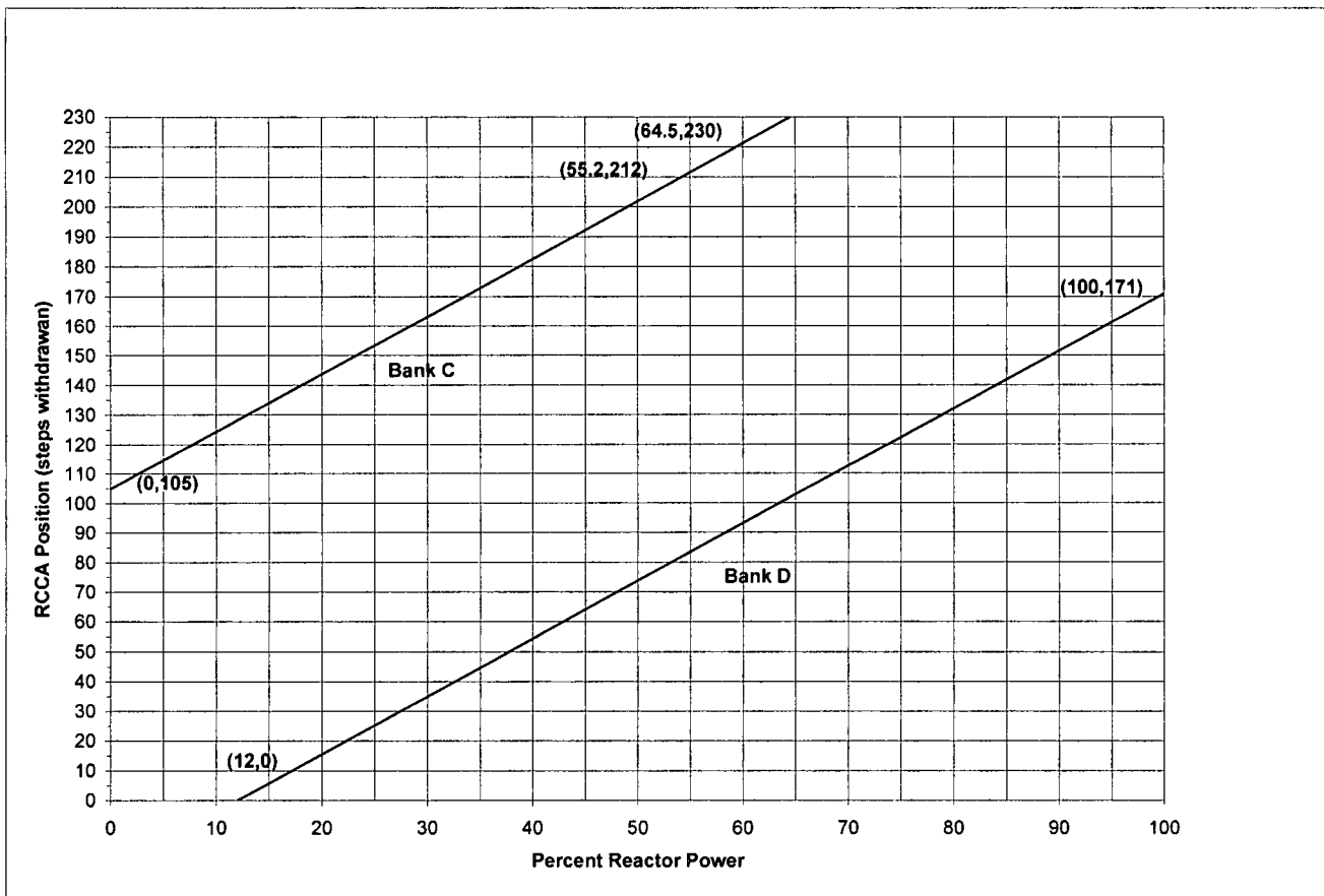
Turkey Point Unit 3 Cycle 27 Rod Insertion Limits vs Thermal Power ARO = 230 Steps Withdrawn, Overlap = 102 Steps
