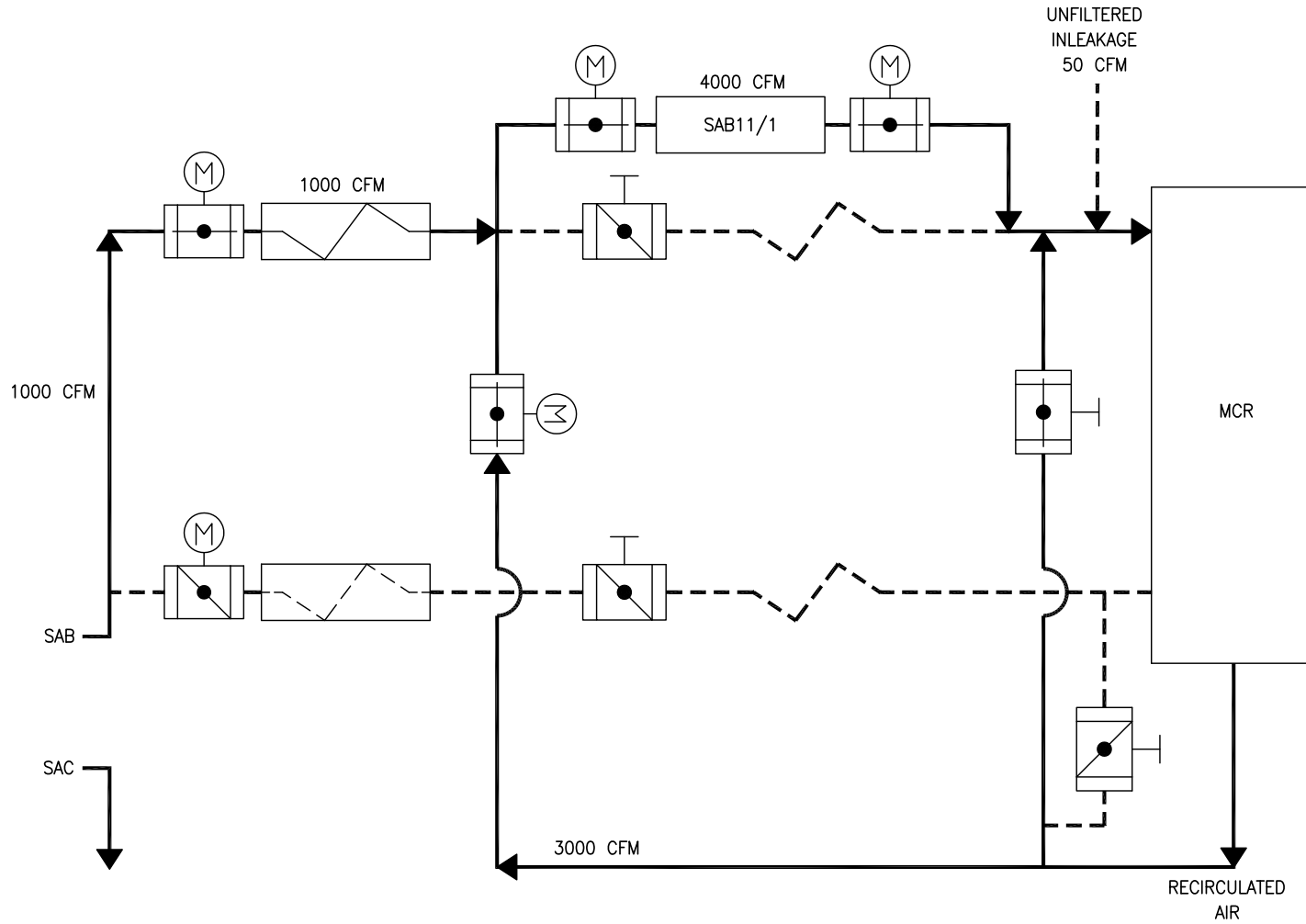
Figure 15.0-4—MCR Envelope Post-Accident HVAC Filtration Mode Model
