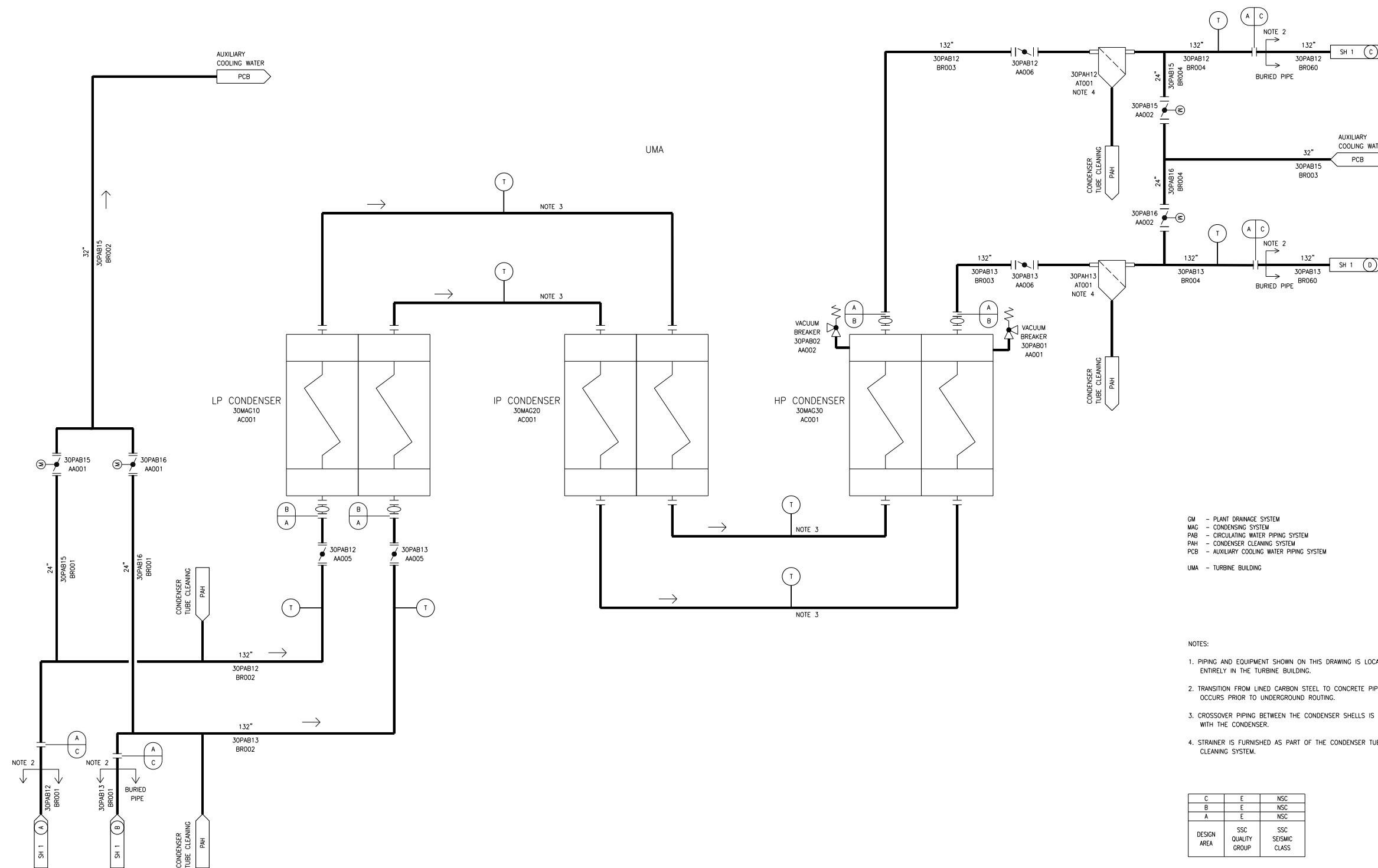
Figure 10.4.5-1—Circulating Water System Flow Diagram Sheet 2 of 2
