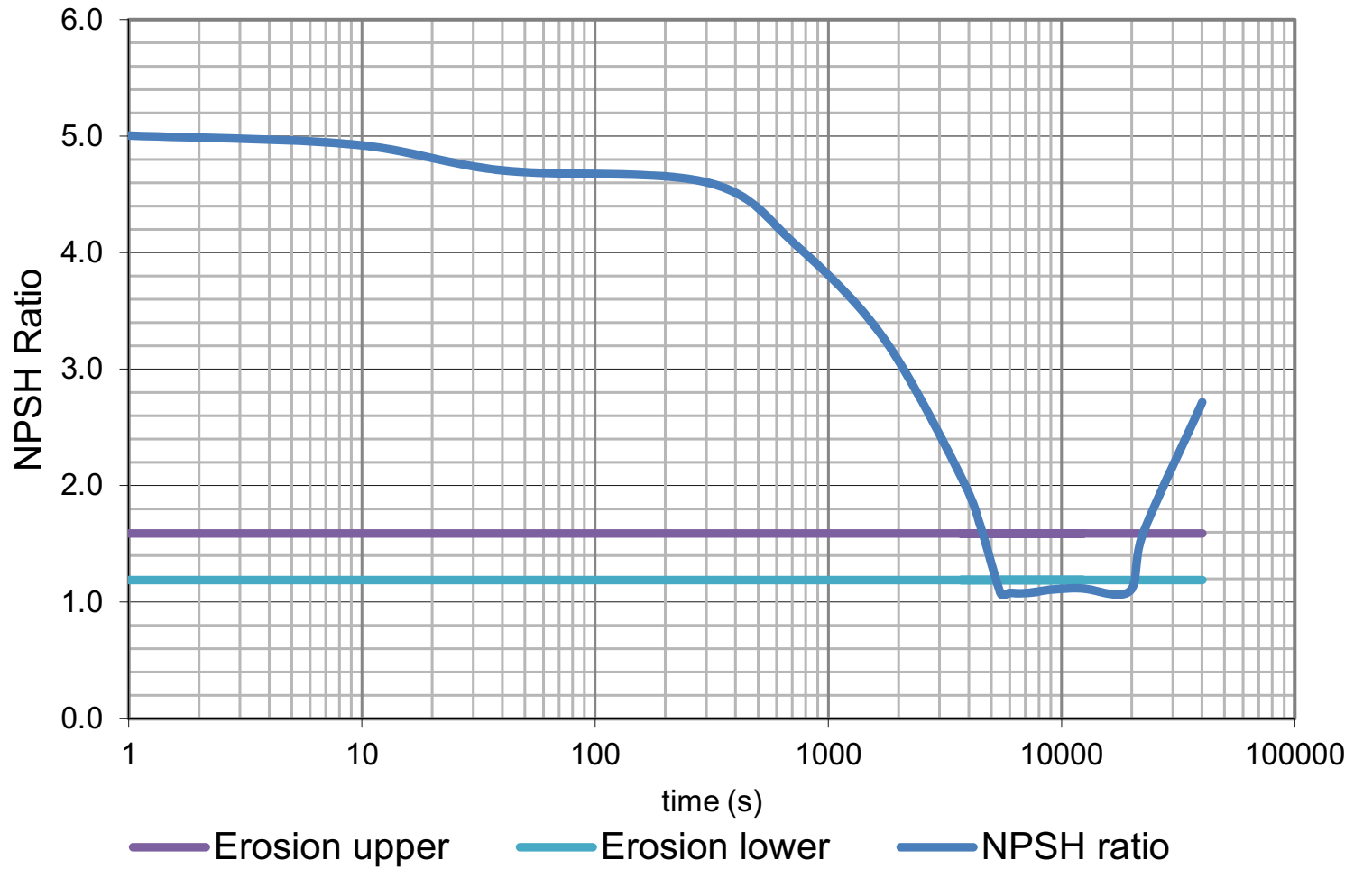
Figure 6.3-10—LHSI in LBLOCA - Cavitation Erosion
