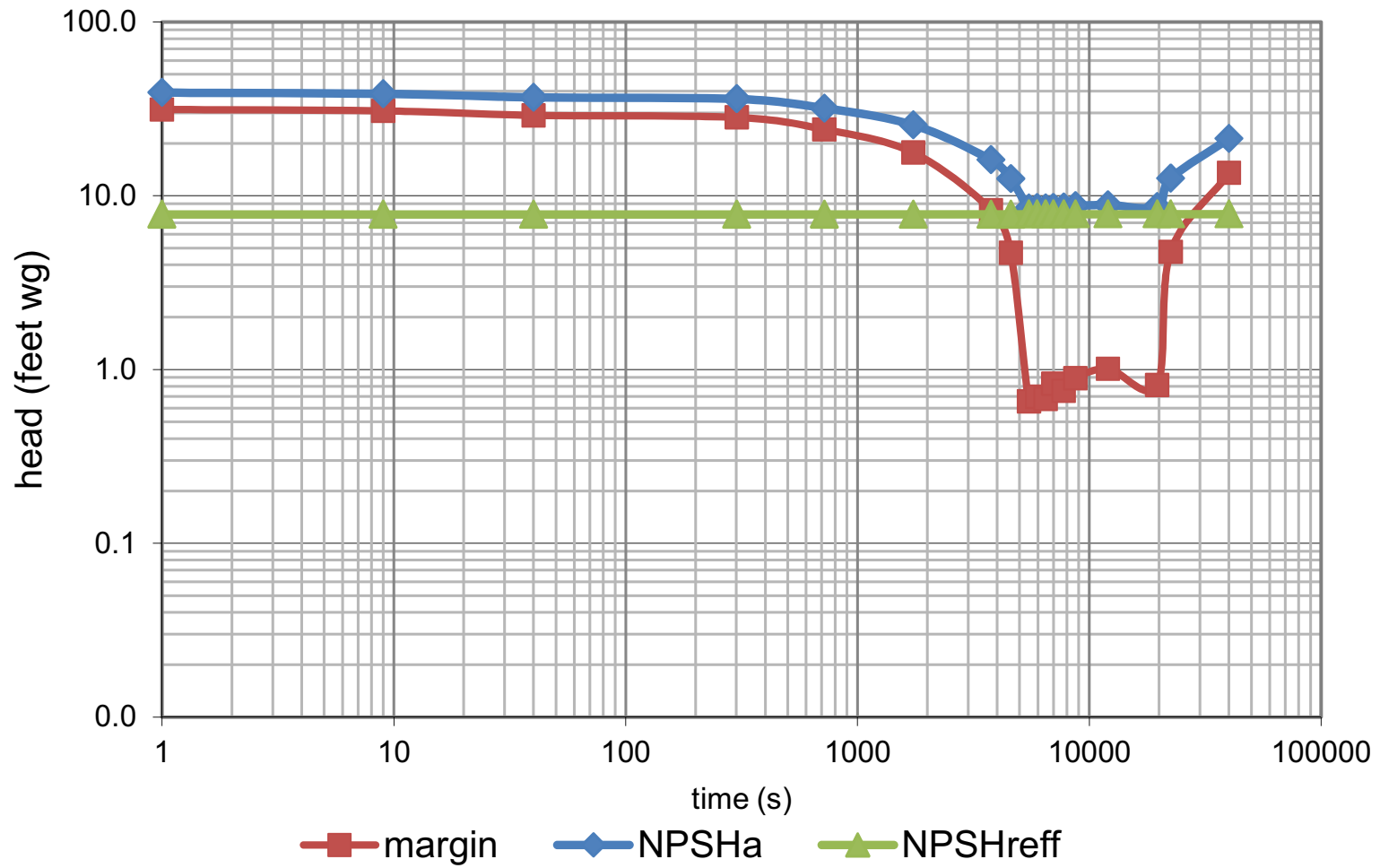
Figure 6.3-8—LHSI in LBLOCA
