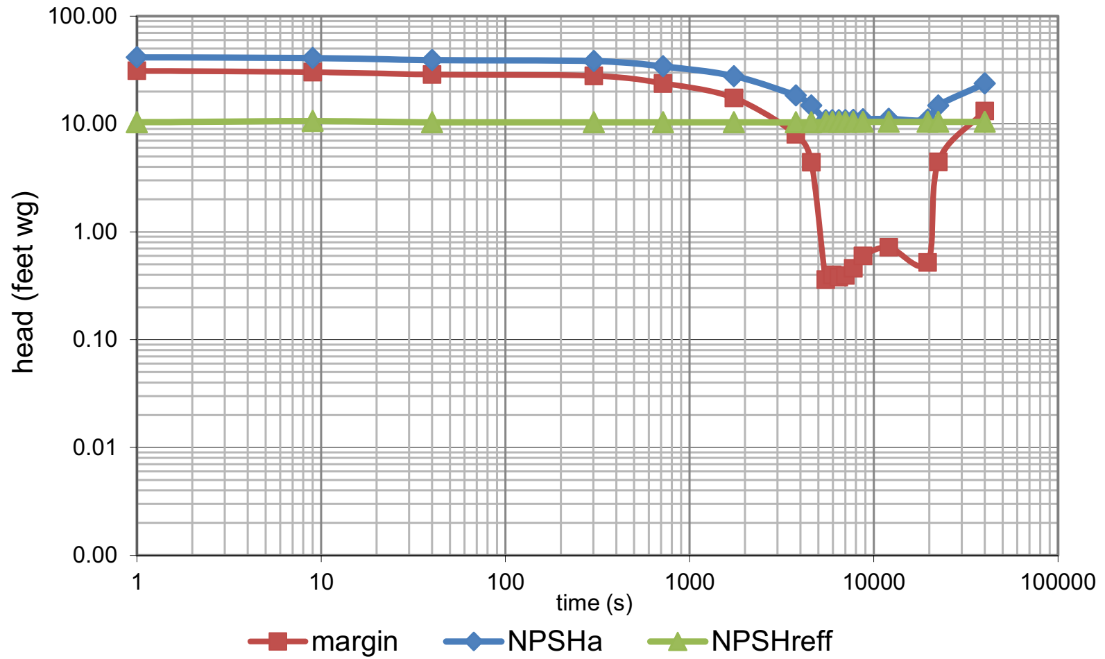
Figure 6.3-9—MHSI in LBLOCA
