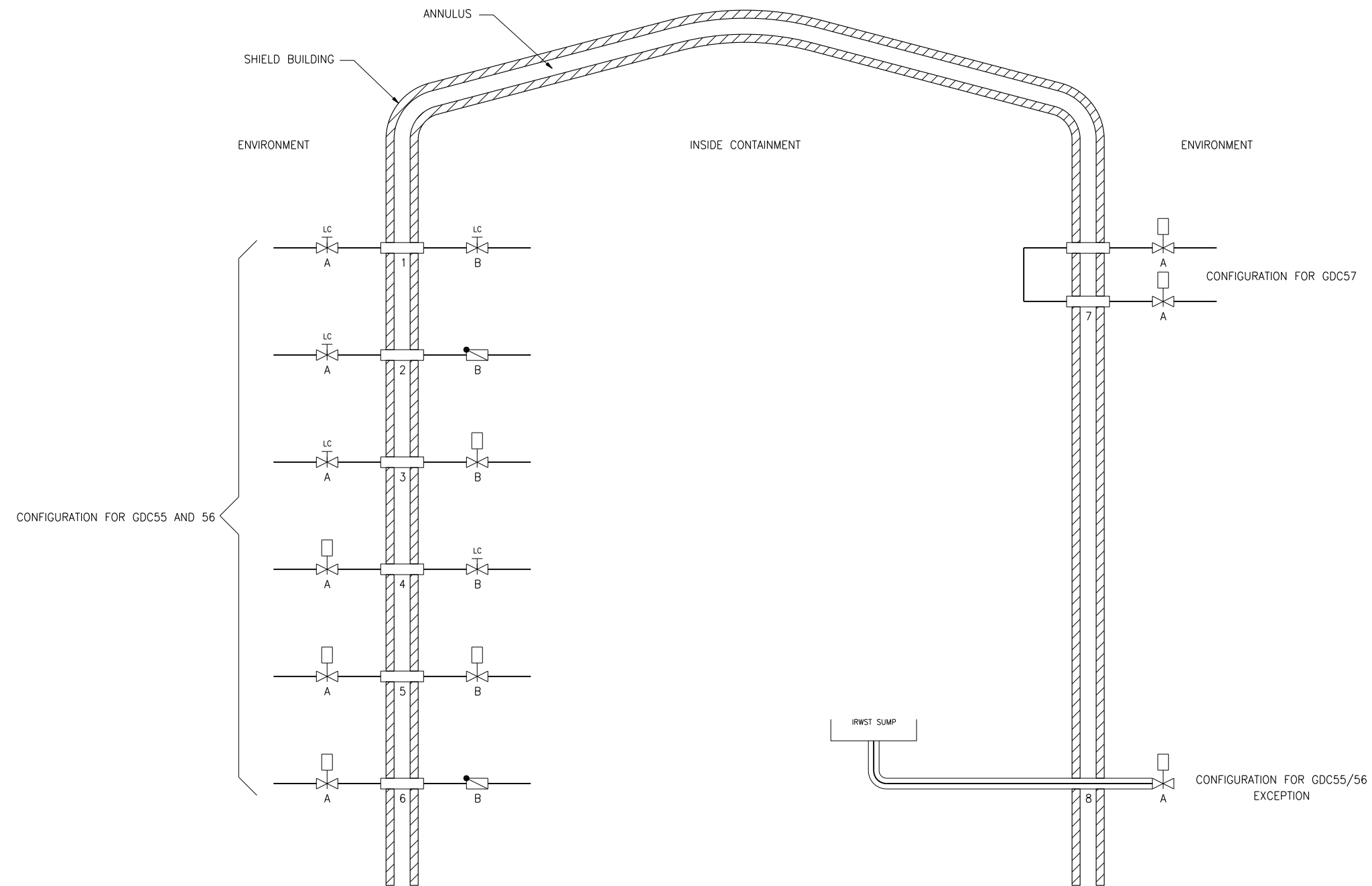
Figure 6.2.4-1—Representative Containment Isolation Valve Arrangement
