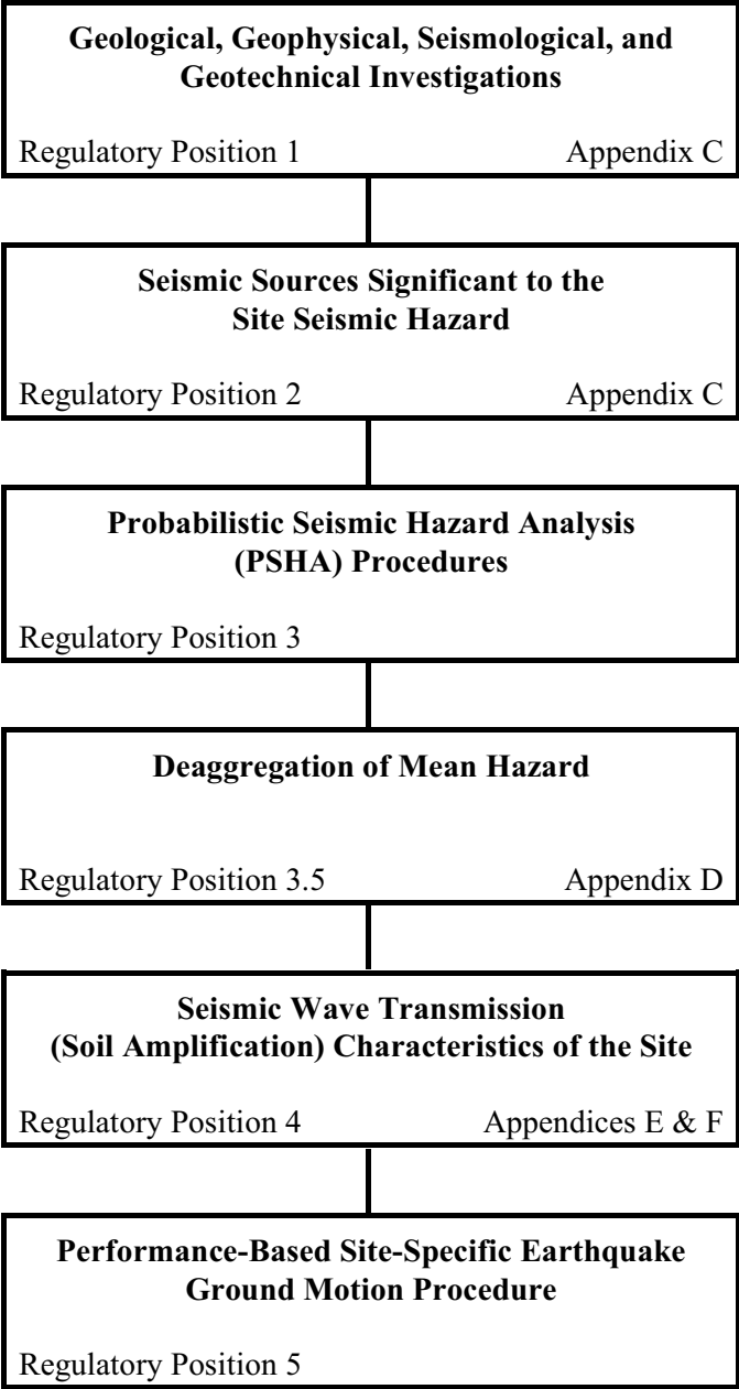
Figure 1. Flow Diagram
