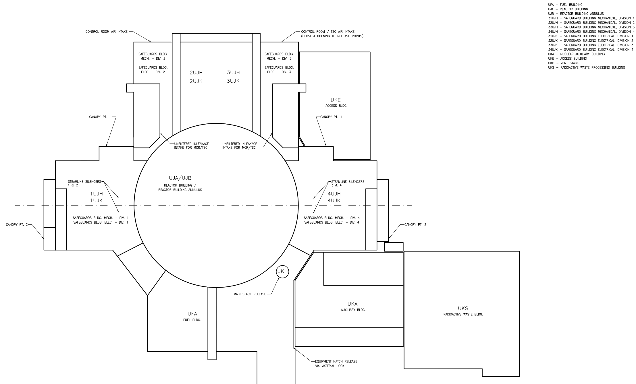
Figure 2.3-1—U.S. EPR Release Points, Control Room Air Intakes, and Unfiltered Inleakage Locations
