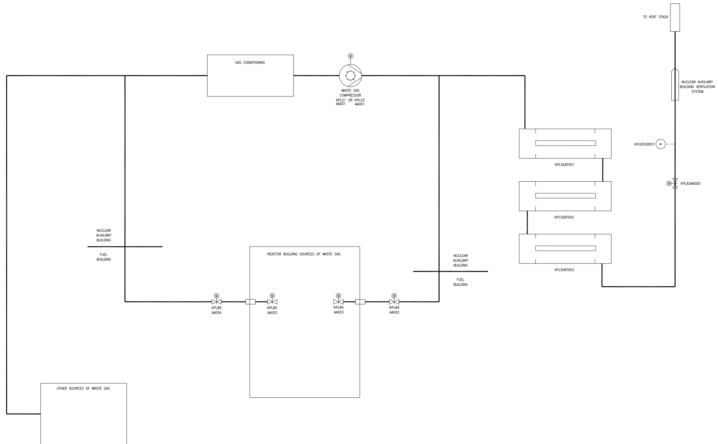
Figure 2.9.3-1—Gaseous Waste Processing System Functional Arrangement
