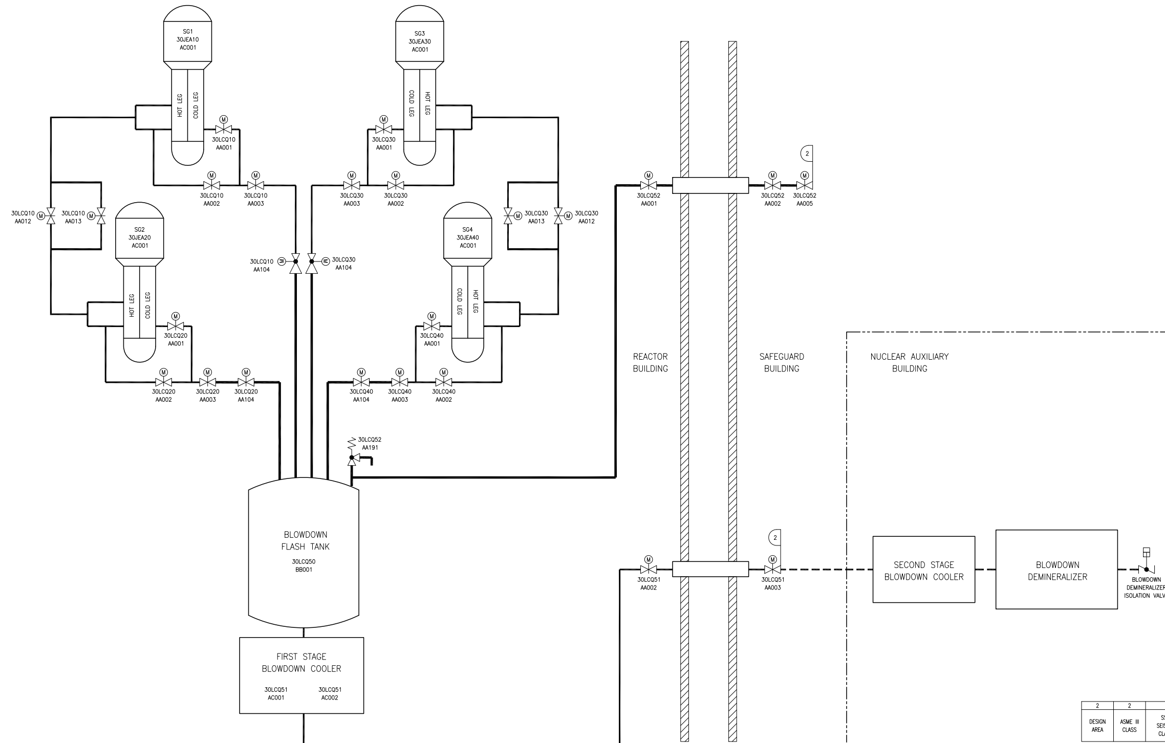
Figure 2.8.7-1—Steam Generator Blowdown System Functional Arrangement
