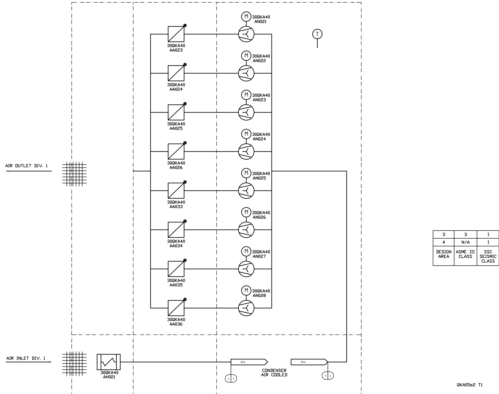
Figure 2.7.2-2—Safety Chilled Water System Air Cooled Division Functional Arrangement Sheet 2 of 2
