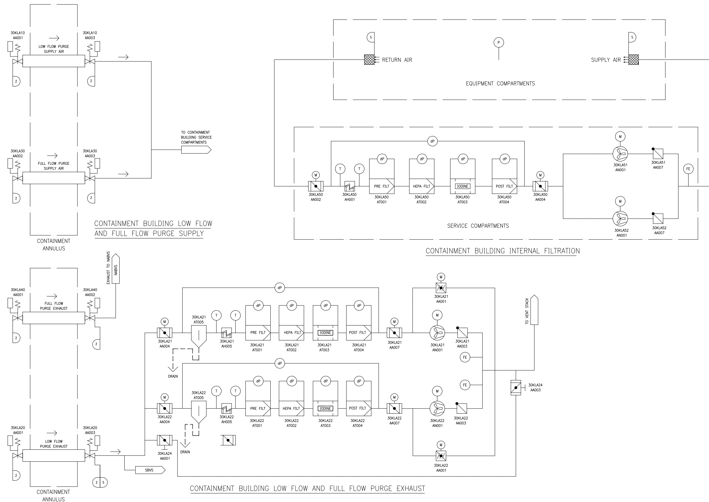
Figure 2.6.8-1—Containment Building Ventilation System Functional Arrangement
