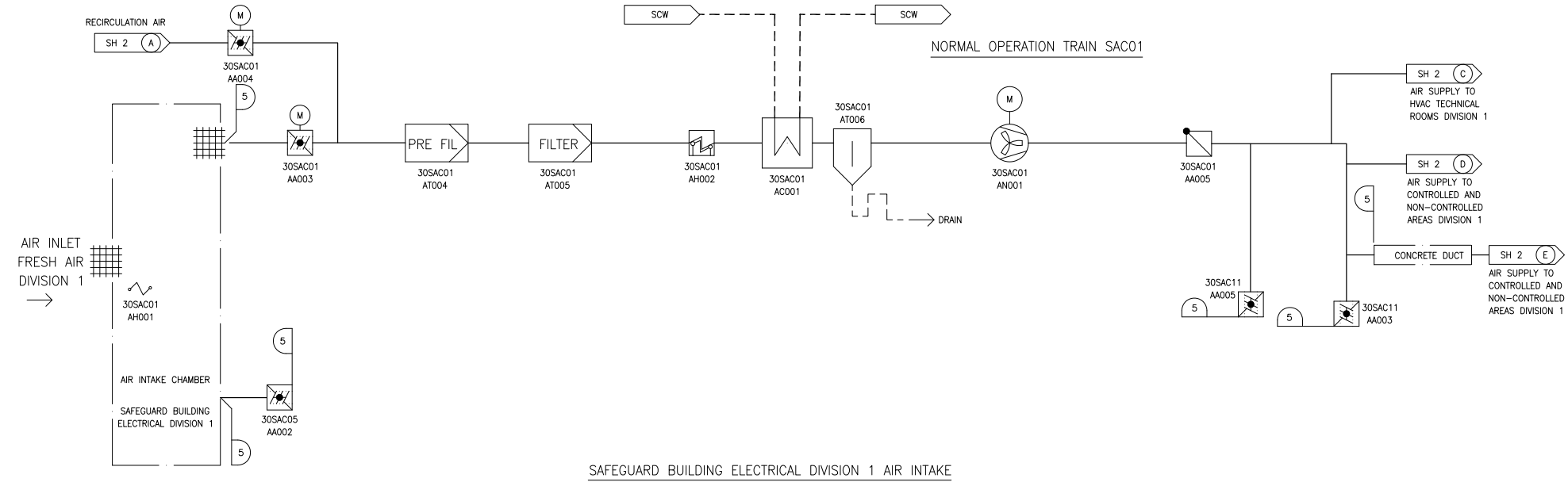
Figure 2.6.7-1—Electrical Division of Safeguard Building Ventilation System Division 1 and Division 4 Air Intake Functional Arrangement
