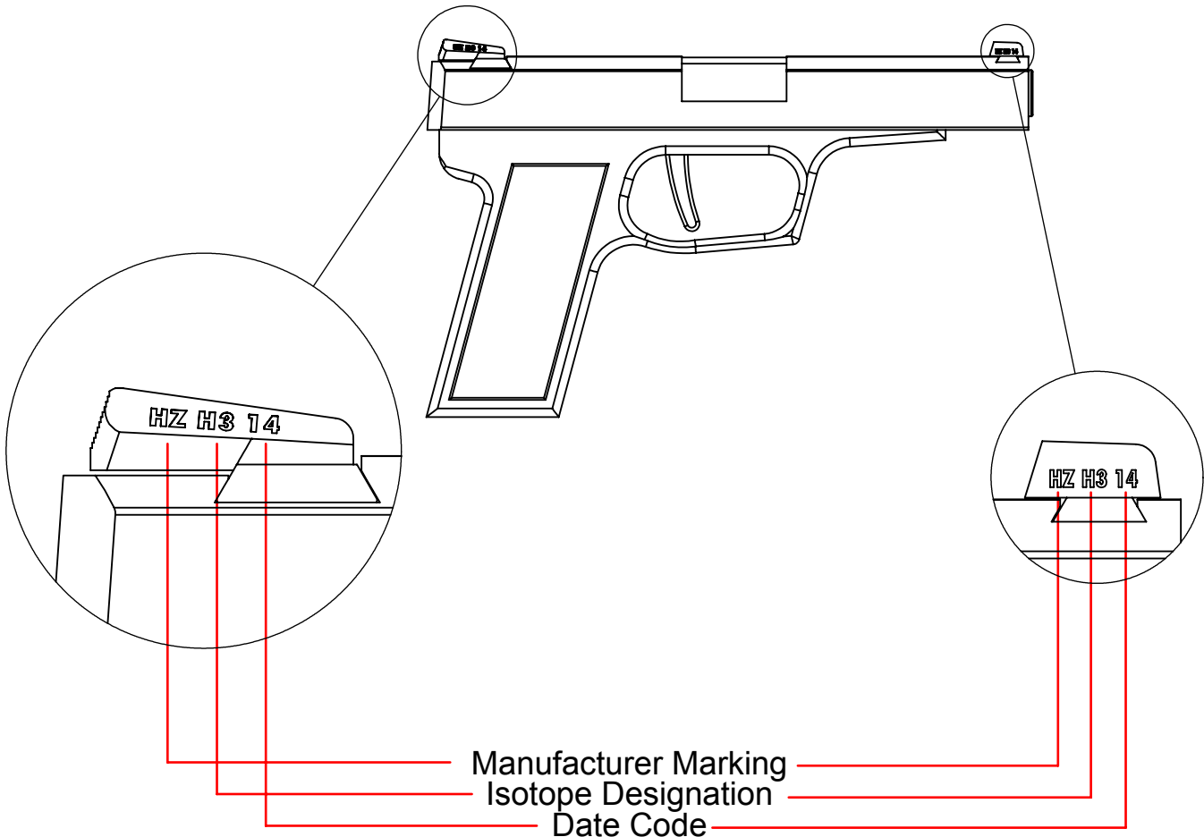
Rear Sight
