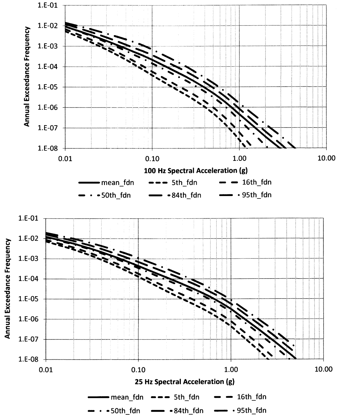
FIGURE C-1 BVPS-2 MEAN AND FRACTILE HAZARD CURVES AT RB FOUNDATION LEVEL (SA AT 100 HZ AND 25 HZ)
