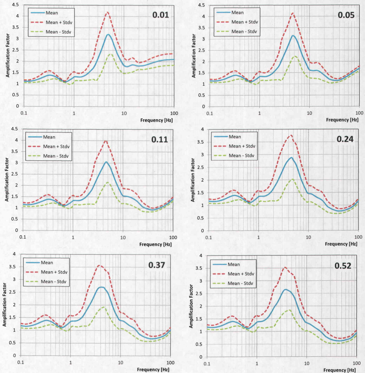
FIGURE 2-4 BVPS-2 SITE AMPLIFICATION FACTORS, BASE-CASE PROFILE (P1), EPRI ROCK G/GMAX AND DAMPING, KAPPA 1, 1-CORNER SOURCE MODEL
