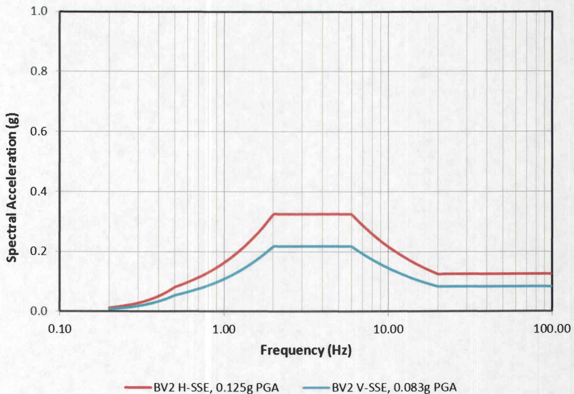
FIGURE 3-1 BVPS-2 SAFE SHUTDOWN EARTHQUAKE 5%-DAMPED RESPONSE SPECTRA
