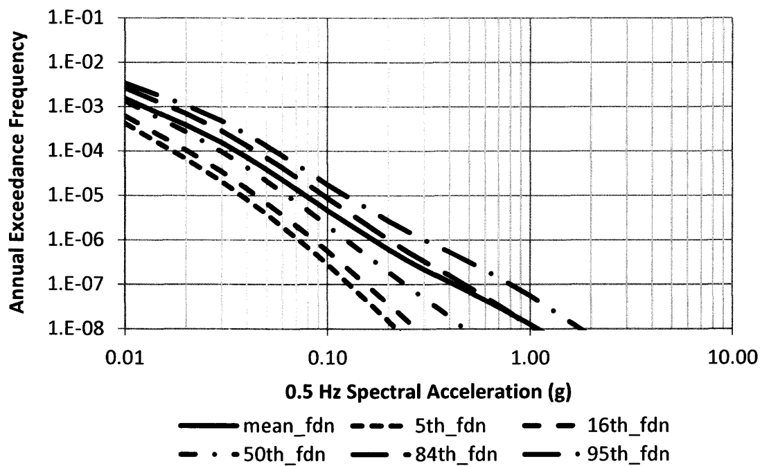
FIGURE C-4 BVPS-2 MEAN AND FRACTILE HAZARD CURVES AT RB FOUNDATION LEVEL (SA AT 0.5 HZ)
