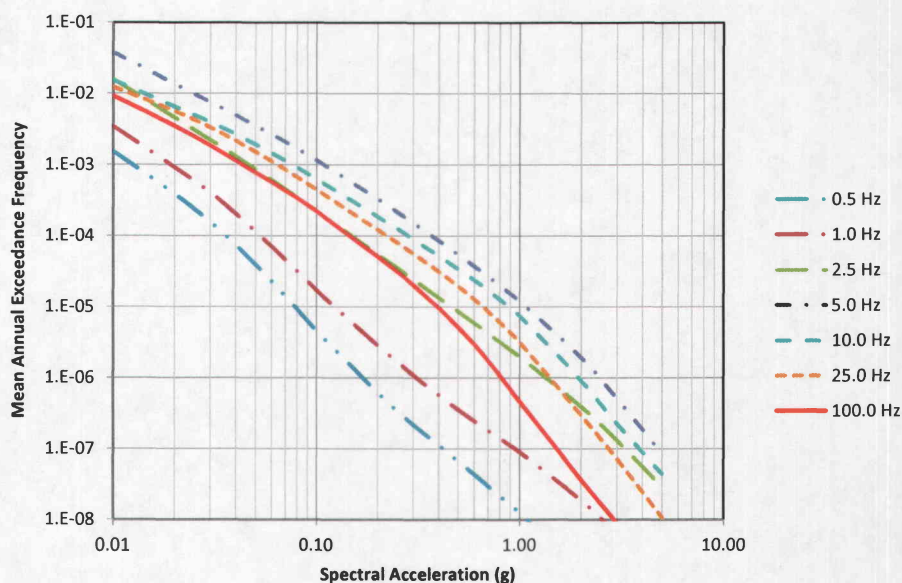
FIGURE 2-6 BVPS-2 MEAN CONTROL POINT SEISMIC HAZARD AT SELECTED SPECTRAL FREQUENCIES
