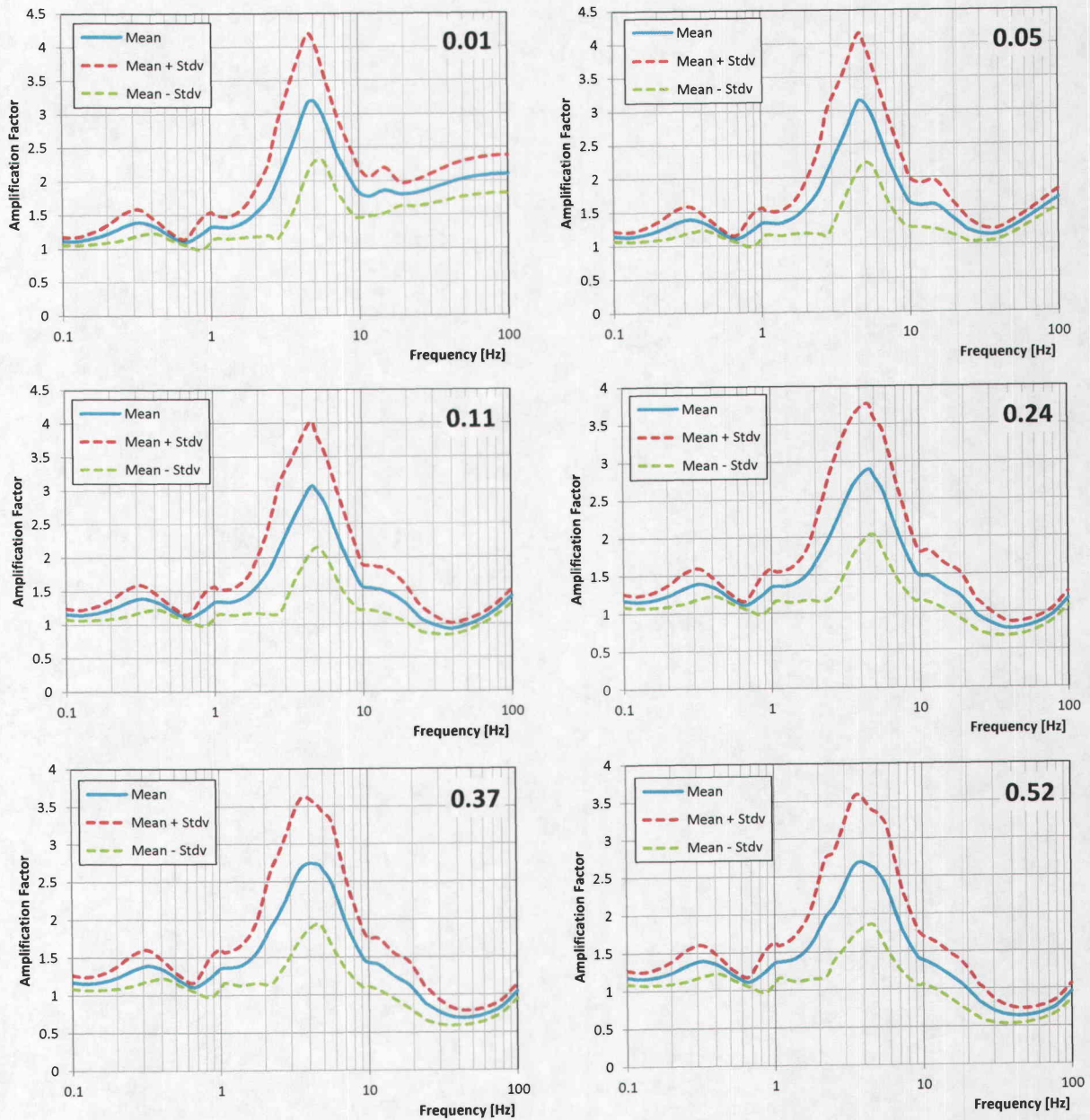
FIGURE 2-5 BVPS-2 SITE AMPLIFICATION FACTORS, BASE-CASE PROFILE (P1), LINEAR ROCK G/GMAX AND DAMPING, KAPPA 1, 1-CORNER SOURCE MODEL
