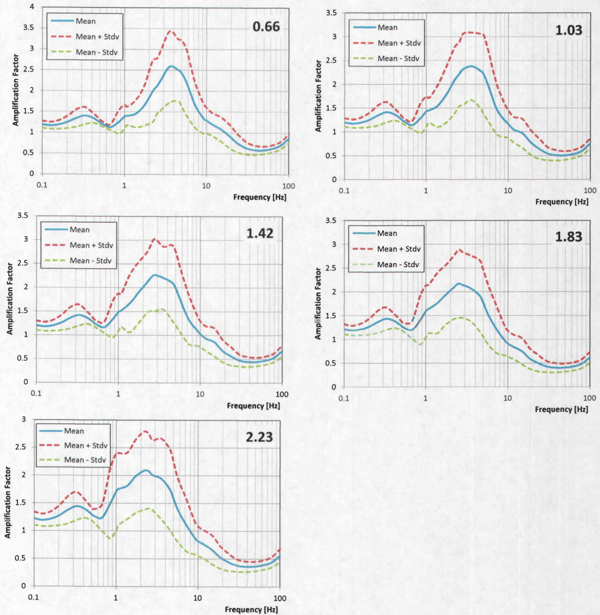
FIGURE 2-4 (CONTINUED) BVPS-2 SITE AMPLIFICATION FACTORS, BASE-CASE PROFILE (P1), EPRI ROCK G/GMAX AND DAMPING, KAPPA 1, 1-CORNER SOURCE MODEL
