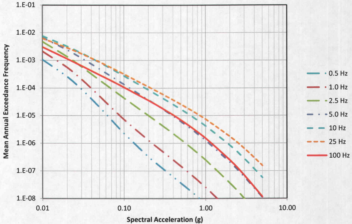
FIGURE 2-1 BVPS-2 MEAN SEISMIC HAZARD AT HARD ROCK
