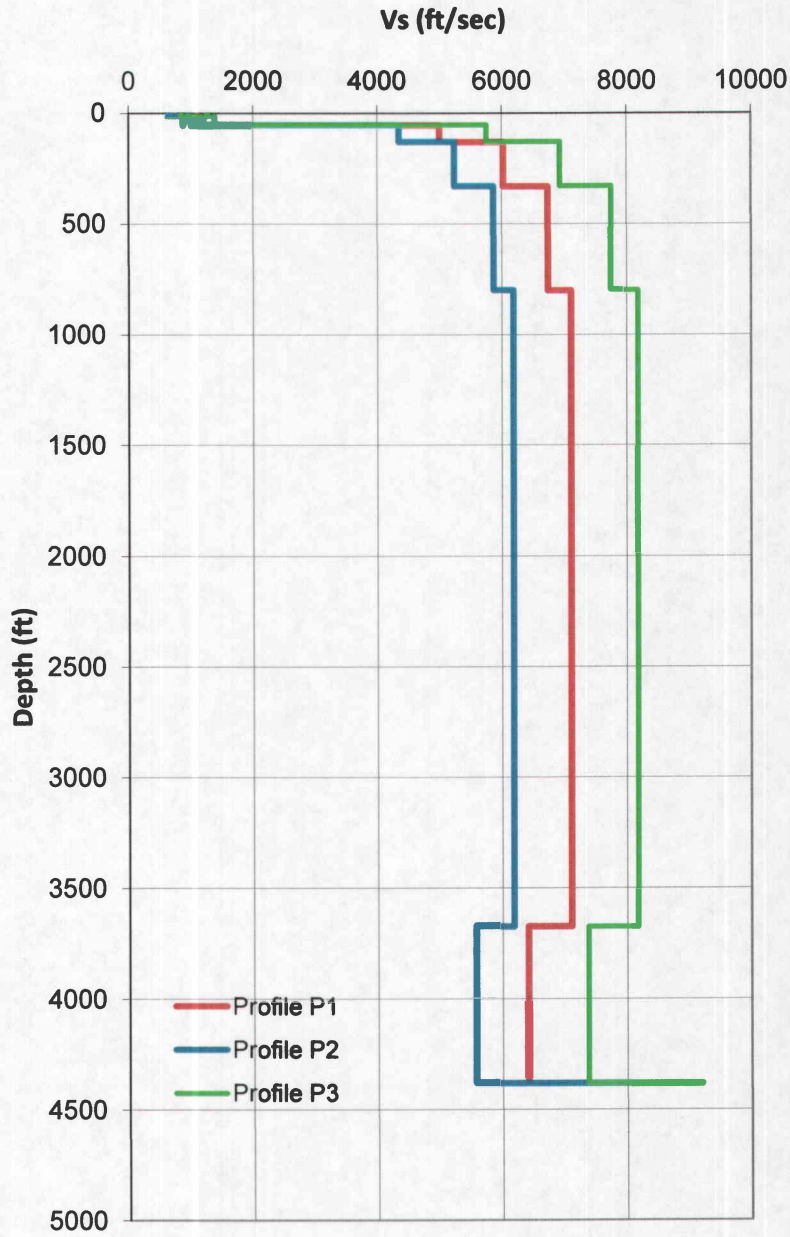
FIGURE 2-3 BASE CASE V_s PROFILES, BVPS-2 SITE
