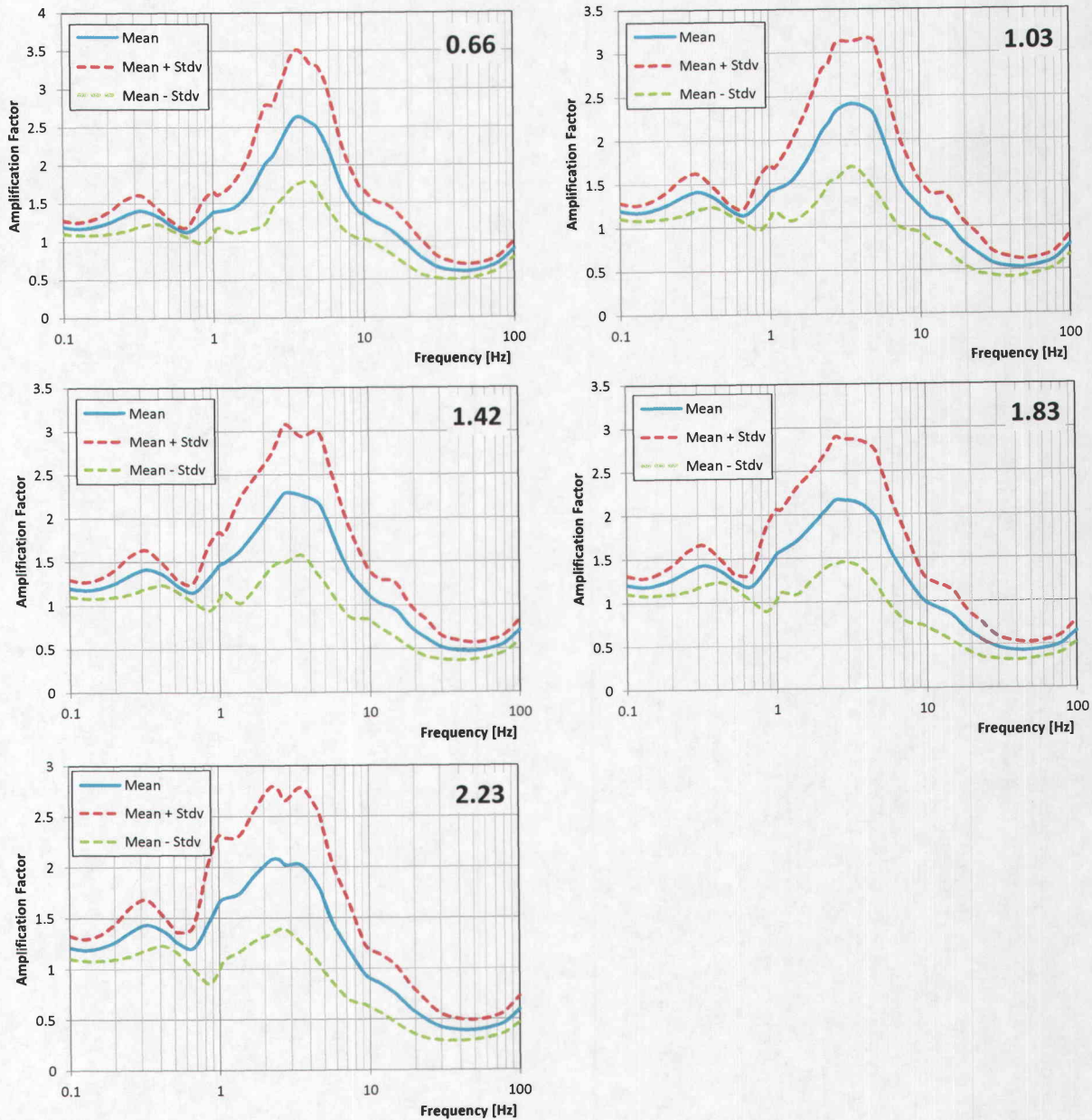
FIGURE 2-5 (CONTINUED) BVPS-2 SITE AMPLIFICATION FACTORS, BASE-CASE PROFILE (P1), LINEAR ROCK G/GMAX AND DAMPING, KAPPA 1, 1-CORNER SOURCE MODEL
