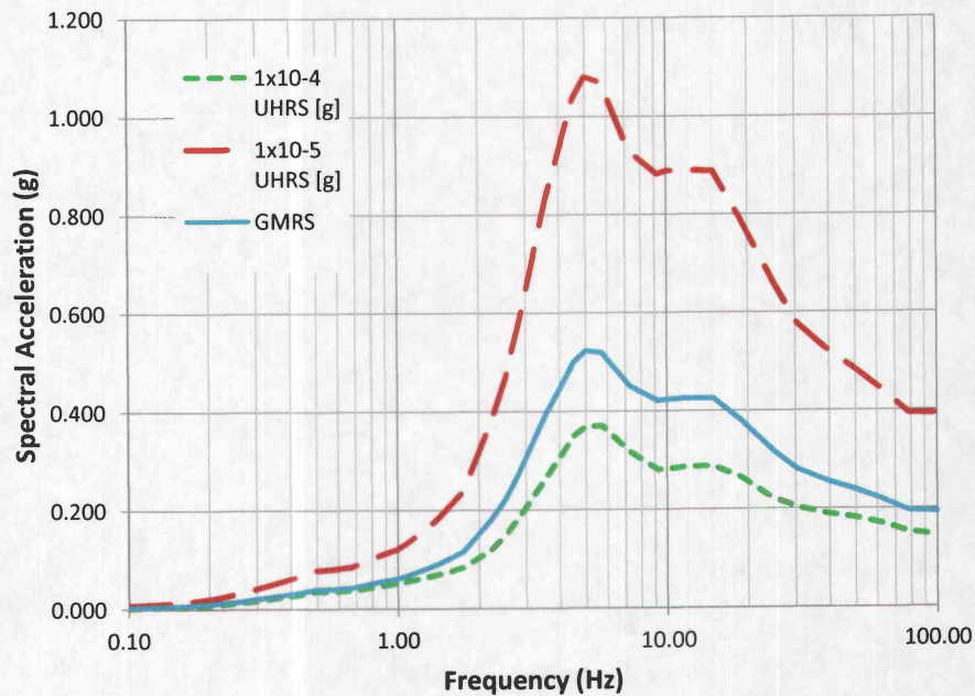
FIGURE 2-7 CONTROL POINT UNIFORM HAZARD RESPONSE SPECTRA AT MEAN ANNUAL FREQUENCIES OF EXCEEDANCE OF 1X10-4 AND 1X10-5, AND GROUND MOTION RESPONSE SPECTRUM AT BVPS-2
