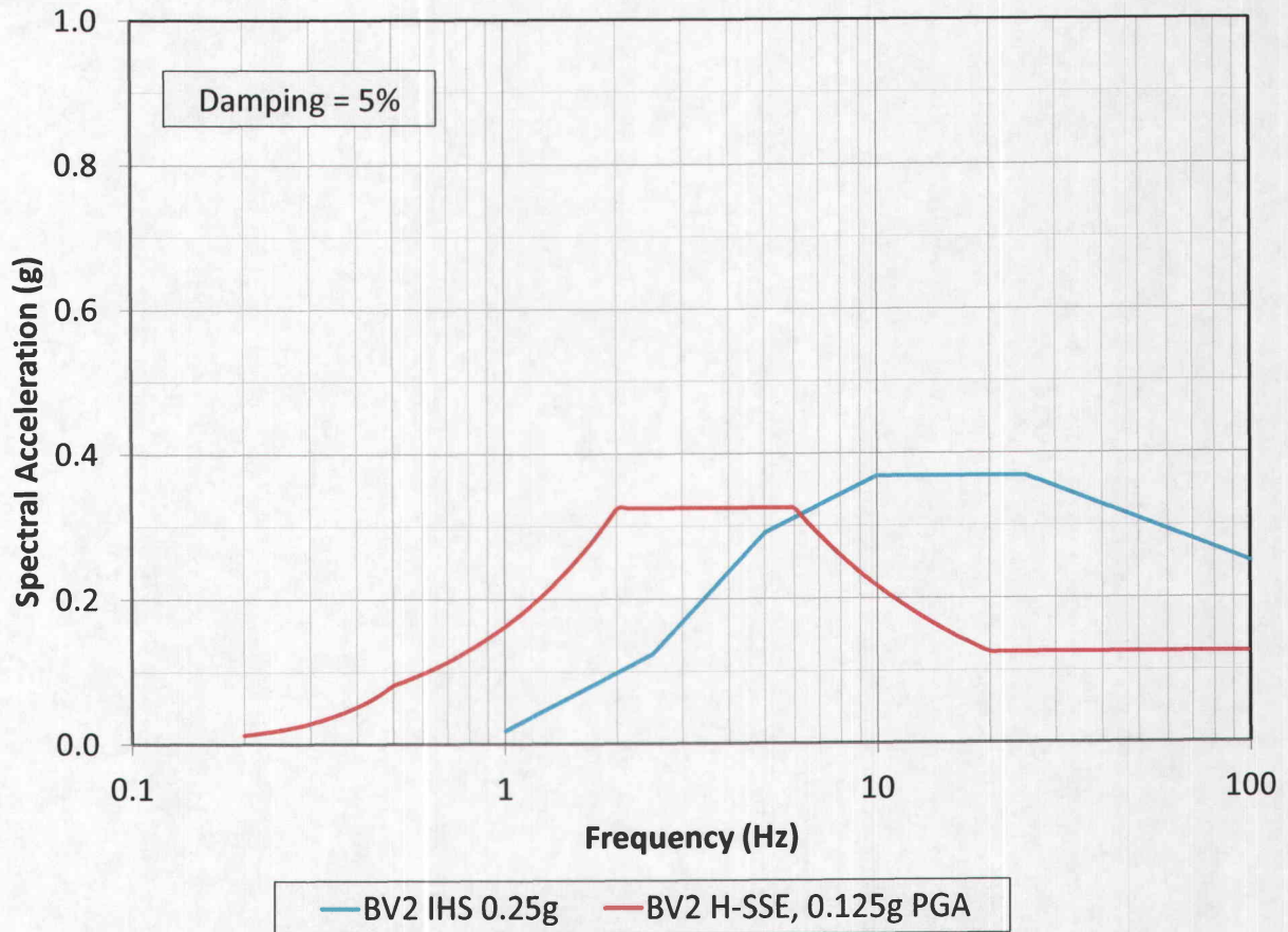
FIGURE 5-1 BVPS-2 SSE AND IPEEE HCLPF SPECTRA
