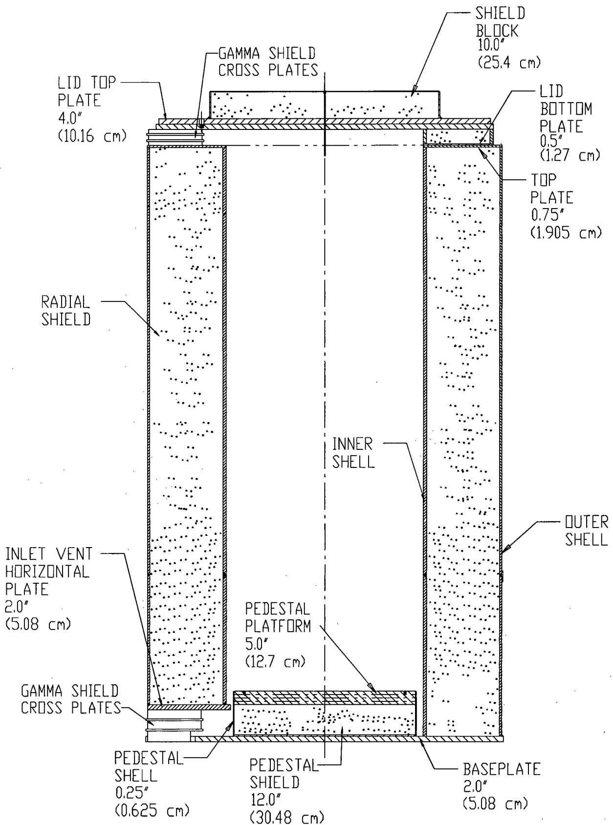
FIGURE 5.3.18; HI-STORM 100S OVERPACK CROSS SECTIONAL ELEVATION VIEW
