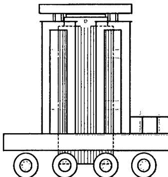
Figure 8.1.29b; Sample HI-TRAC Transfer Options (HI-TRAC 100/125 Shown)
