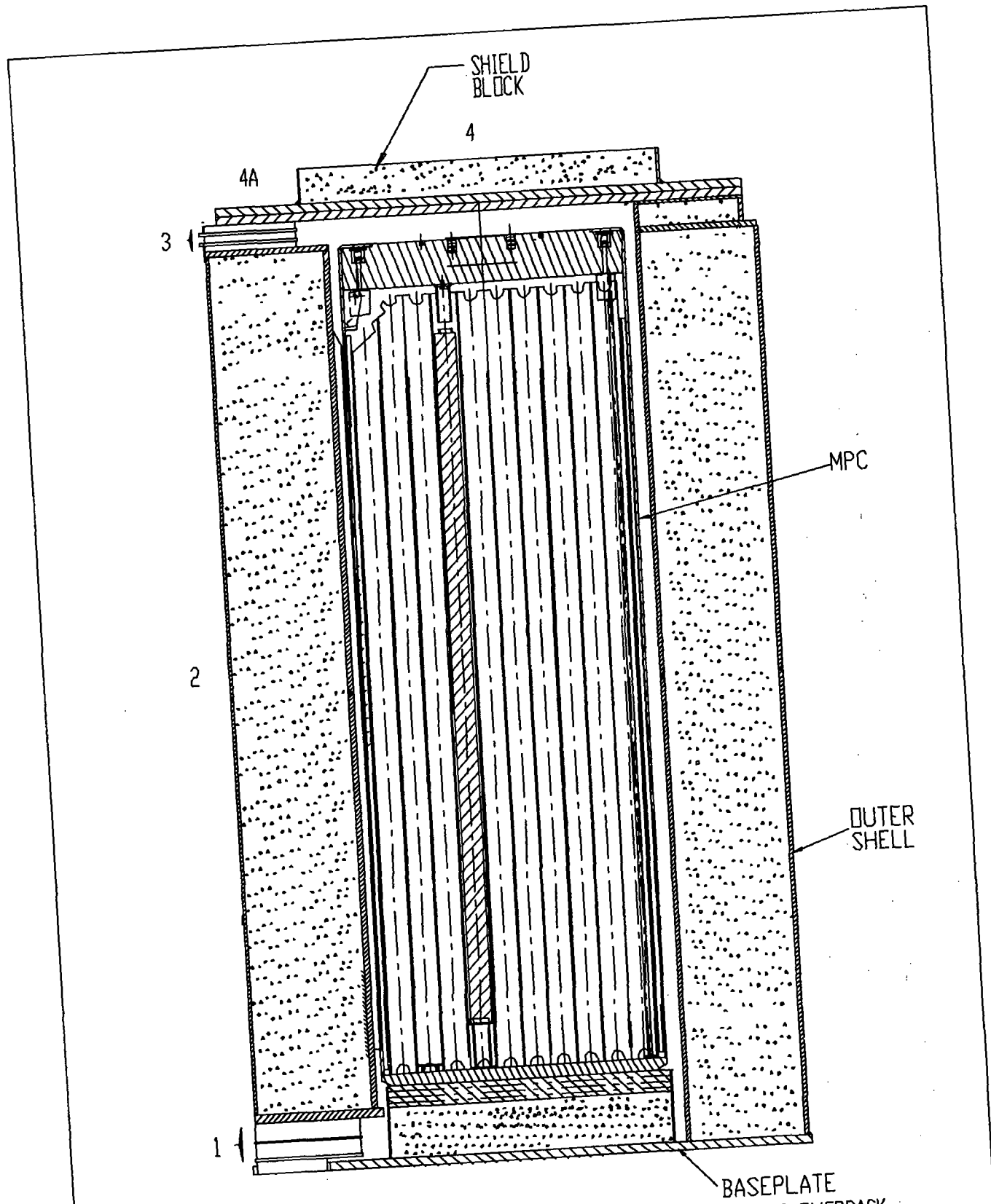
FIGURE 5.1.12; CROSS SECTION ELEVATION VIEW OF THE HI-STORM 100S OVERPACK WITH DOSE POINT LOCATION
