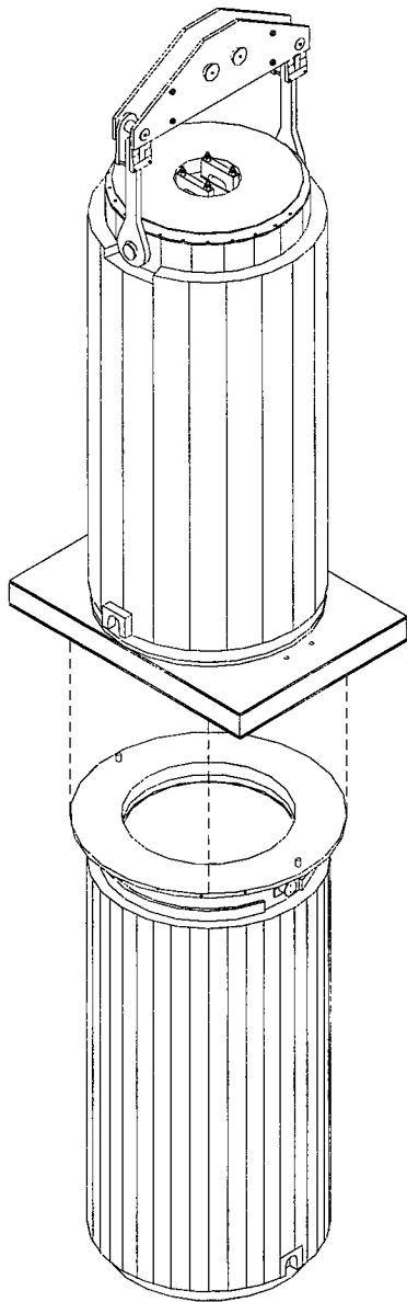
HI-TRAC 100 / 125
