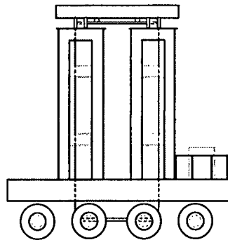
Figure 8.1.29a; Sample HI-STORM Transfer Options
