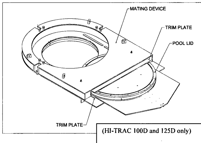
Figure 8.1.33; Trim Plate Locations
