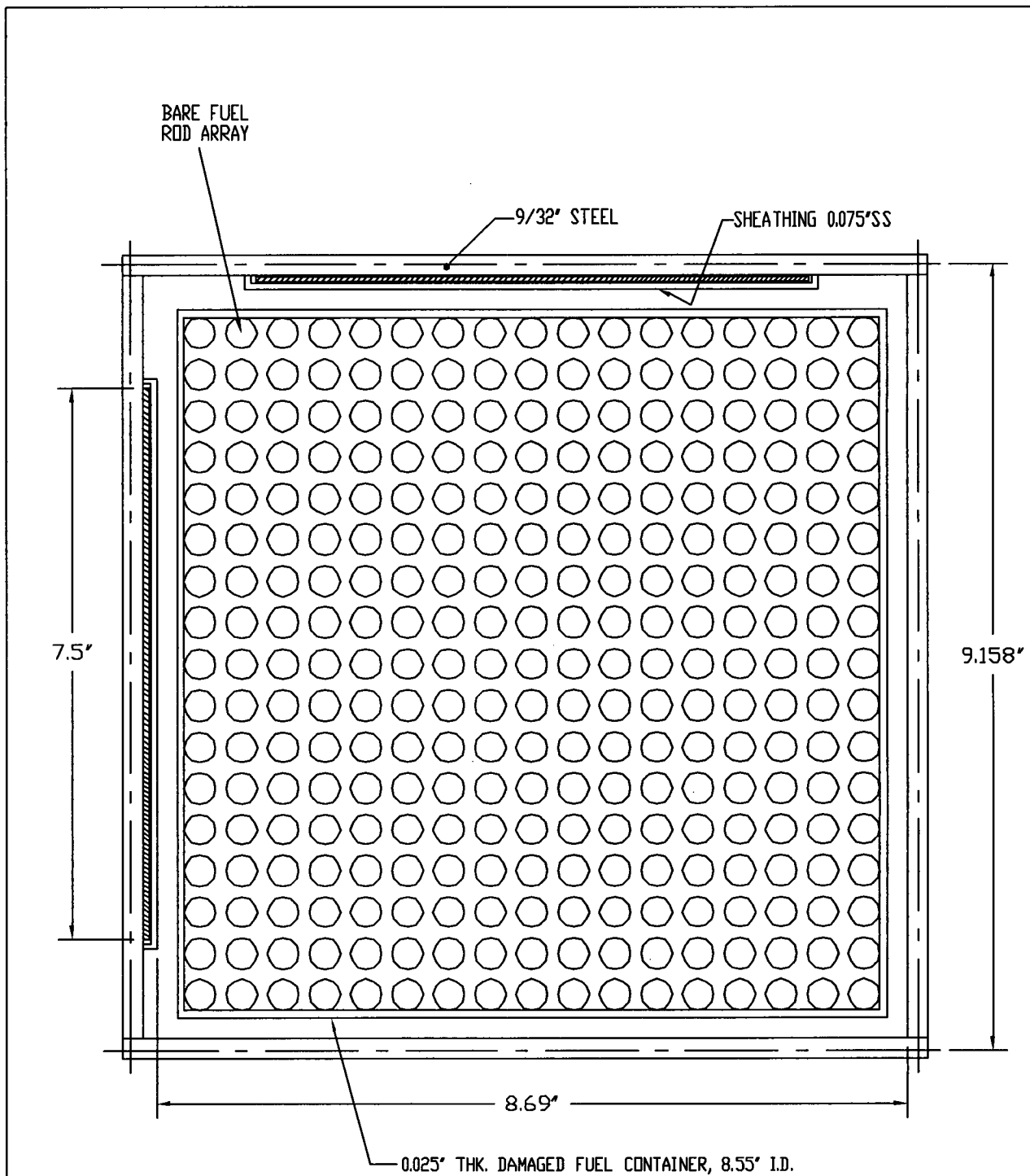
FIGURE 6.4.17; DAMAGED FUEL/FUEL DERIS CALCULATION MODEL (PLANAR CROSS-SECTION) WITH BARE FUEL RODS IN THE MPC-32 BASKET ( SEE CHAPTER 1 FOR TRUE BASKET DIMENSIONS )
