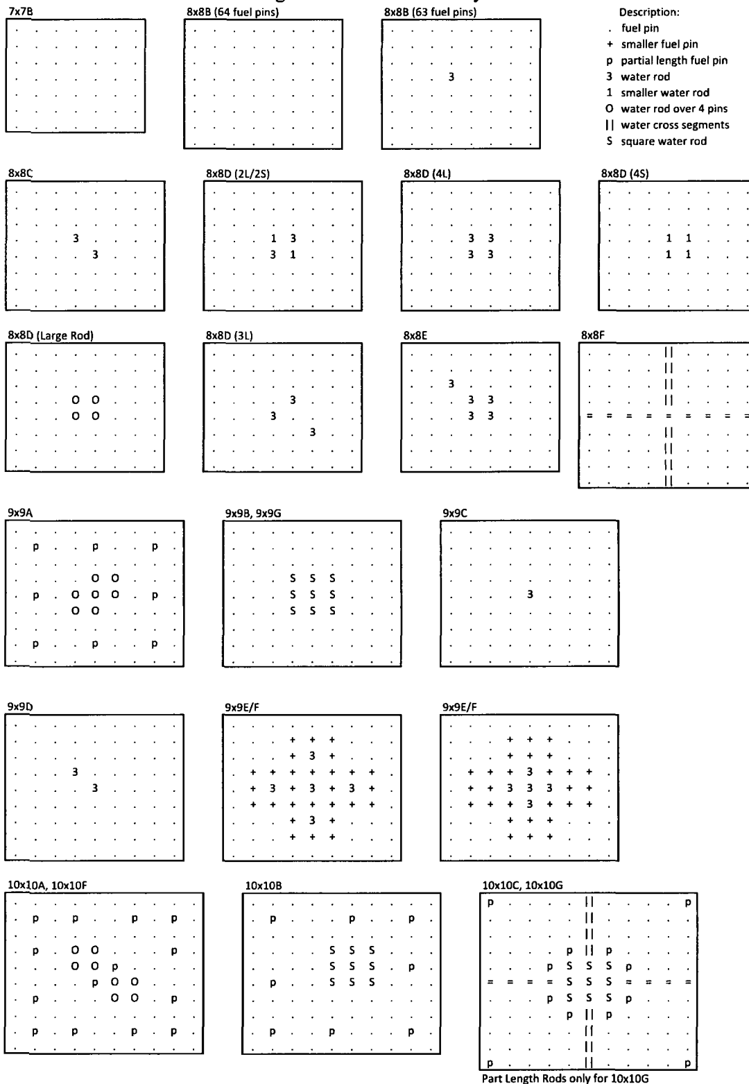
Figure 6.III.4.1 Assembly Cross Sections
