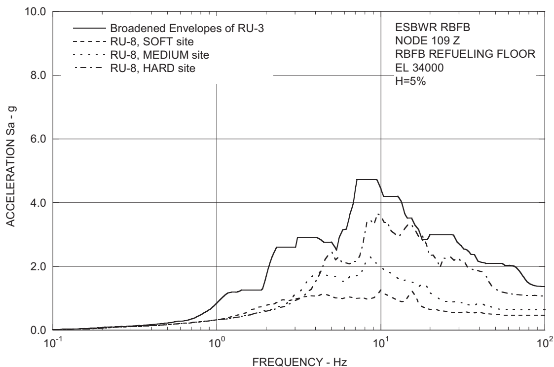
Figure 3.8-94(28) FRS (Compared with the DAC3N) – RBFB Refueling Floor Z
