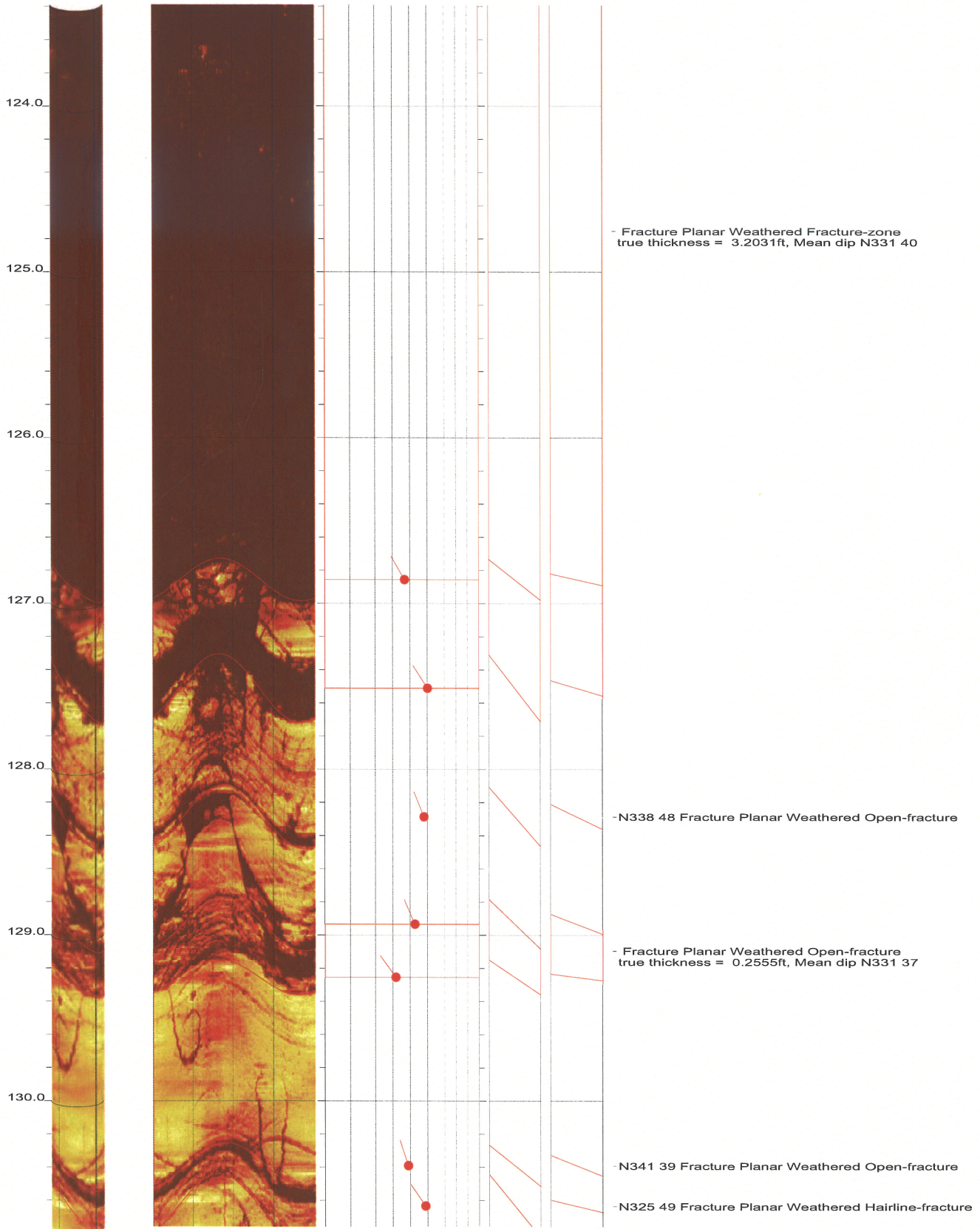
North Anna COL Boring B-901 Acoustic Televiewer Dips Sheet 13 of 36
