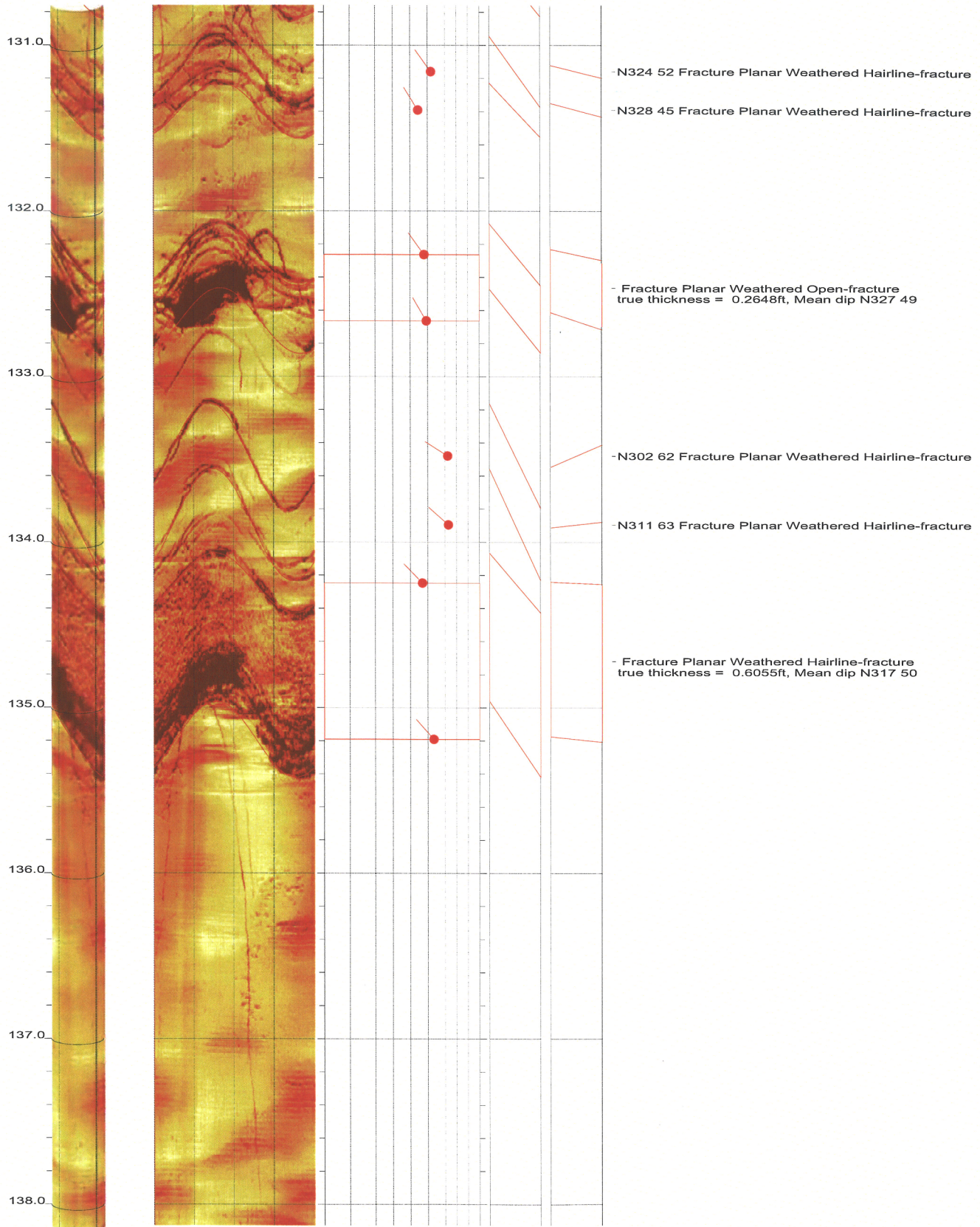
North Anna COL Boring B-901 Acoustic Televiwer Dips Sheet 14 of 36
