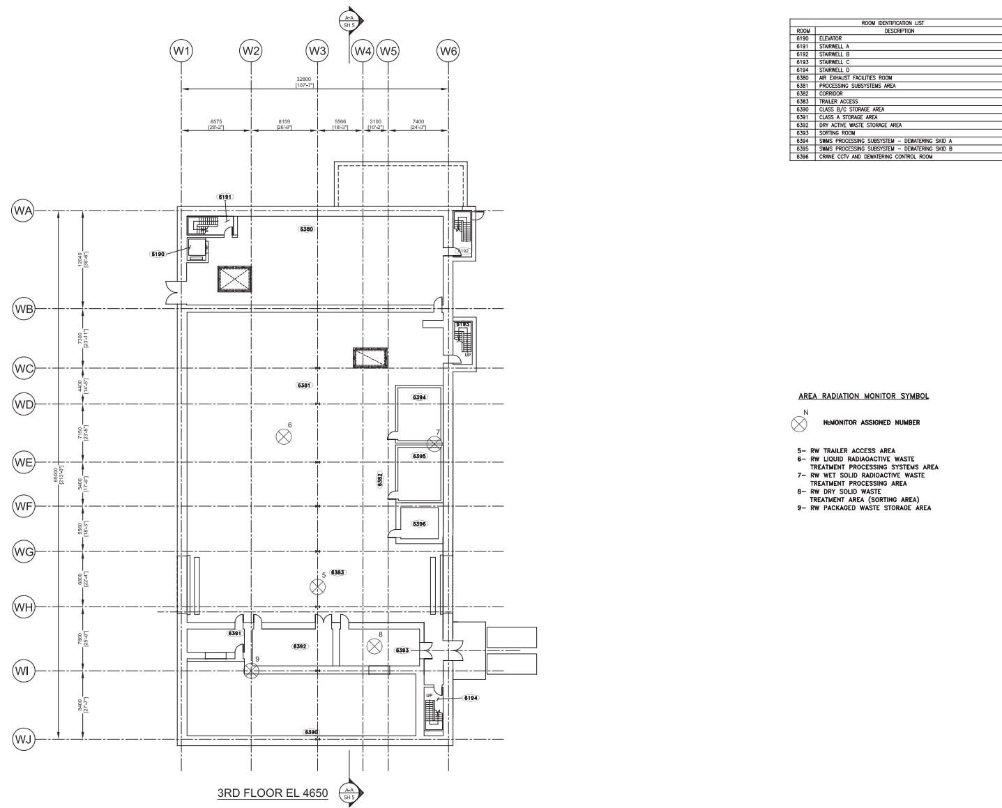
NAPS DEP 11.4-1 Figure 12.3-41R Radwaste Building Radiation Monitors EL 4650
