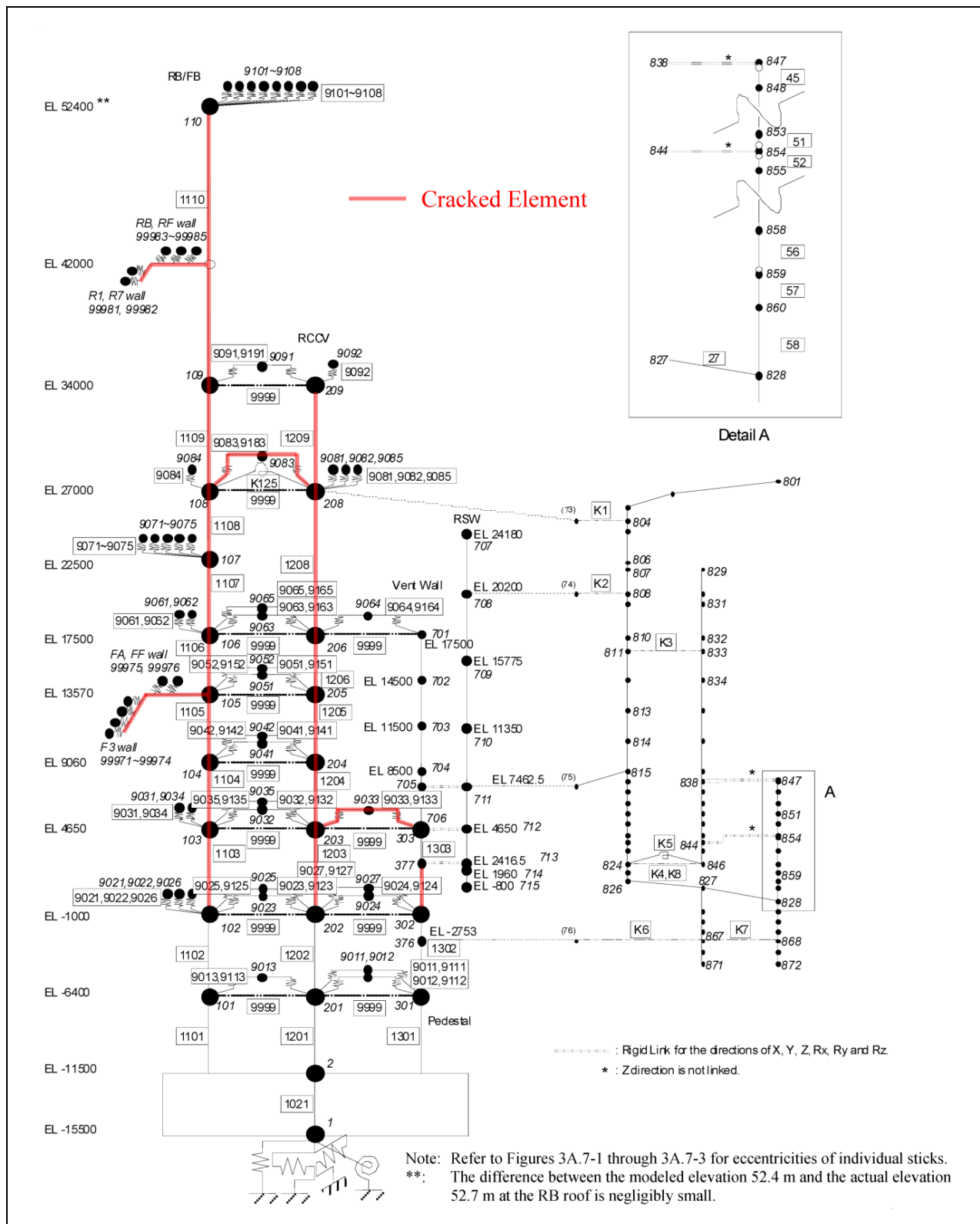
Figure 3.7.2-210 RB/FB Complex Seismic Model with Cracked Elements
