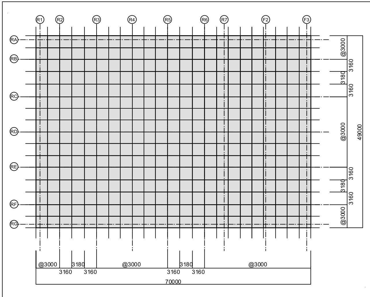
Figure 3.7.2-201 SASSI2010 Plate Elements for RB/FB Basemat
