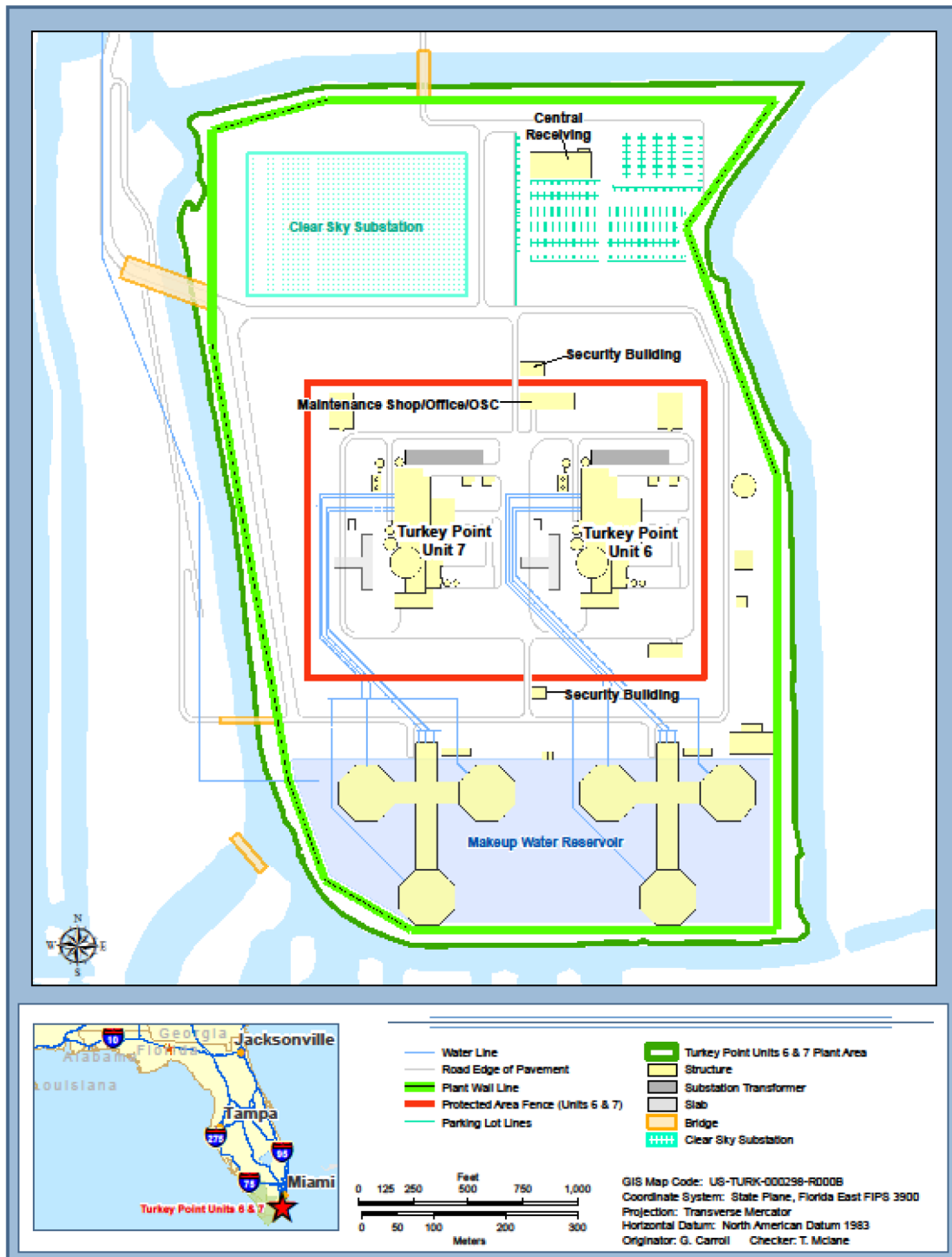
Figure C1-1 Units 6 &amp; 7 Facility Layout
