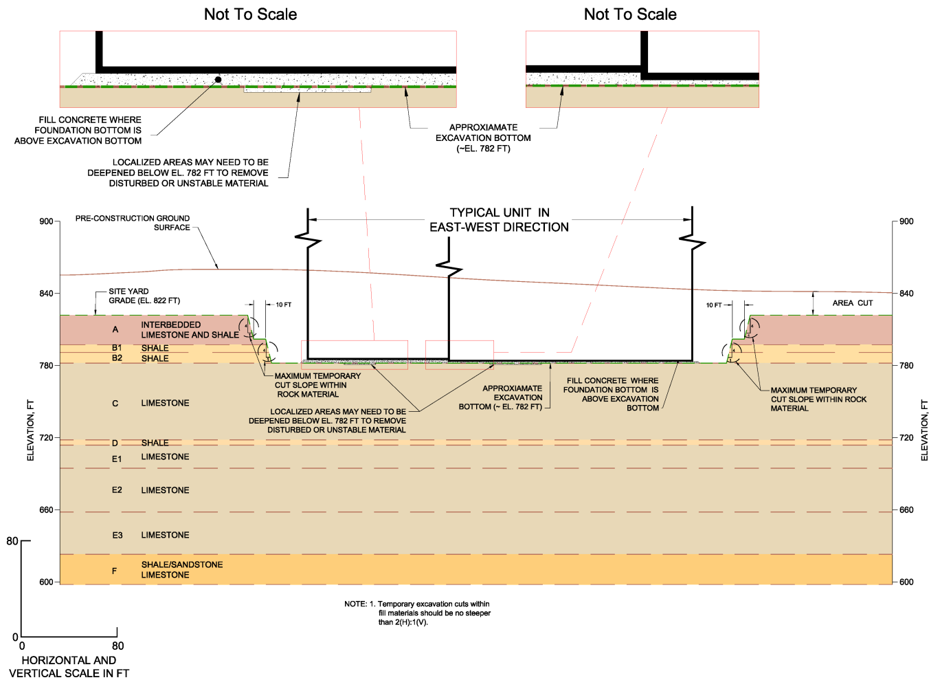
Figure 2.5.4-217 General Excavation Profile
