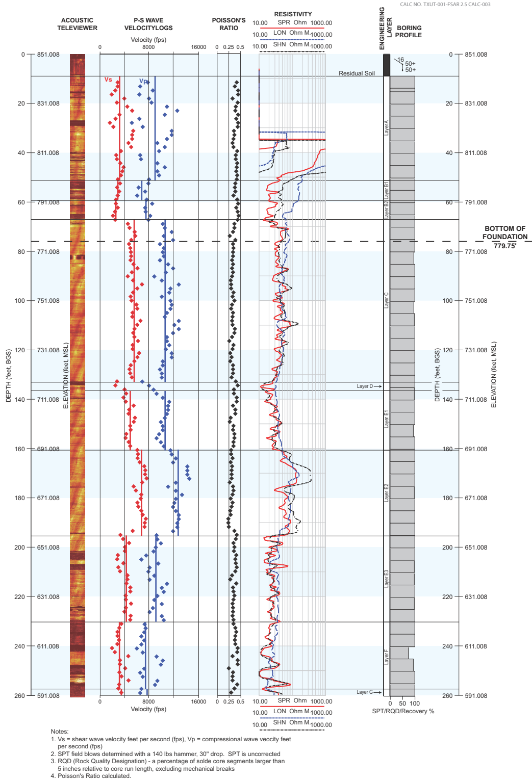
Figure 2.5.4-206 Boring In Situ Test Summary Log, B-1000 (Sheet 1 of 2)
