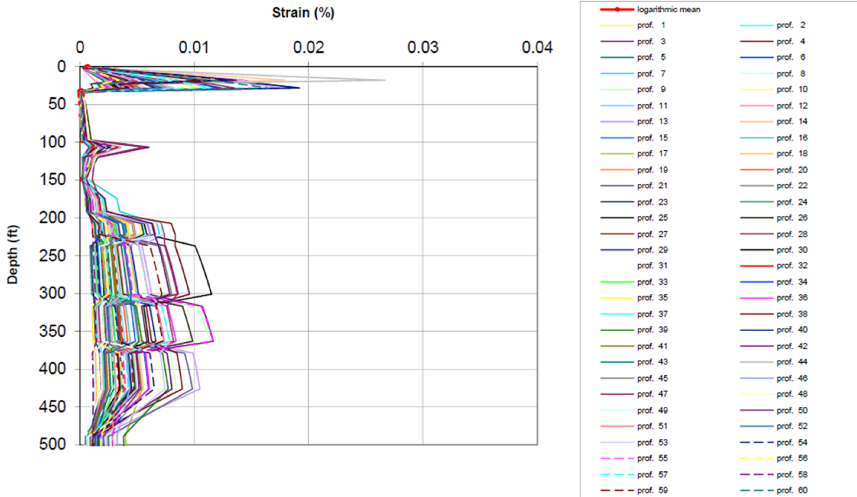
Figure 2.5.2-252 Maximum Shear Strain for the upper 500 feet below Elevation 822 ft of FIRS4_SCSR (Full Site Column Corresponding to FIRS4) for 10^{-4} Broad-Band Spectra
