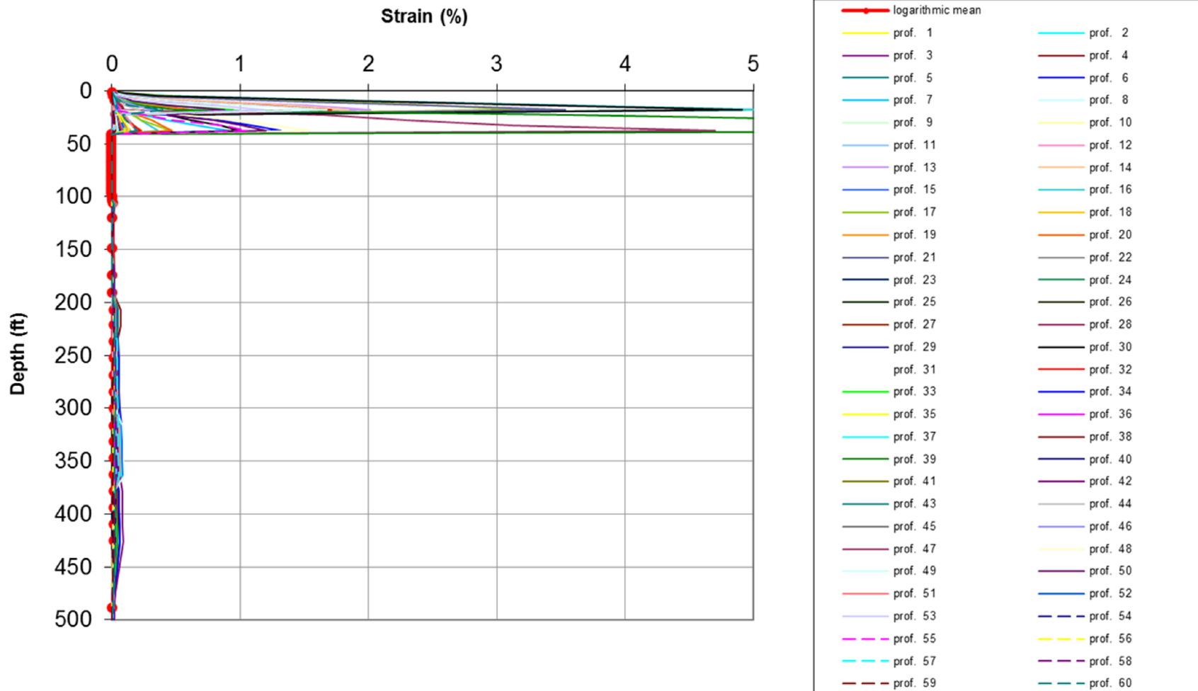
Figure 2.5.2-251 Maximum Shear Strain for the Upper 500 feet below Elevation 822 ft of FIRS3_COV50 Site Column (Full Site Column Corresponding to FIRS1_COV50 and FIRS2_COV50) for 10^{-6} Broad-Band Spectra
