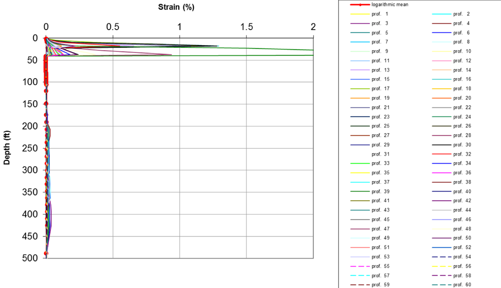
Figure 2.5.2-250 Maximum Shear Strain for the Upper 500 feet below Elevation 822 ft of FIRS3_COV50 Site Column (Full Site Column Corresponding to FIRS1_COV50 and FIRS2_COV50) for 10^{-5} Broad-Band Spectra
