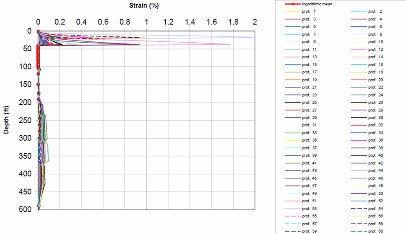
Figure 2.5.2-248 Maximum Shear Strain for the Upper 500 feet below Elevation 822 ft of FIRS3 Site Column (Full Site Column Corresponding to GMRS/FIRS1 and FIRS2) for 10^{-6} Broad-Band Spectra
