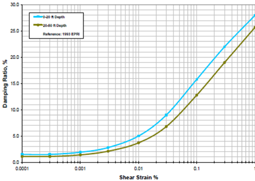
Figure 2.5.2-241 G/Gmax and Damping Ratio versus Strain for Granular Fill
