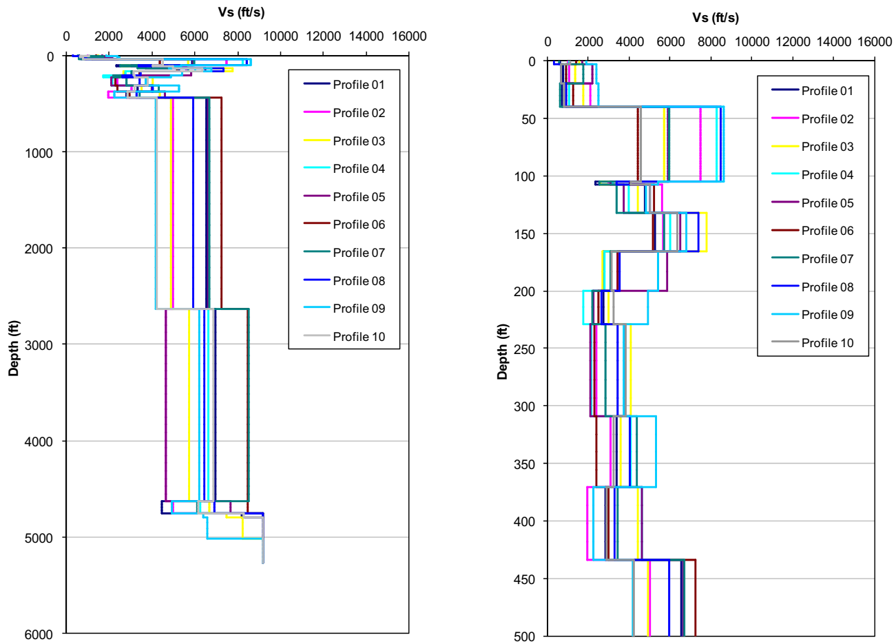
Figure 2.5.2-236 Velocity versus Depth for the First 10 Synthetic Profiles Generated for the FIRS3_COV50 Site Column
