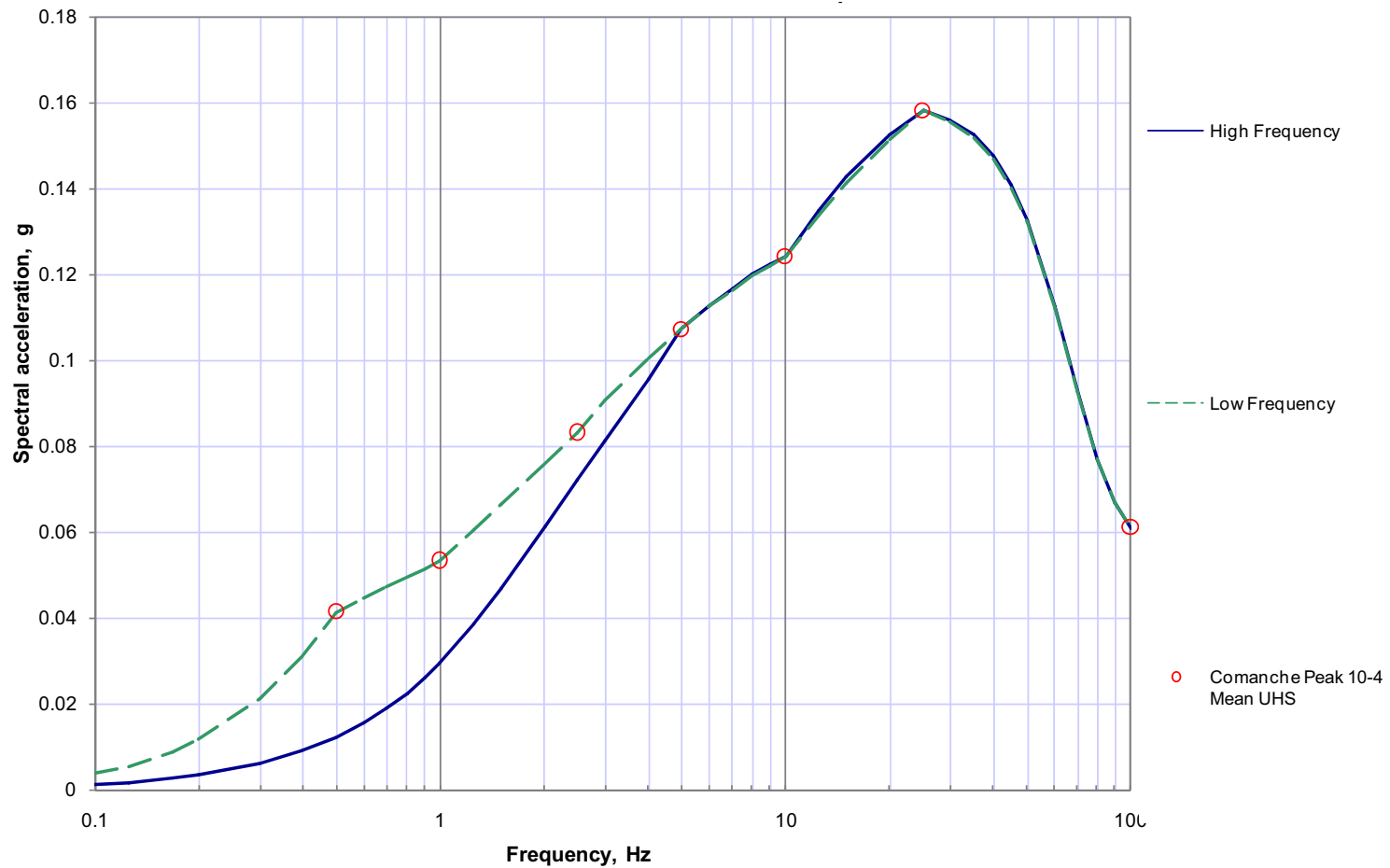
Figure 2.5.2-231 Smooth 10^{-4} Rock UHS for High and Low Frequencies
