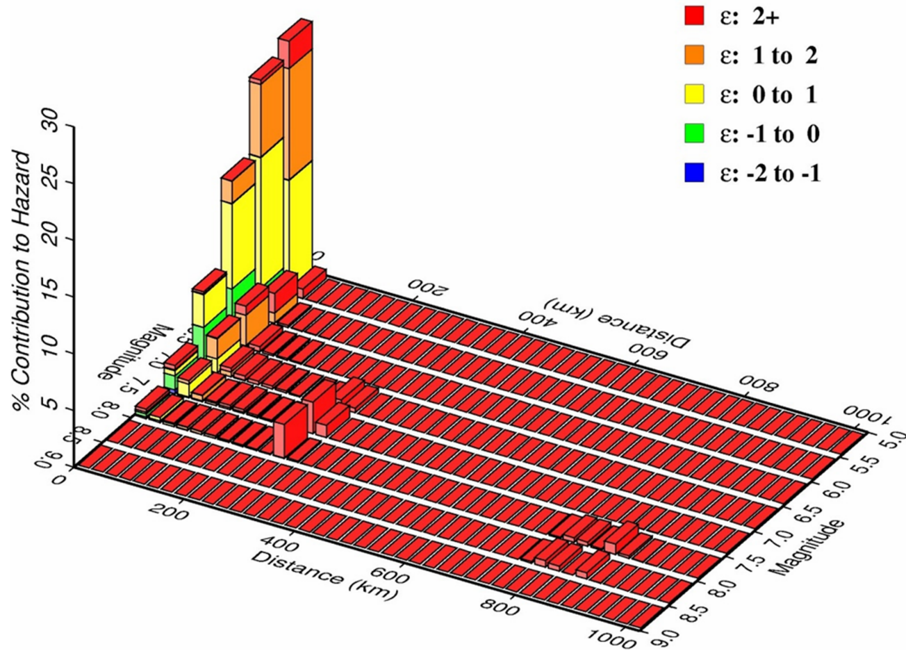
Figure 2.5.2-229 Deaggregation of 10^{-6} Rock Hazard for 5 and 10 Hz
