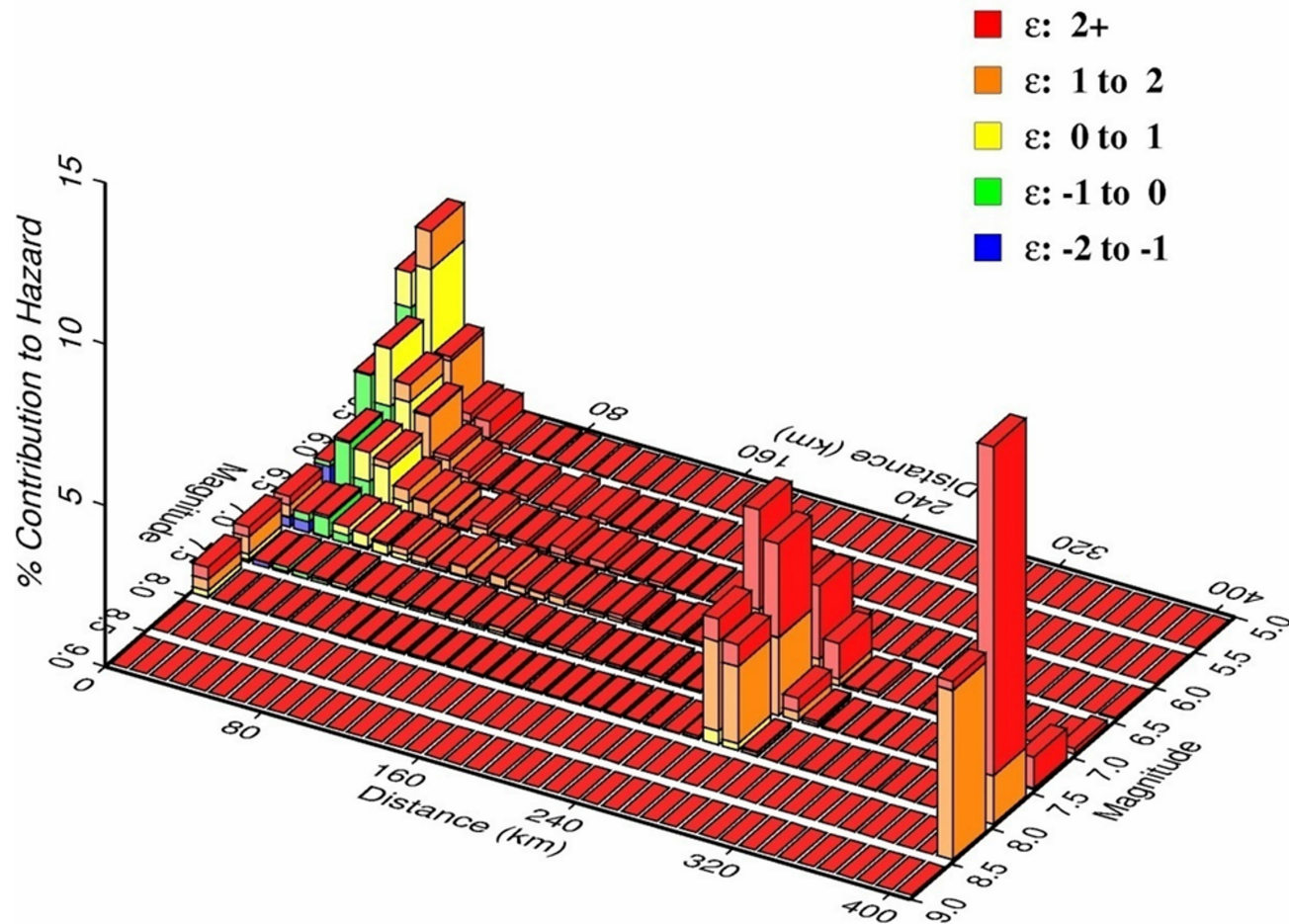
Figure 2.5.2-227 Deaggregation of 10^{-5} Rock Hazard for 5 and 10 Hz
