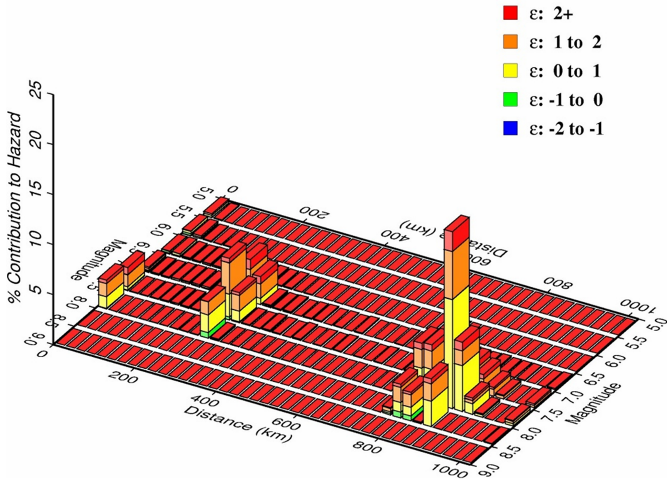
Figure 2.5.2-226 Deaggregation of 10^{-4} Rock Hazard for 1 and 2.5 Hz
