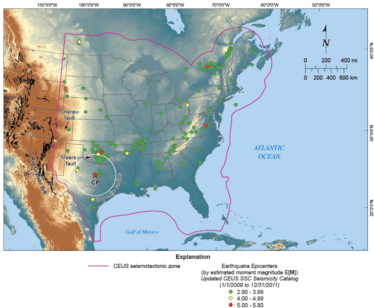
Figure 2.5.2-202 Updated CEUS SSC Seismicity Catalog plotted with the CEUS SSC Study Region
